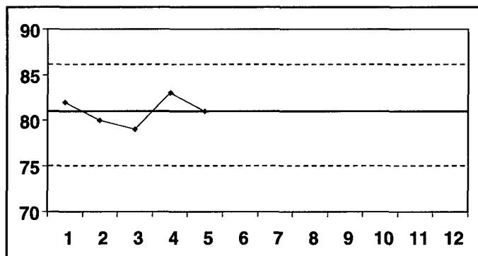
Figure 3. Control Chart
