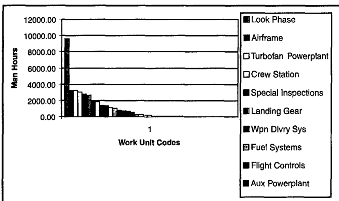
Figure 2. Pareto Chart
