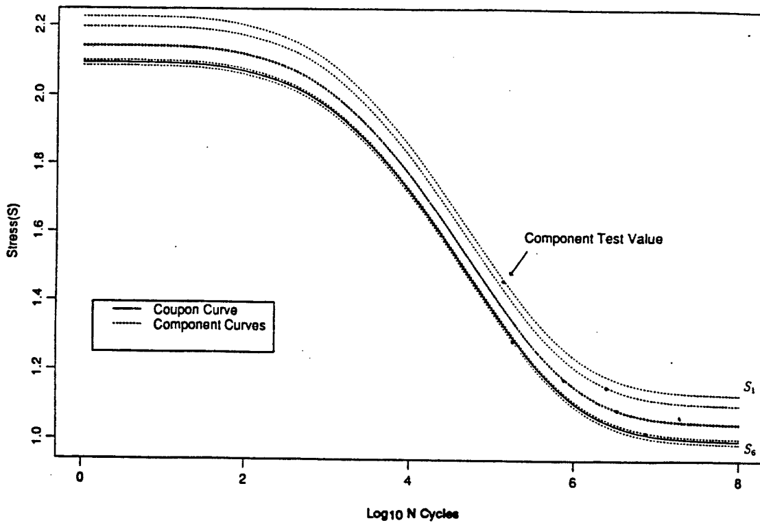
Figure 3. Extrapolation of component data.
