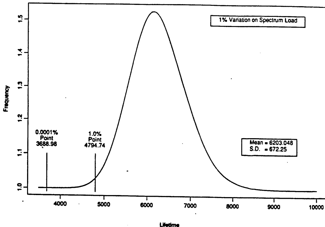
Figure 8. Component fatigue life probability density function and reliability.
