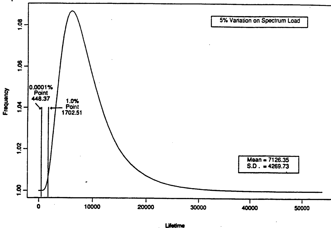
Figure 9. Component fatigue life probability density function and reliability.
