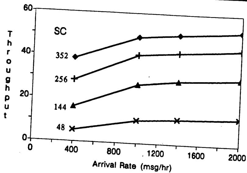
Figure 7. Normalized Throughput vs Arrival Rate Grouped by Message Length (Single Channel)
