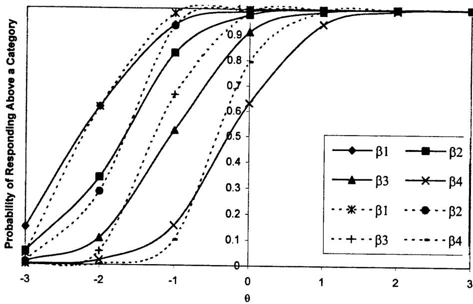
Figure 7 Boundary Response Functions for MEOCS 23 and MEOCS-R 29
