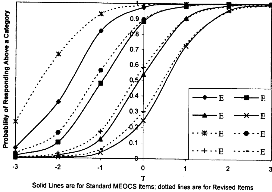
Figure 35 Category Response Functions for RAPS 100 and MEOCS 87
