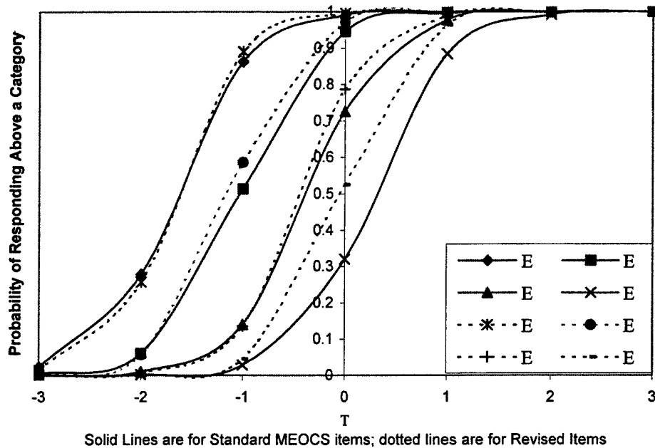
Figure 26 Boundary Response Functions for RAPS 75 and MEOCS 78
