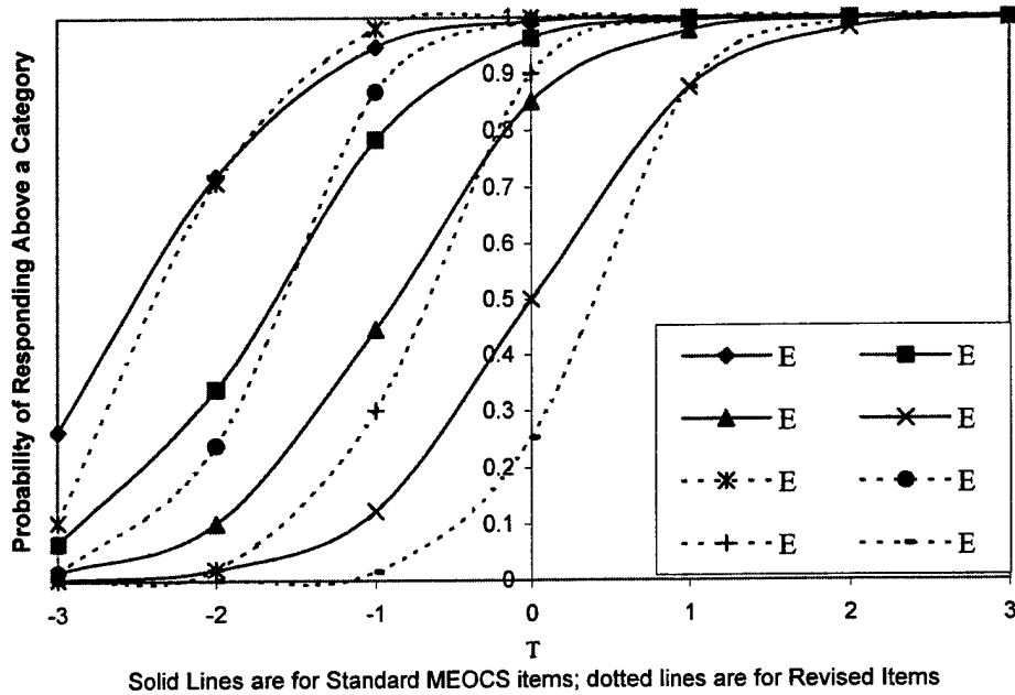
Figure 18 Boundary Response Functions for MEOCS 12 and MEOCS-R 95
