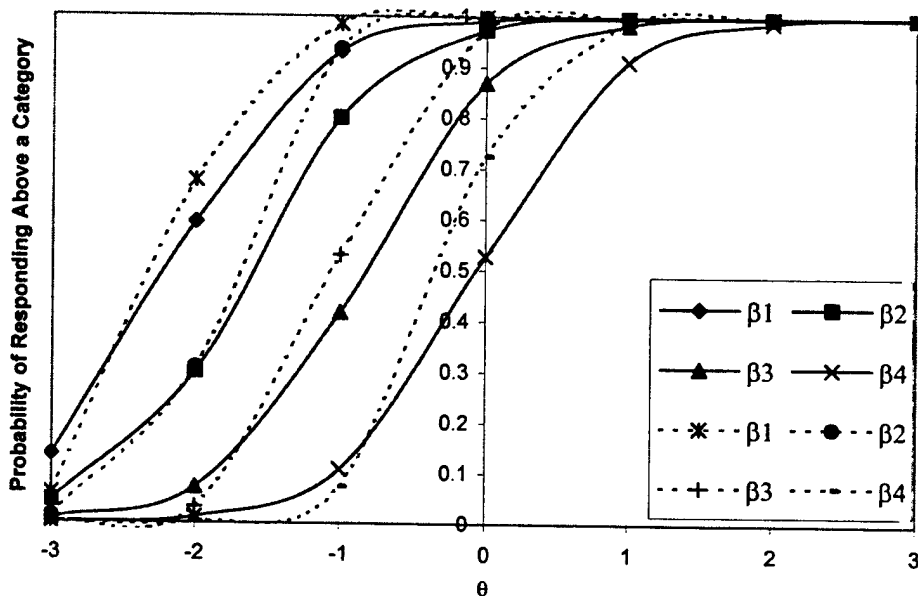
Figure 8 Boundary Response Functions for MEOCS 34 and MEOCS-R 30
