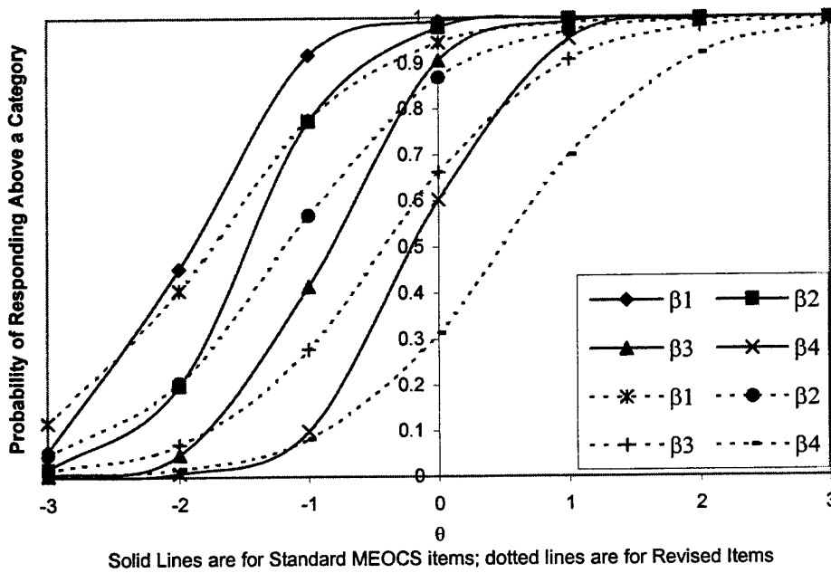
Figure 10 Boundary Response Functions for MEOCS 44 and MEOCS-R 32
