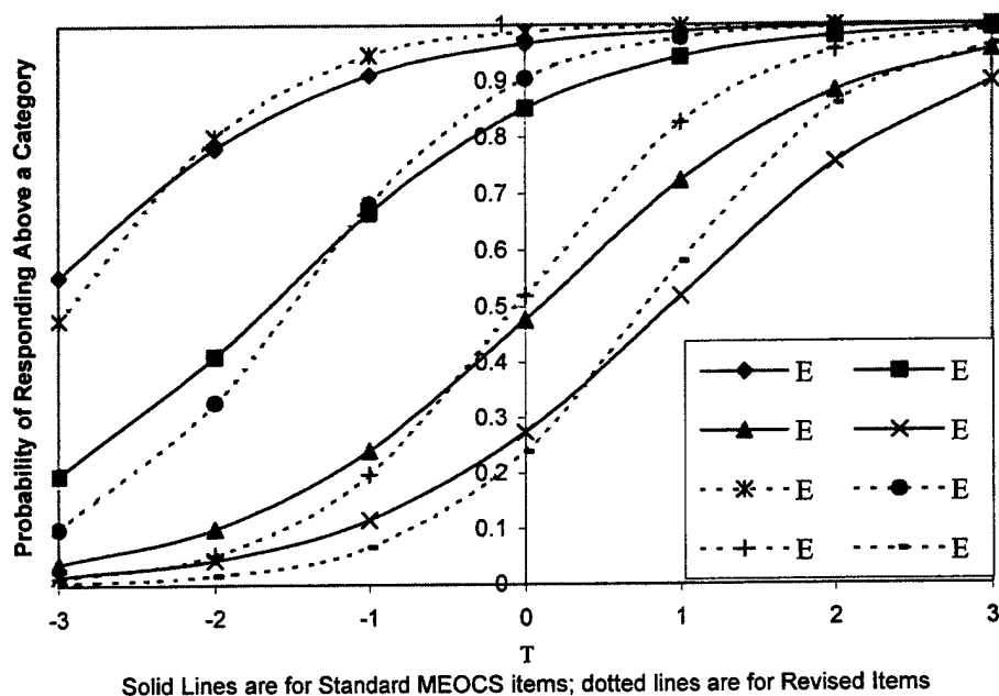
Figure 34 Category Response Functions for RAPS 99 and MEOCS-R 86
