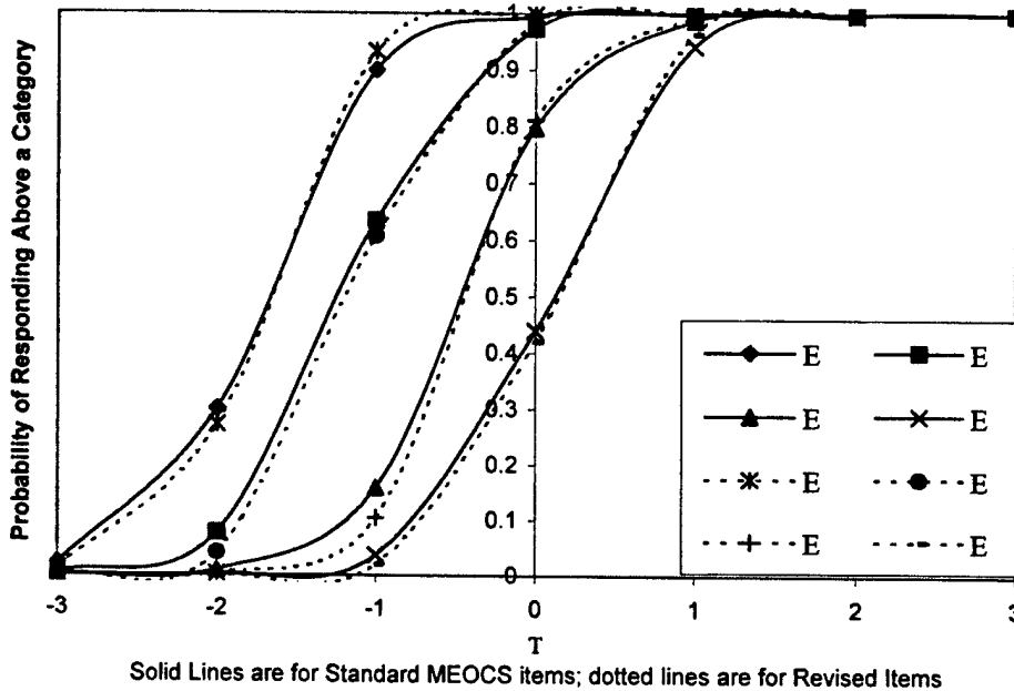
Figure 28 Category Response Functions for RAPS 77 and MEOCS-R 80
