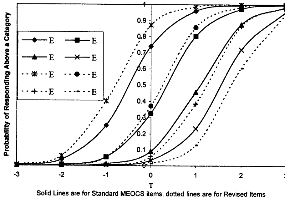
Figure 15 Boundary Response Functions for MEOCS 50 and MEOCS-R 43
