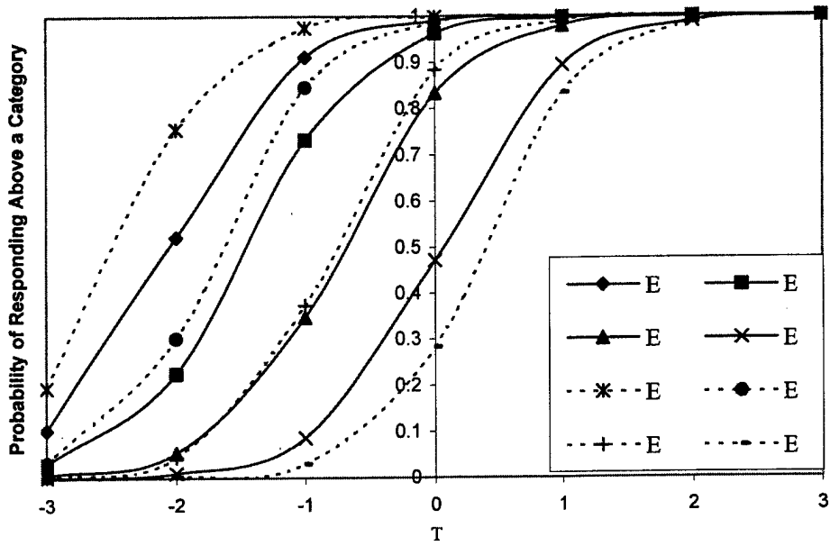
Figure 22 Boundary Response Functions for MEOCS 17 and MEOCS-R 99
