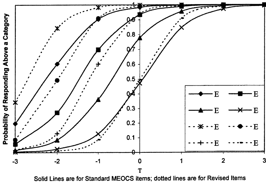
Figure 25 Boundary Response Functions for MEOCS 45 and MEOCS-R 102
