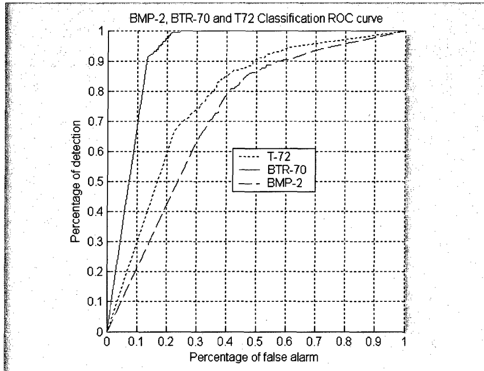
Figure 2. ROC curves of the MLP NN classifier, using the test set against the six confusers.
