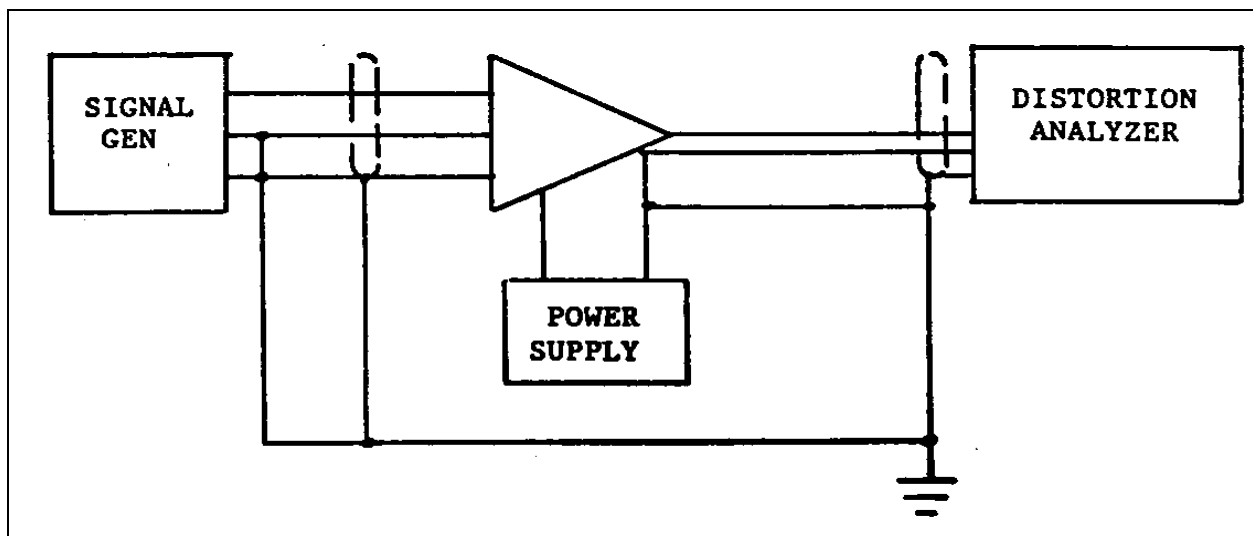
Figure 3-14 Block diagram for harmonic distortion test.
