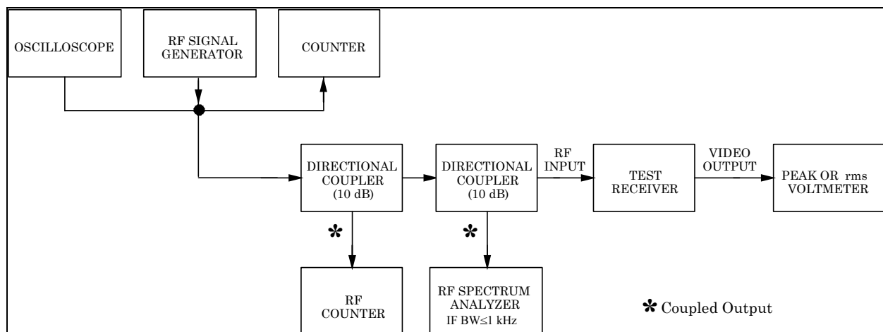
Figure 5-19. Incidental frequency modulation calibration test.
