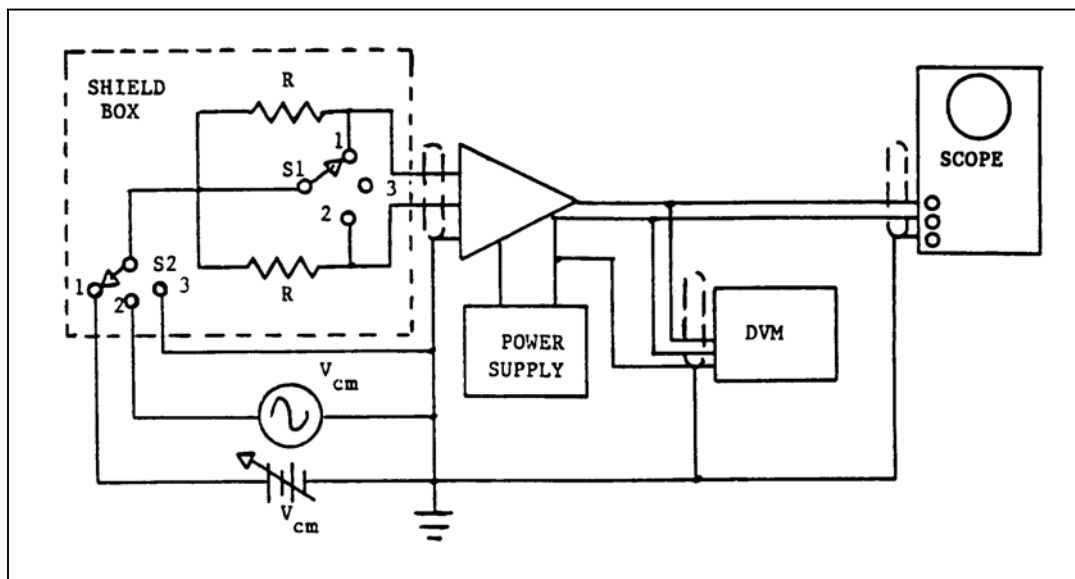
Figure 3-4. Block diagram for common mode rejection test.
