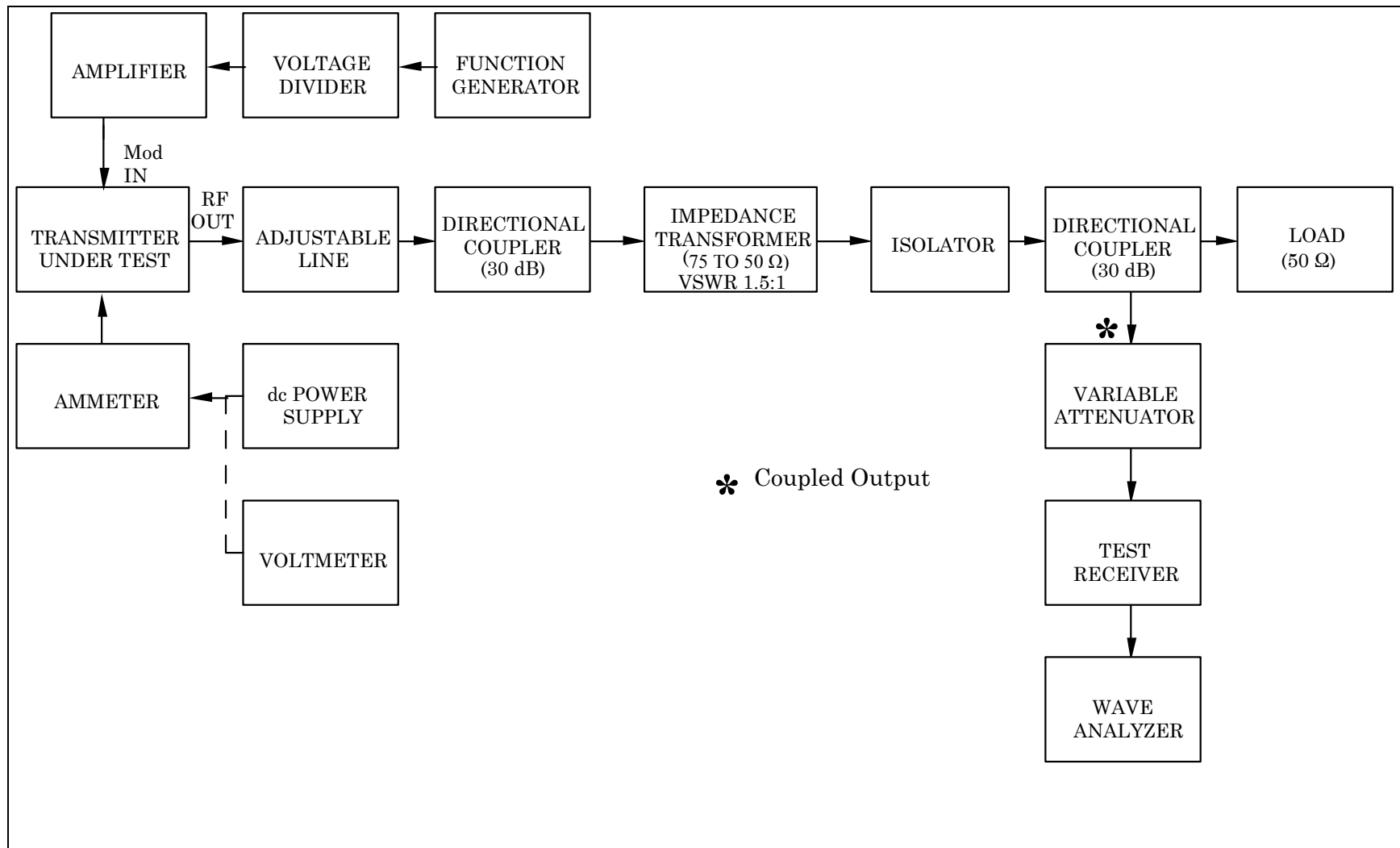
Figure 5-5. Modulation (ac) linearity test.
