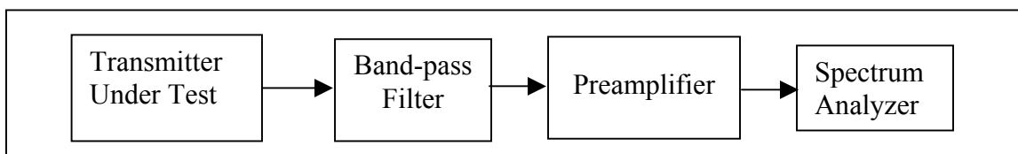
Figure 5-13b. Test setup for measuring low-level spurious signals at the transmitter output.
