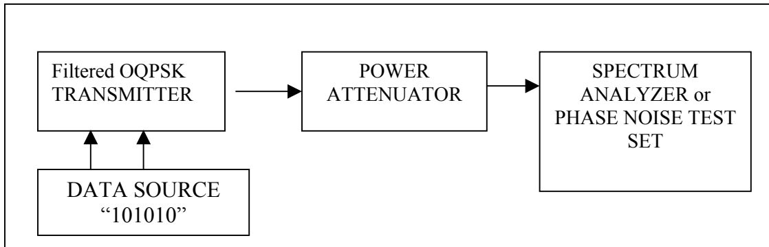
Figure 5-38. Test setup for filtered OQPSK transmitter phase noise test.
