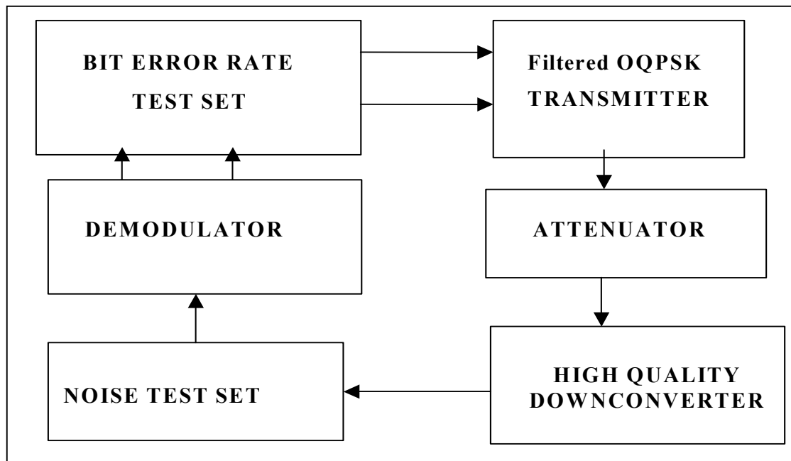
Figure 5-39. Test setup for filtered OQPSK transmitter bit error probability test.
