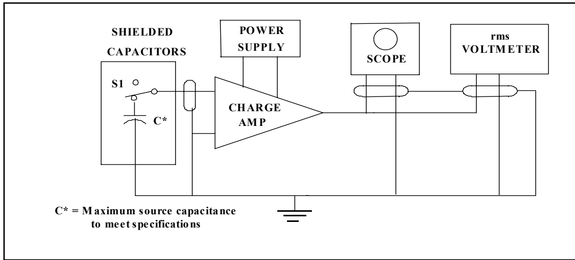
Figure 2-6. Block diagram for residual noise test.
