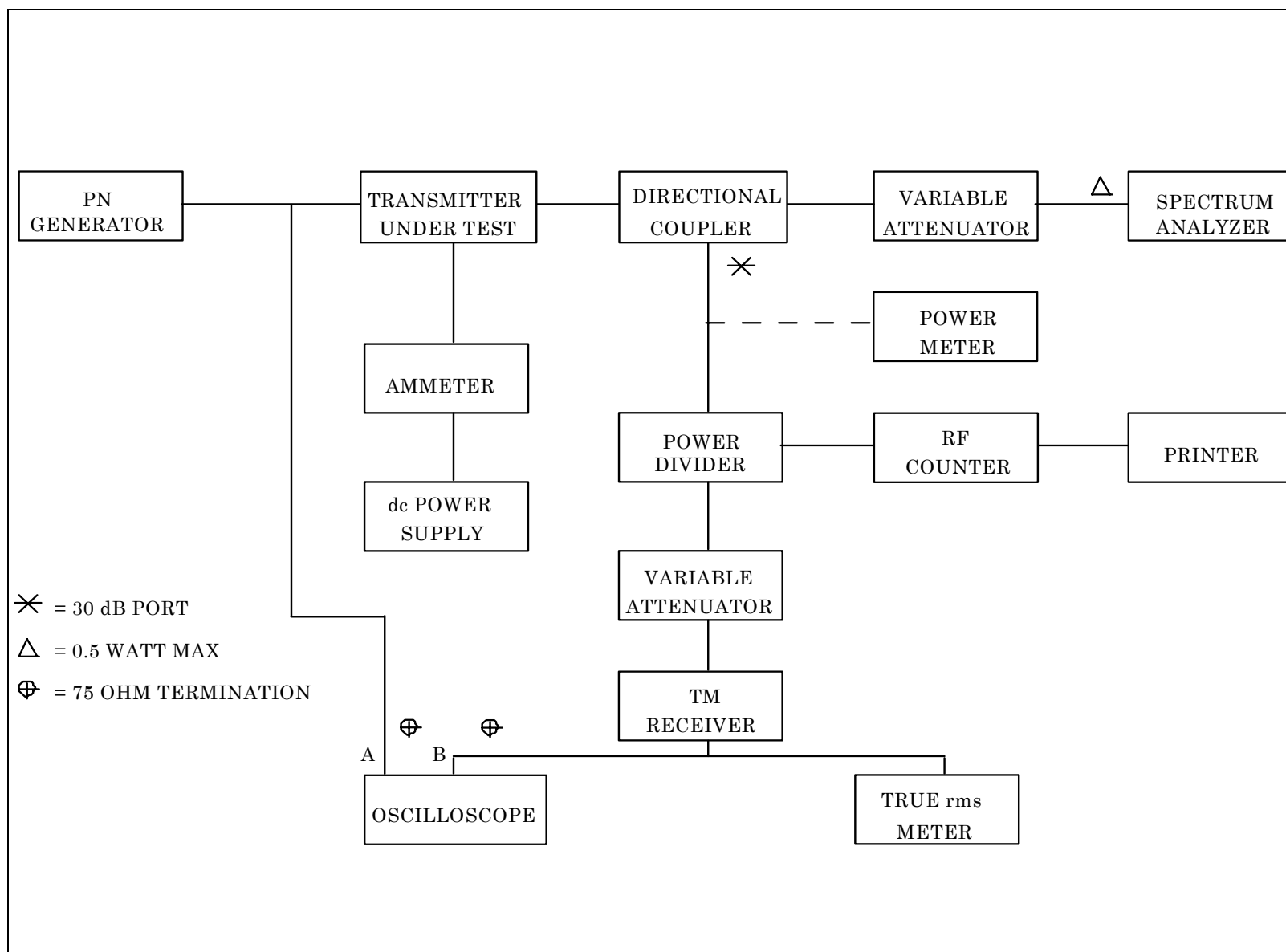
Figure 5-30. Eye pattern response test setup.
