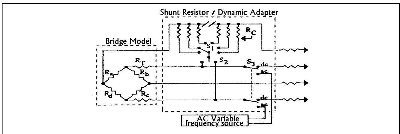
Figure 1-11. Shunt-resistor bridge.
