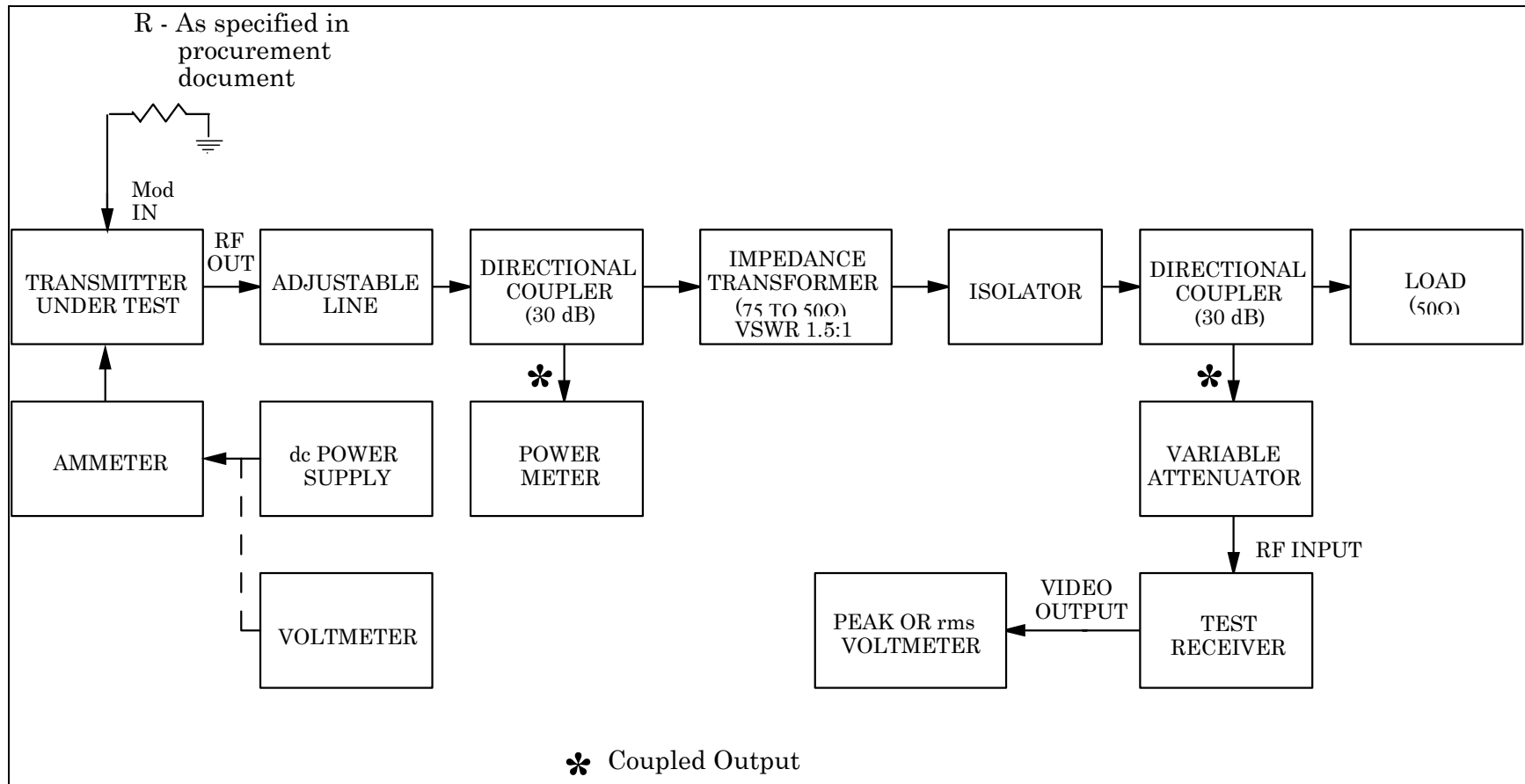
Figure 5-20. Incidental frequency modulation test.
