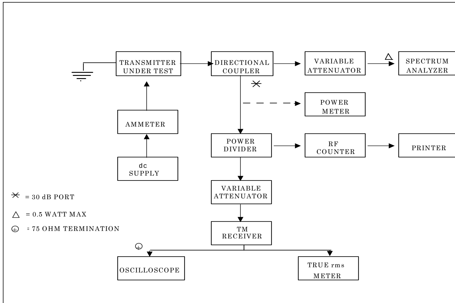
Figure 5-25. Center frequency and frequency stability test setup.
