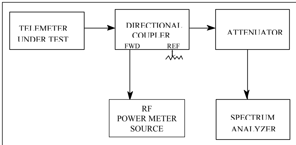
Figure 5-34. Laboratory setup.
