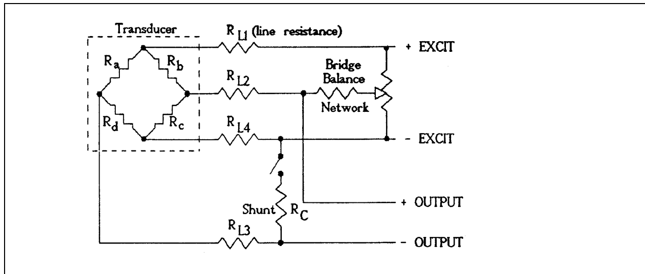
Figure 1-2. Four-wire system.
