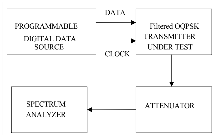
Figure 5-37. Test setup for filtered OQPSK modulator quality and spectral mask tests.
