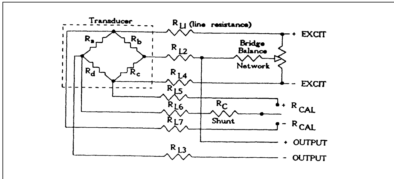
Figure 1-4. Bipolar shunting.
