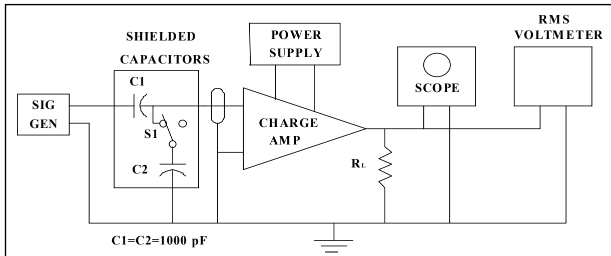
Figure 2-3. Block diagram for gain stability test.
