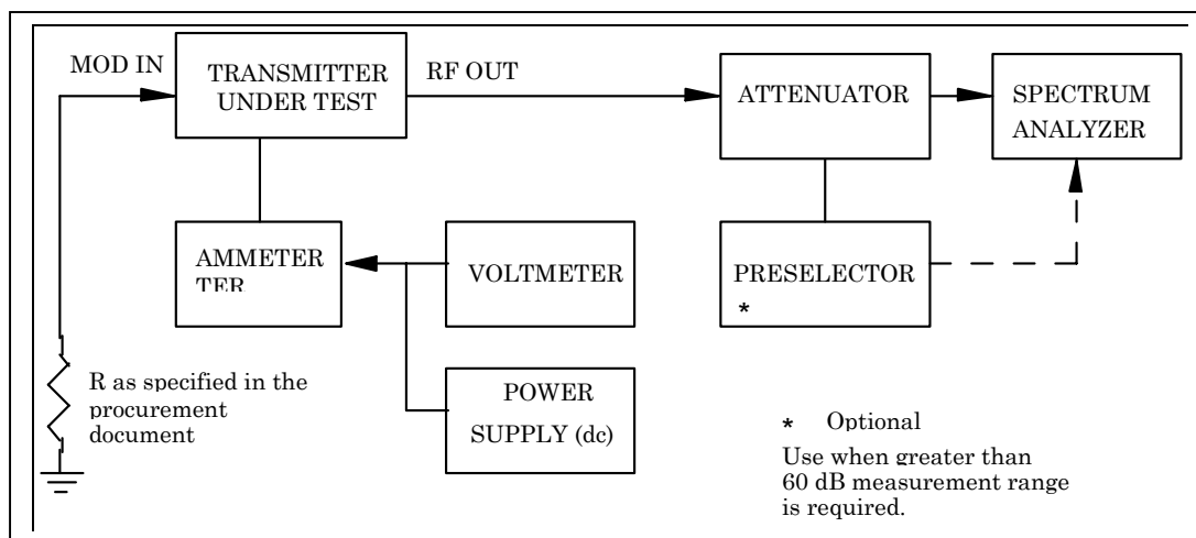
Figure 5-13a. Antenna conducted spurious and harmonic output test.
