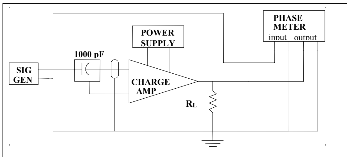
Figure 2-4. Block diagram for phase response test.
