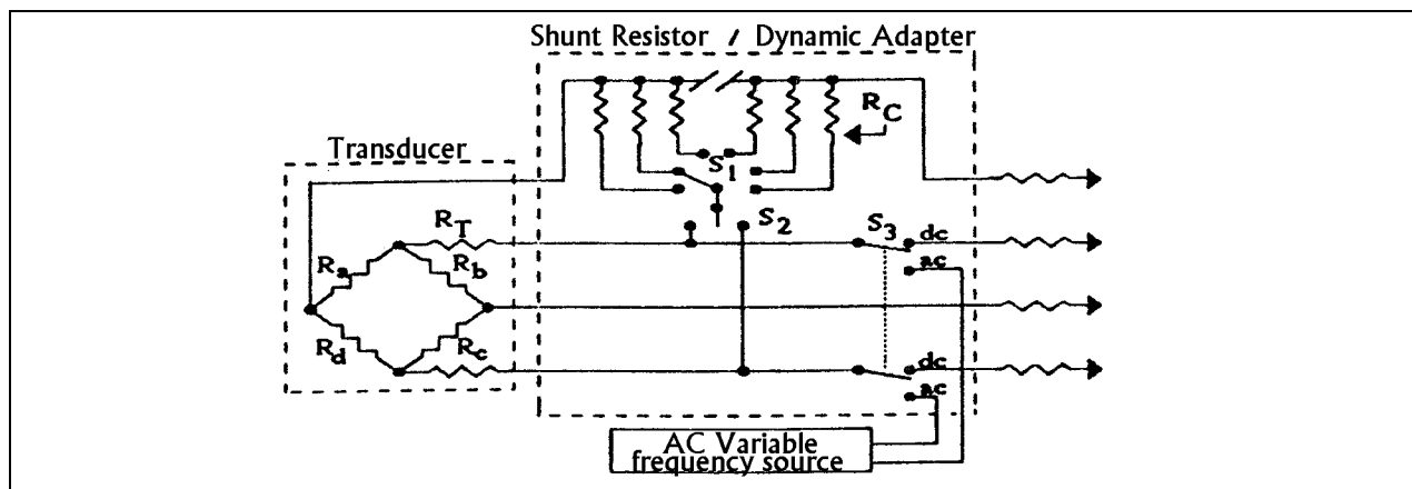
Figure 1-9. Shunt-resistor adapter.
