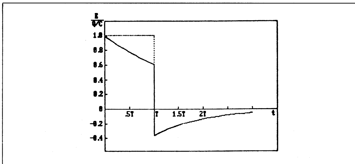
Figure 1-17. Effect of low-frequency response.
