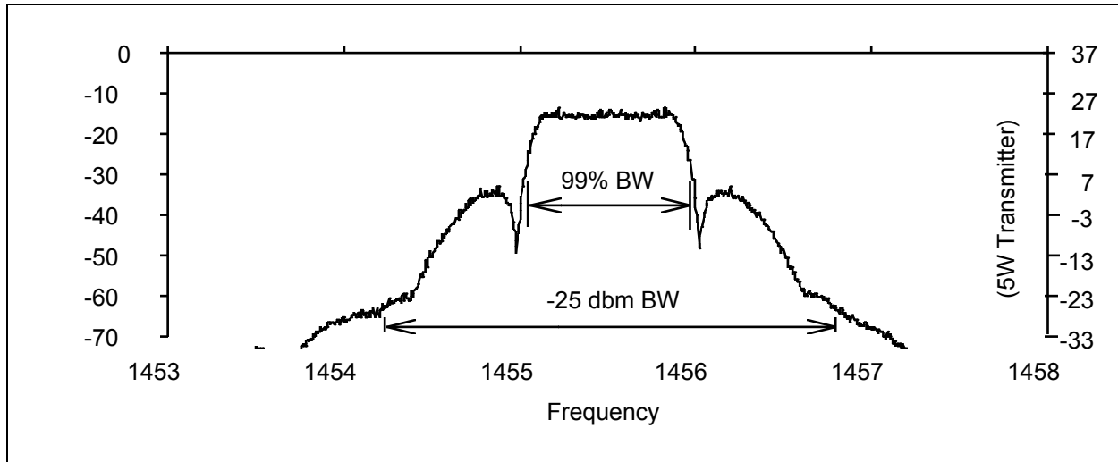
Figure 5-33. NRZ PCM/FM spectrum test.
