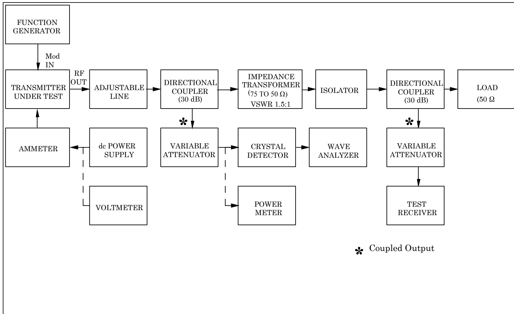
Figure 5-3. Incidental amplitude modulation test.
