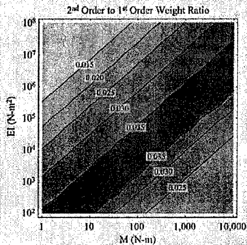
Figure 14: Ratio of 2 nd order to 1 st order truss weight per length optimization results ( E = 200 \text{ GPa (29 Msi)} , \rho = 1660 \text{ kg/m}^3 (0.06 \text{ lb/in}^3) ).
