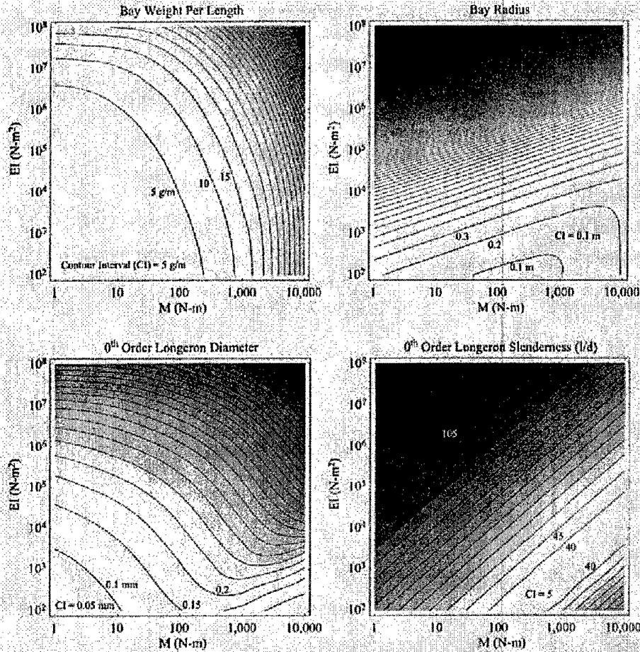
Figure 13: 2 nd order optimization results ( E = 200 \text{ GPa} (29 Msi), \rho = 1660 \text{ kg/m}^3 (0.06 lb/in 3 )).
