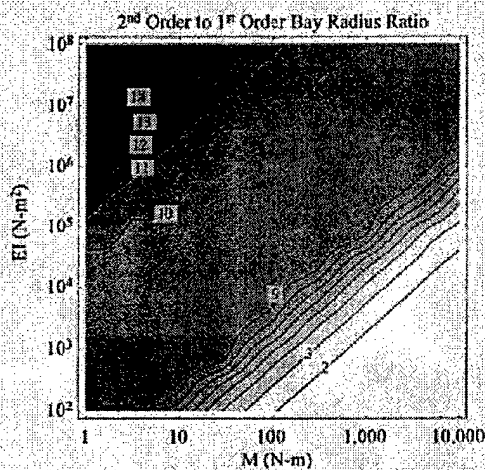
Figure 15: Ratio of 2 nd order to 1 st order truss radius optimization results ( E = 200 \text{ GPa (29 Msi)} , \rho = 1660 \text{ kg/m}^3 (0.06 \text{ lb/in}^3) ).
