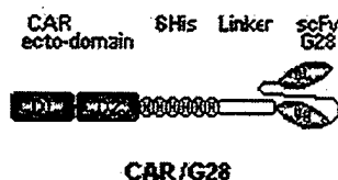
Figure 1 Structure of CAR/G28 fusion protein. The fusion protein consists of an extracellular portion of human CAR (domains D1 + D2) at the N-terminus connected to anti human CD40 scFv G28 via a short peptide linker (PSASASAPGS) preceded by a 6 histidine (6His) purification tag. CAR binds to Ad5 fiber knob, whereas G28 binds to CD40 present on DCs, thus facilitating Ad viral docking to DCs.
