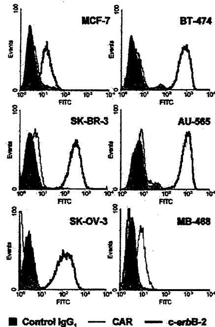
Fig. 5. Expression of CAR and c-erbB-2 in cancer cell lines. The breast cancer cell lines MCF-7, BT-474, SK-BR-3, AU-565, and MB-468 and ovarian cancer cell line SK-OV-3 were analyzed for CAR and c-erbB-2 expression (by indirect immunofluorescence assay using anti-CAR RmcB and anti- c-erbB-2 /HER-2/neu Ab-2 MAb, respectively). Positive staining for CAR (thin black line) and c-erbB-2 (bold black line) is seen relative to an isotype control IgG (spike filled in gray). Representative data from two independent experiments are shown.
