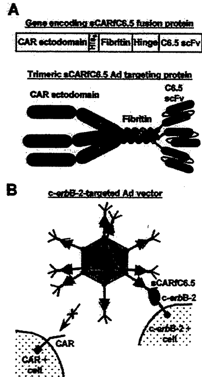
Fig. 1. A, design of sCARfC6.5 fusion protein. The recombinant fusion gene encoding the human CAR ectodomain, His 6 , polypeptide derived from phage T4 fibrin protein (Fibrin); proline-rich hinge region (Hinge), and C6.5 scFv to c-erbB-2 oncoprotein was constructed in a baculovirus expression vector. The sequence encoding fibrin polypeptide was introduced into the design to achieve sCARfC6.5 protein trimerization. Recombinant gene was expressed in baculovirus-infected insect cells and secreted sCARfC6.5 protein was purified. B, use of sCARfC6.5 protein for Ad targeting. Engineered bispecific sCARfC6.5 fusion protein serves as an adapter between Ad and cells expressing c-erbB-2 oncoprotein. Presence of three sCAR domains in the context of trimerized adapter molecule potentially provides high-affinity viral linkage because of the trivalent stoichiometry of CAR-knob binding. The use of trimeric sCARfC6.5 adapter protein might, therefore, allow efficient blocking of Ad infection of CAR-bearing cells. C6.5 scFv targeting moiety of virus-bound adapter protein mediates recognition of c-erbB-2 -positive cells, thereby providing novel target-specific Ad tropism.
