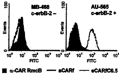
Fig. 4. Confirmation of sCARfC6.5 protein binding to cellular c-erbB-2 . Trimeric sCARfC6.5 and sCARf fusion proteins were incubated with either c-erbB-2 -positive AU-565 or c-erbB-2 -negative MB-468 cells. The sCARf fusion proteins bound to cells were probed with anti-CAR RmcB MAb and then detected with secondary Alexa 488-labeled goat antimouse antibodies. Binding of sCARfC6.5 protein (black line) to c-erbB-2 -positive AU-565 cells is seen because of the positive staining relative to sCARf control protein (gray line) or anti-CAR MAb alone (spike filled in black). Representative data from two independent experiments are shown.
