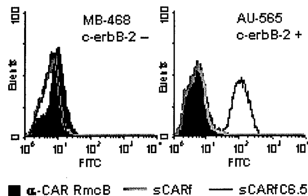
Fig. 8. Confirmation of sCARfC6.5 protein binding to cellular c-erbB-2 . Trimeric sCARfC6.5 and sCARf fusion proteins were incubated with either c-erbB-2 -positive AU-565 or c-erbB-2 -negative MB-468 cells. The sCAR fusion proteins bound to cells were probed with anti-CAR RmcB MAb and then detected with secondary Alexa 488-labeled goat antimouse antibodies. Binding of sCARfC6.5 protein ( black line ) to c-erbB-2 -positive AU-565 cells is seen because of the positive staining relative to sCARf control protein ( gray line ) or anti-CAR MAb alone ( spike filled in black ). Representative data from two independent experiments are shown.
