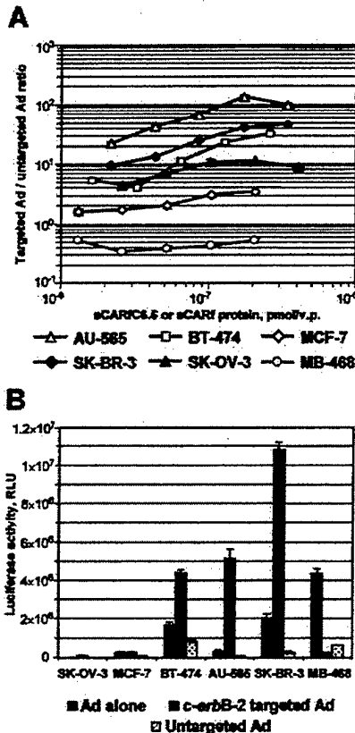
Fig. 6. sCARfC6.5 targeting adapter protein promotes Ad gene transfer to c-erbB-2 -positive cells. A , determination of optimal sCARfC6.5 adapter protein:Ad ratio. AdLucGFP vector expressing luciferase reporter gene was preincubated with either sCARfC6.5 targeting protein or sCARf control protein at varying concentrations to form c-erbB-2 -targeted or untargeted viral complexes, respectively. The monolayers of MCF-7, BT-474, SK-BR-3, AU-565, SK-OV-3, and MB-468 cells were infected with targeted or untargeted viral complexes at MOI of 100 v.p./cell. Cells were incubated for 46 h to allow expression of reporter gene, then were lysed, and the luciferase activity was analyzed. Results are presented as logarithm of ratio of luciferase activities detected in the cells infected with targeted Ad to luciferase activities detected in the cells infected with untargeted Ad complexes formed at the same concentration of each sCAR protein (Targeted Ad:Untargeted Ad). Each point represents the cumulative mean \pm SD of triplicate determinations. Error bars (some are smaller than the symbols). SDs. B , enhancement of Ad gene transfer by sCARfC6.5 targeting protein. AdLucGFP vector was preincubated with either PBS (Ad alone) or one of sCARfC6.5 ( c-erbB-2 -targeted Ad) or sCARf (untargeted Ad) proteins at the concentration providing maximal gene transfer augmentation as determined in A . The cell monolayers were infected with Ad alone (■), c-erbB-2 -targeted Ad (■), or untargeted Ad (□) viral complexes at MOI of 100 v.p./cell and analyzed for luciferase expression 46 h postinfection. Luciferase activities detected in cell lysates are shown as the cumulative mean of triplicate determinations of relative light units (RLU) \pm SD.
