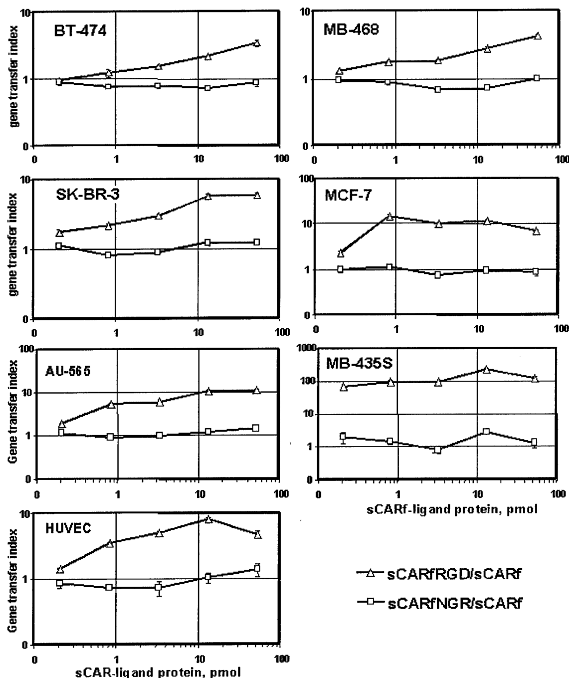
Fig. 11. Determination of optimal sCAR-ligand protein:Ad ratio. AdLucGFP vector expressing luciferase reporter gene was complexed with sCARfRGD or sCARfNGR targeting proteins or sCARf control protein at varying concentrations to form integrin-targeted, APN-targeted, or untargeted viral complexes, respectively. Monolayers of BT-474, MDA-MB-468, SK-BR-3, MCF-7, AU-565, MDA-MB-435S, and HUVEC cells were infected with targeted or untargeted viral complexes at a MOI of 100 vp/cell. Cells were incubated for 46 h to allow expression of reporter gene, then were lysed, and the luciferase activity was measured. Results are presented as gene transfer indexes that were calculated as the ratio of luciferase activities detected in the cells infected with targeted Ad to luciferase activities detected in the cells infected with untargeted Ad complexes formed at the same concentration of each sCAR protein ( Targeted Ad:Untargeted Ad ). Each point represents the cumulative mean \pm SD of triplicate determinations. Some error bars depicting SDs are smaller than the symbols. data clearly indicate that the sCARfC6.5-targeting adapter promoted Ad infection of CAR-deficient cells specifically via a c-erbB-2-dependent pathway.
