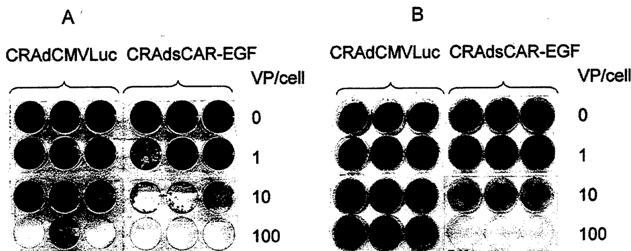
Fig. 3. Targeting oncolytic Ad to EGFR with sCAR-EGF results in an increased oncolytic effect. (A) SKOV3.ip1 or (B) A431 cells were infected with CRAdsCAR-EGF, a replication-competent sCAR-EGF-secreting dual-virus system. Oncolytic potency was compared with CRAdCMVLuc, which is isogenic in regard to replicativity but does not secrete a retargeting molecule. A similar effect on cells was observed with 1 VP/cell of CRAdsCAR-EGF as with 100 VP/cell of CRAdCMVLuc, suggesting increased oncolysis because of sCAR-EGF secretion-mediated EGFR targeting.
