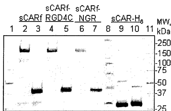
Fig. 2. Trimerization analysis of sCAR-fusion proteins by polyacrylamide gel electrophoresis. Samples of purified sCARf (lanes 2, 3), sCARf-RGD4C (lanes 4, 5), sCARf-NGR (lanes 6, 7), sCAR-H 6 (lanes 9, 10), and molecular mass markers (lanes 1, 8, 11) were separated on 4-15% gradient SDS gel. The samples in lanes 3, 5, 7, and 10 were boiled in Laemmli loading buffer to denature proteins to monomers, while lanes 2, 4, 6, and 9 contain unboiled proteins in their native conformation. Protein bands were visualized by GELCODE blue stain reagent (Pierce, Rockford, IL). The numbers on the right indicate molecular masses of marker proteins in kilodaltons (kDa).
