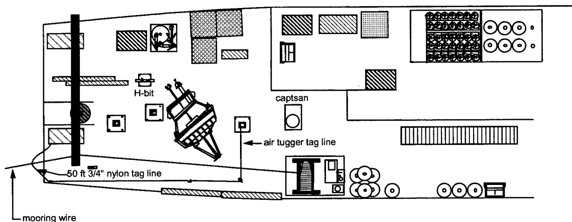
Figure 30. Haul-down fair lead utilized during NTAS-2 recovery. This allowed the mooring wire to be pulled close to the transom so that instruments could be removed.
