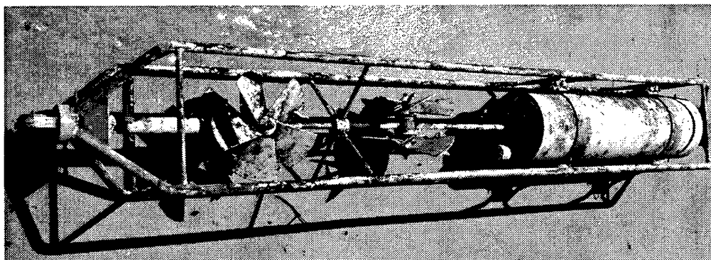
Figure 37. NTAS-2 VMCM after recovery.
