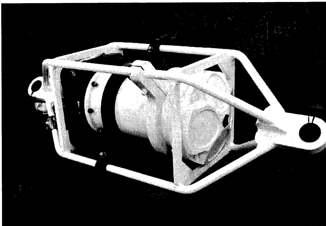
Figure 8. Photograph of the 300-kHz ADCP in welded aluminum load cage. Anti-fouling paint has been applied to the ADCP transducer head.
