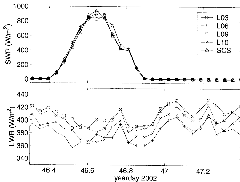
Figure 26. Shortwave (SWR, upper) and longwave (LWR, lower) radiation during the intercomparison period.
