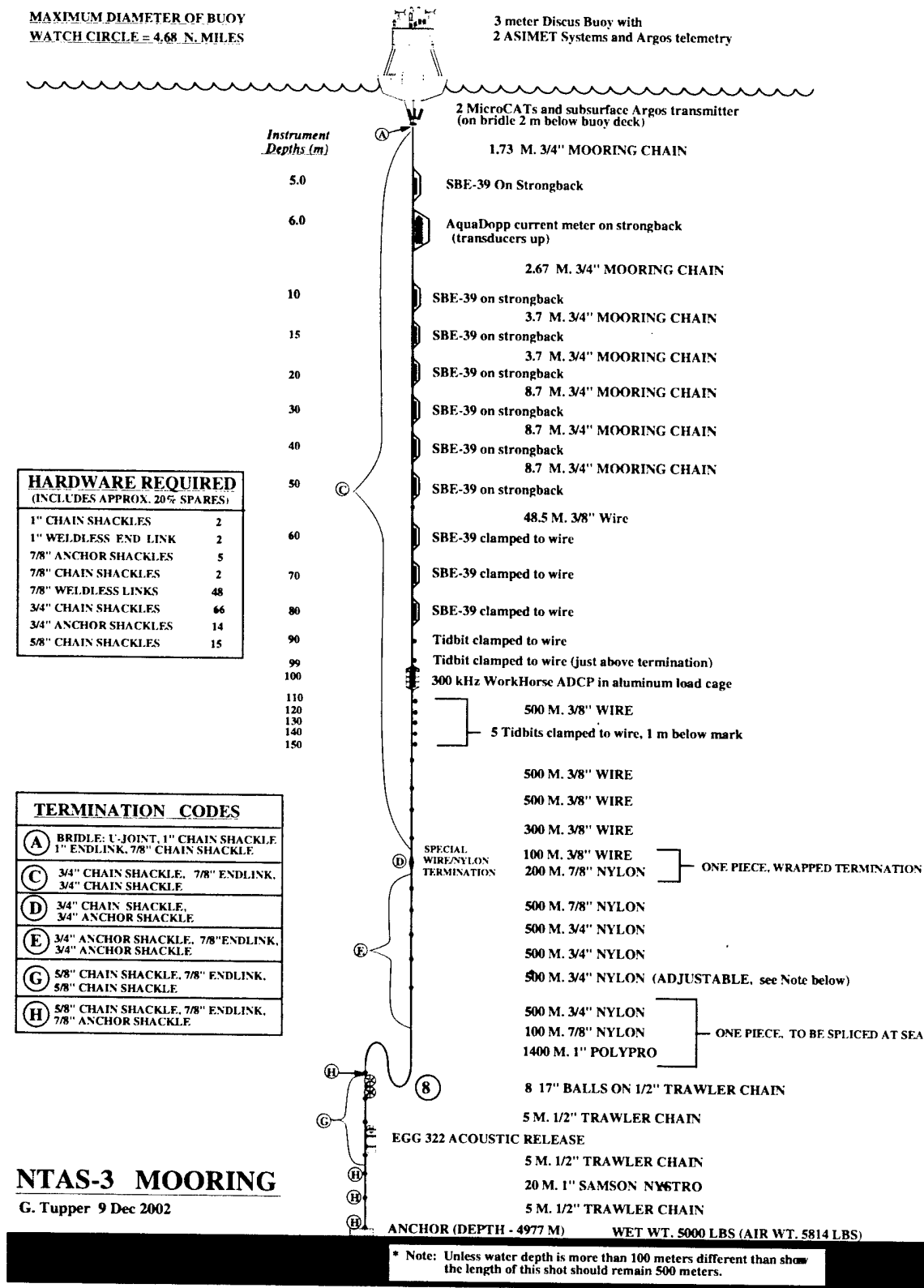
Figure 3. NTAS-3 mooring diagram.
