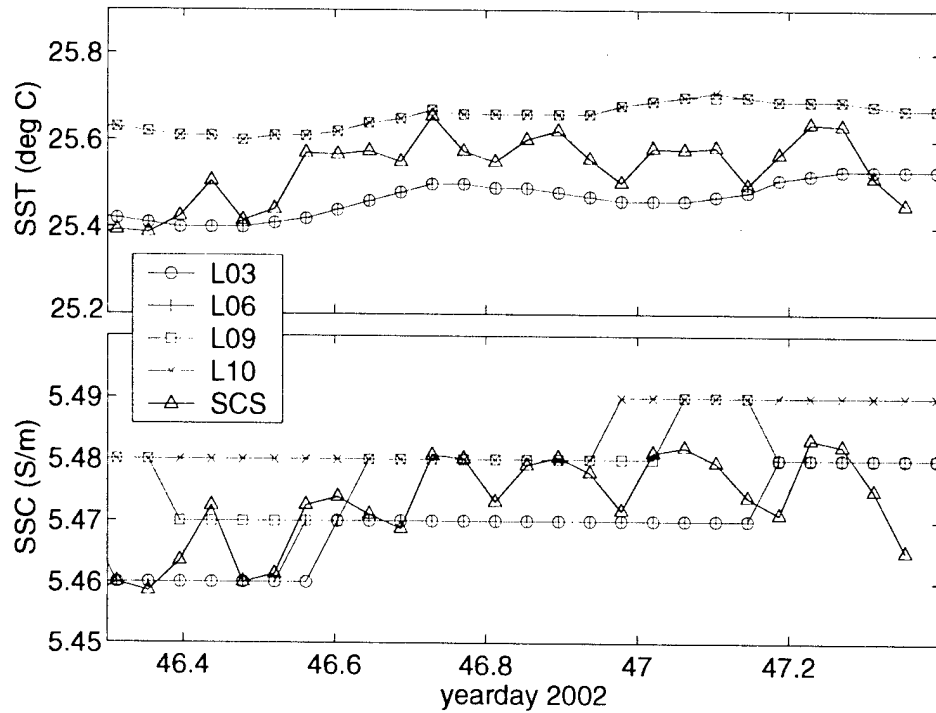
Figure 25. Sea surface temperature (SST, upper) and conductivity (SSC, lower) during the intercomparison period.
