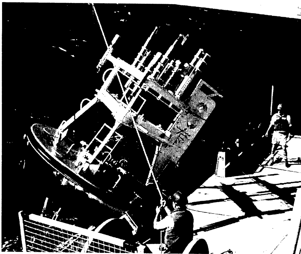
Figure 29. NTAS-2 buoy being recovered over the starboard rail.
