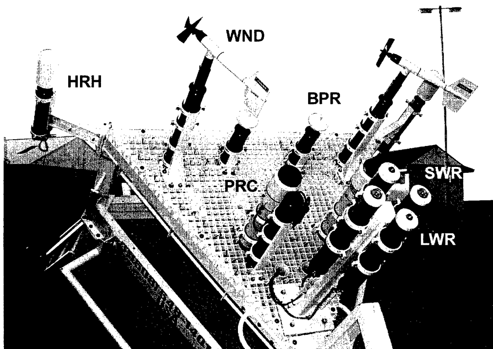
Figure 5. Photograph of the NTAS-3 tower top showing the location of ASIMET modules. The sea surface temperature and conductivity (STC) modules, located on the bridle legs, are not visible in this view.
