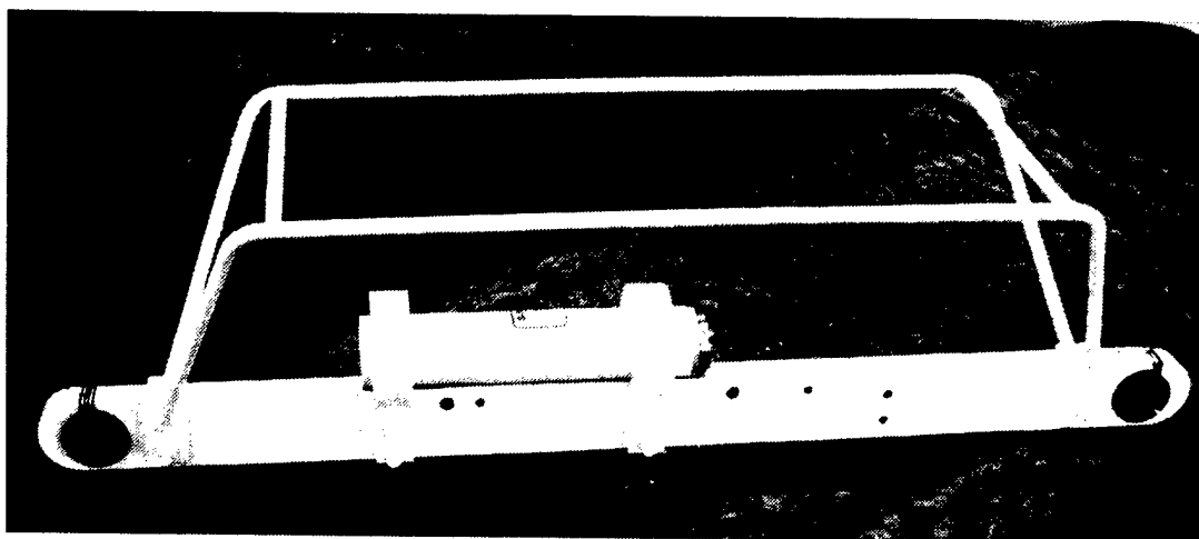
Figure 9. Photograph of SBE-39 attached to a titanium load bar. Anti-fouling paint has been applied to the load bar, cage and brackets.
