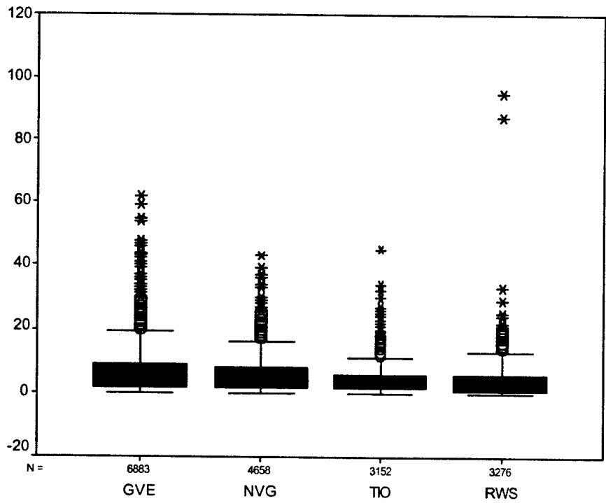
*Note: Extreme values are excluded to allow for better visual representation. Figure 25. Combined roll velocity box plots for subject #1.
