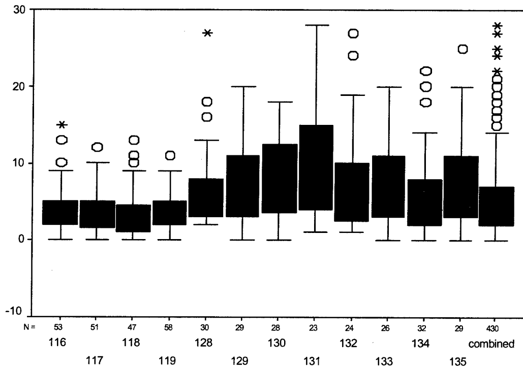
Figure G-1. Subject #1 GVE excursion box plots.
