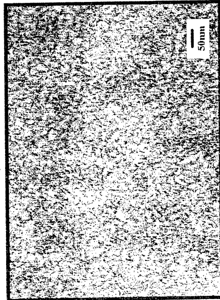
“Coarse” Cylinder Nanostructure (Diameter ~ 12nm) 50CpPOSS/PN
