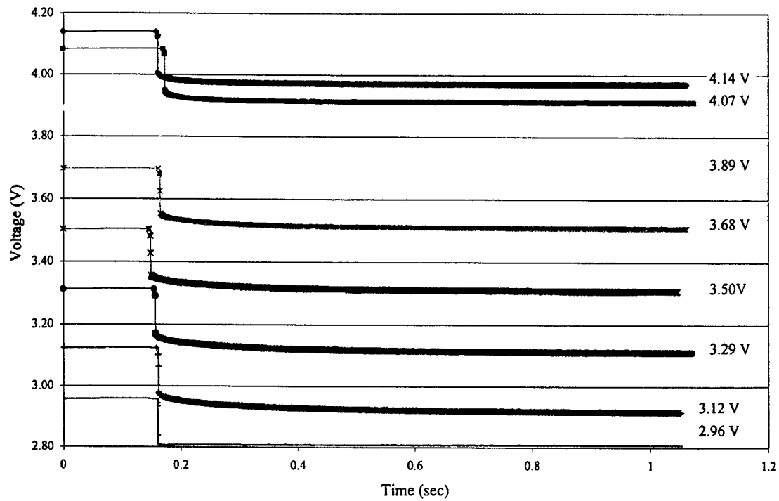
Figure 10. Transient voltage response of the space-grade cell to 2.8-A current; (top) before wake-up characterization cycle; (bottom) after wake-up characterization cycle.
