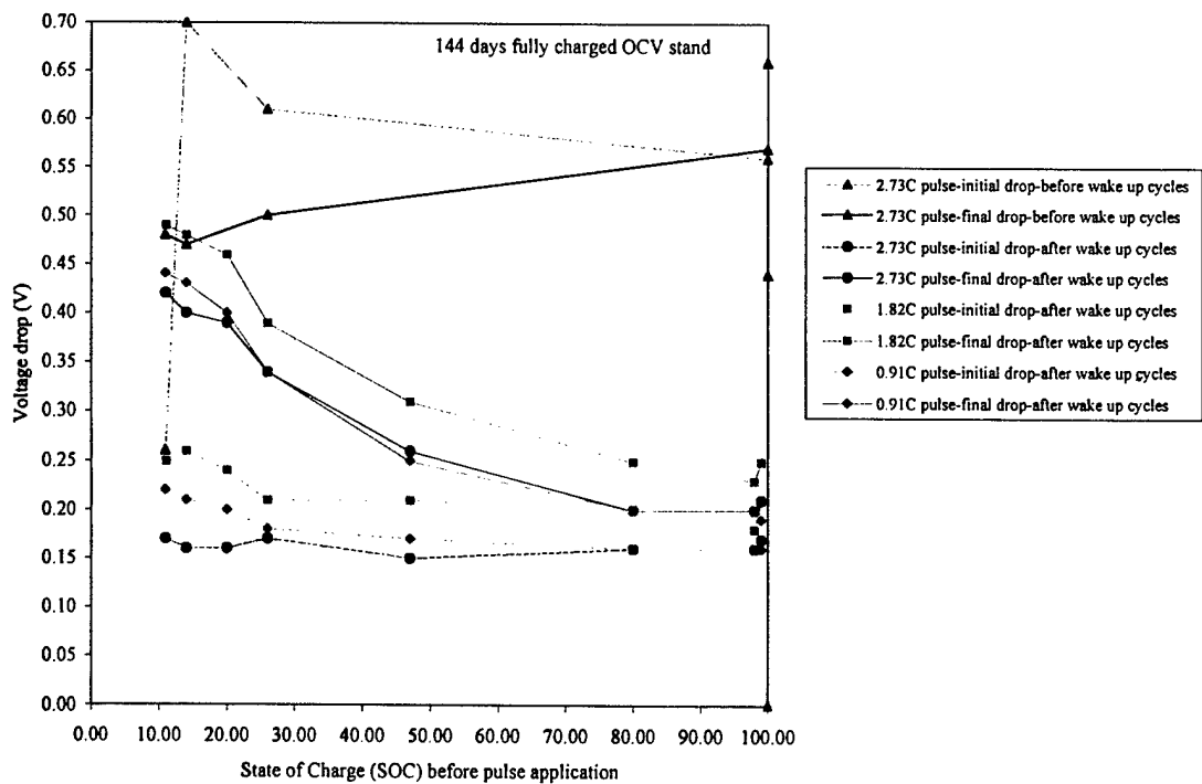
Figure 14. Plot presenting the instantaneous (0.01 s) and total (1 s) voltage drop after the application of pulse load in Canon (A&TB) CB-2 cell before and after the wake-up characterization cycles; (top) plot vs. voltage; (bottom) plot vs. SOC ( \pm 5\% ).
