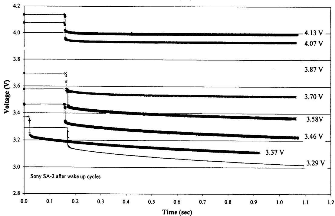
Figure 6. Transient voltage response of Sony SA-2 cell to 2.8-A current; (top) before wake up characterization cycle; (bottom) after wake up characterization cycle
