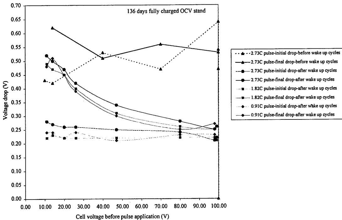
Figure 13. Plot presenting the instantaneous (0.01 s) and total (1 s) voltage drop after the application of pulse load in Canon (A&TB) CB-1 cell before and after the wake-up characterization cycles; (top) plot vs. voltage; (bottom) plot vs. SOC ( \pm 5\% ).
