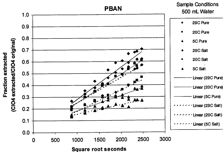
Figure 2.4. Plot of PBAN results. Linear-least-square fit is overlaid on the mass fraction (mass of perchlorate extracted divided by the mass of perchlorate originally in the specimen) vs. immersion time in 500 ml of deionized (pure) or salt water. Data from specimens run under the same conditions are combined in this plot.
