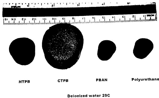
Figure 2.7. Wet solid propellant specimens after 3-month immersion at 29°C in deionized water. Left to right: HTPB, CTPB, PBAN, PU.
