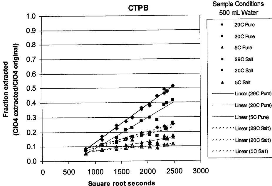
Figure 2.3. Plot of CTPB results. Linear-least-square fit is overlaid on the mass fraction (mass of perchlorate extracted divided by the mass of perchlorate originally in the specimen) vs. immersion time in 500 ml of deionized (pure) or salt water. Data from specimens run under the same conditions are combined in this plot.
