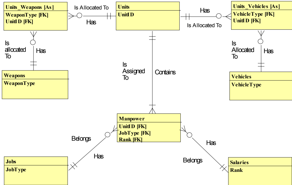
Figure 18. Entity Relationship Diagram of the Database Model – Primary Key Level
