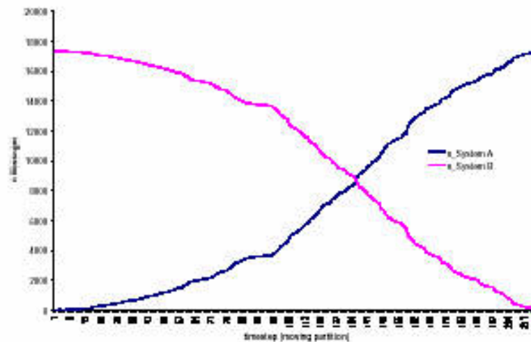
Figure III-12 Messages in two subsystems
