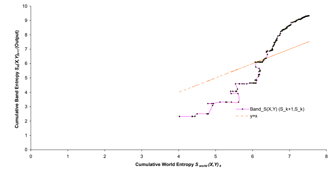
B_Band Entropy Map -- S_{\text{band}}(X,Y)_{k+1} , S_{\text{world}}(X,Y)_k Ada (month)
