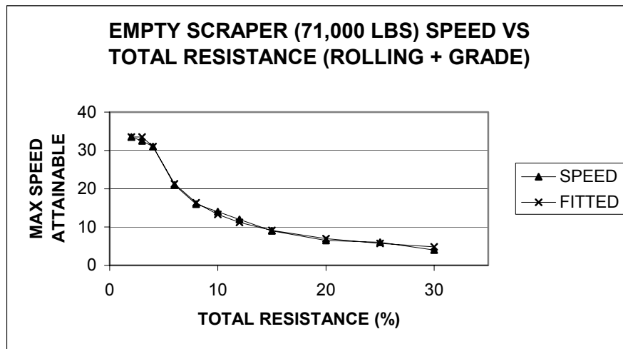
Figure 4-14: Empty Scraper Speed On Adverse Grades
