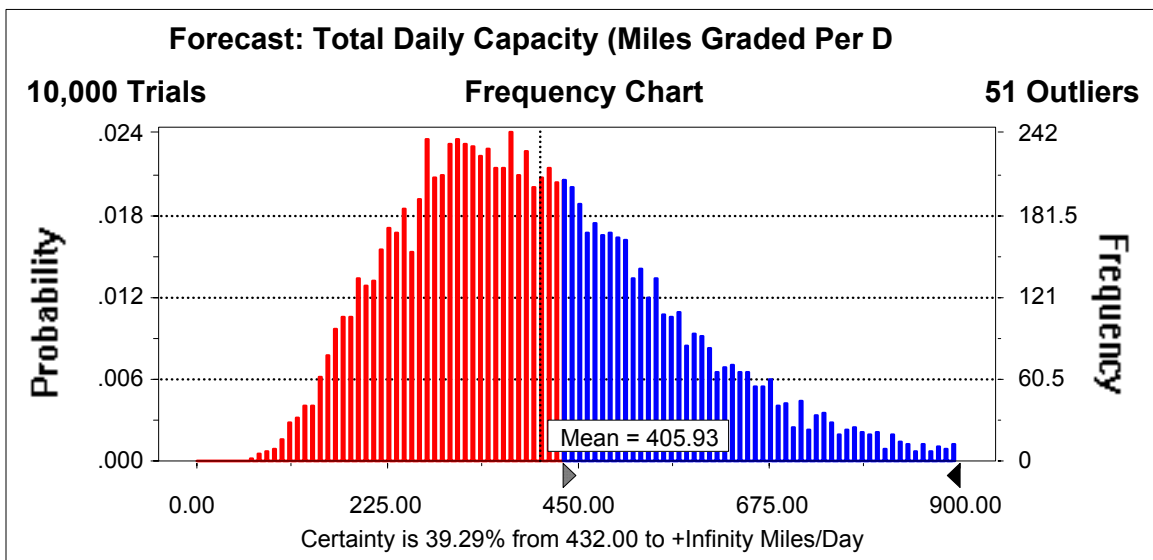
Figure 4-27: Grader Total Capacity (Surge)
