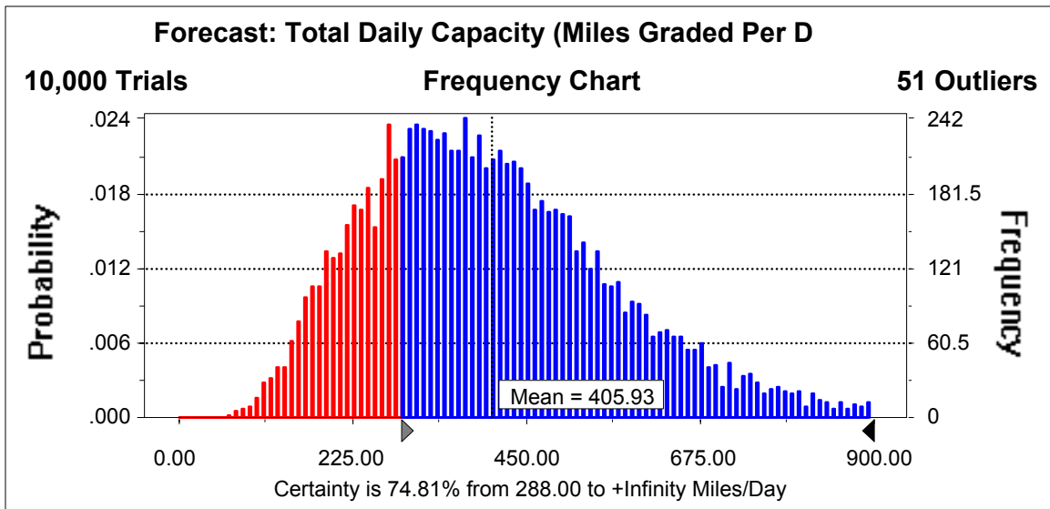
Figure 4-26: Grader Total Capacity (Peacetime)
