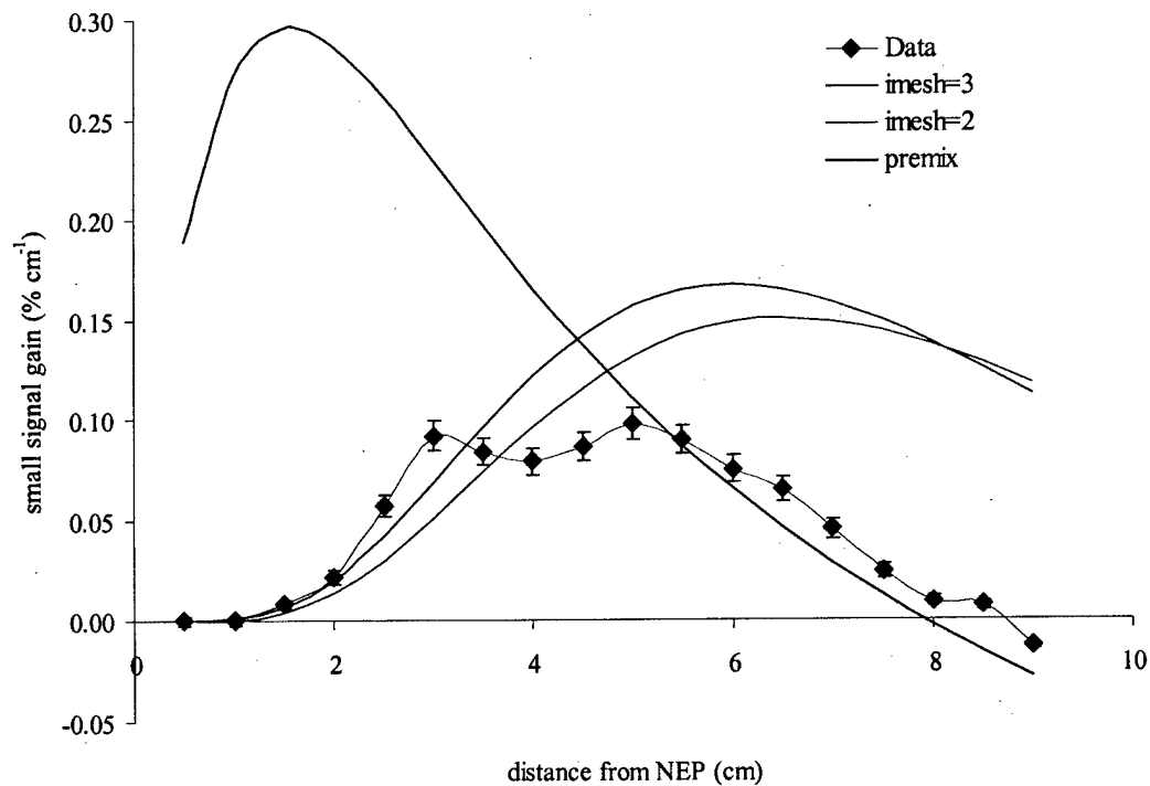
Figure 5.43 Measured and predicted centerline gain for the (F_2=2, H_2=10) flow conditions. Error bars represent 6% bias and 0.002 \% \text{ cm}^{-1} precision uncertainties.
