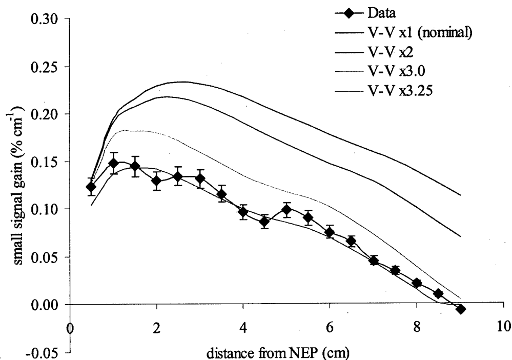
Figure 5.56 Measured and predicted peak gain for different HF V-V rate constants for the ( F_2=2 , H_2=10 ) flow conditions. Error bars represent 6% bias and 0.002 % \text{cm}^{-1} precision uncertainties.
