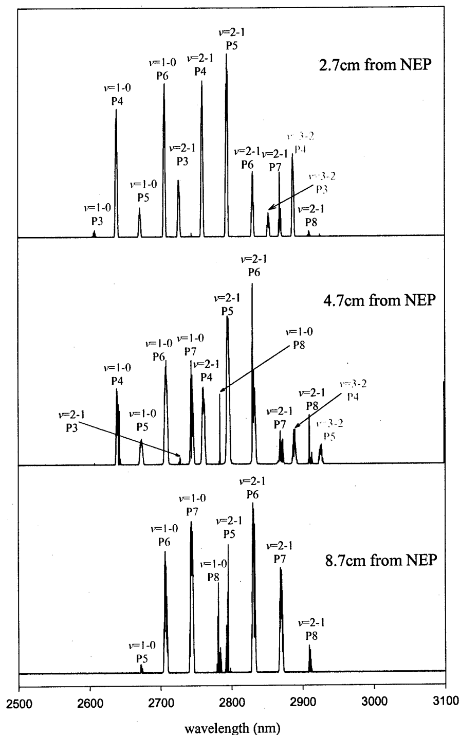
Figure 5.88 Fundamental multi-lasing spectra for the ( F_2=3 , H_2=10 ) flow conditions at optical axis positions of 2.7, 4.7 and 8.7 cm downstream of the NEP. All spectra were taken with Max R and 95% outcoupler reflectivity resonator. The intensity of each lasing line is scaled relative to the most intense line at each downstream location.
