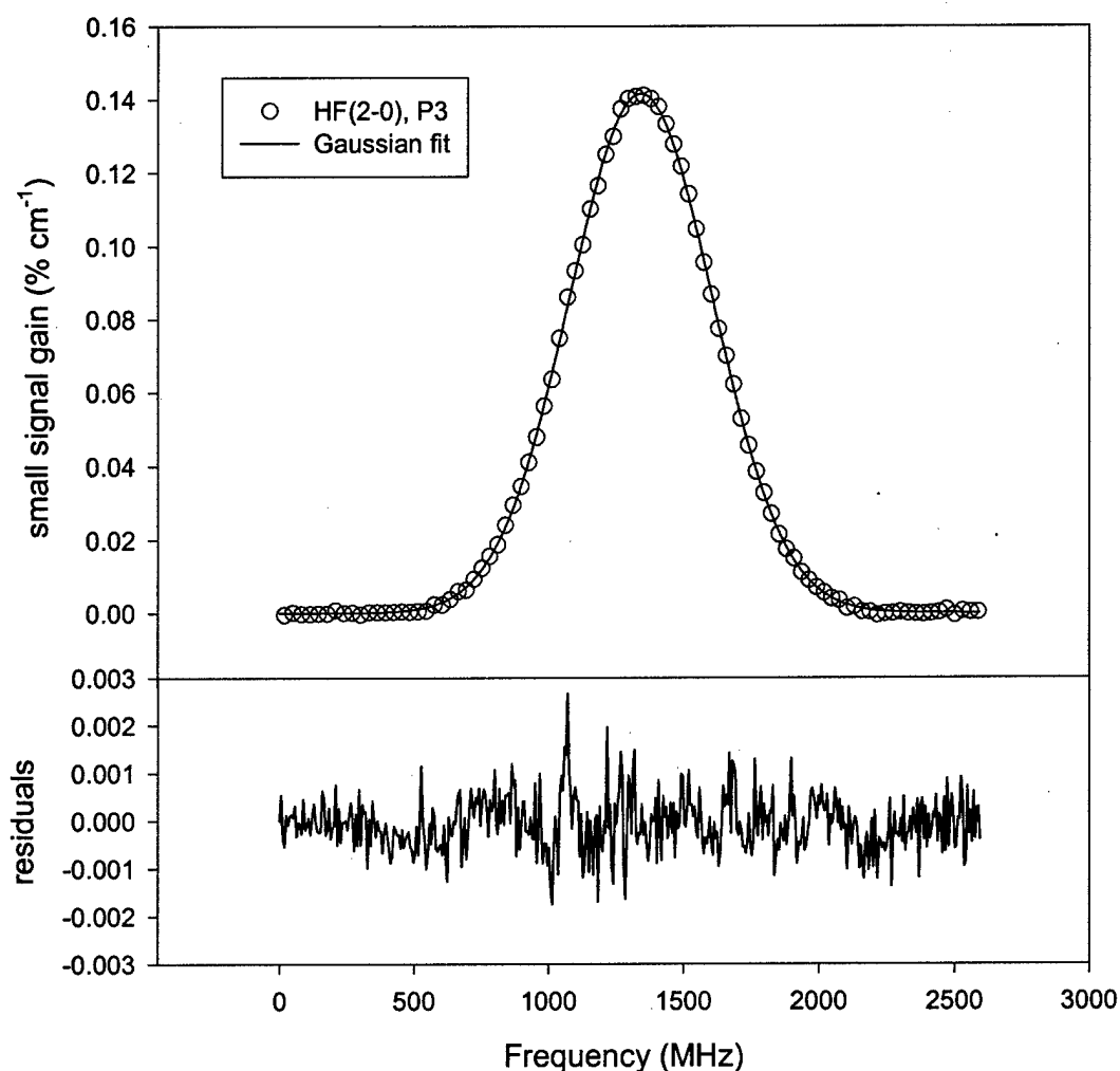
Figure 3.10 Transition lineshape of the P(3) ro-vibrational line of the first HF overtone ( \nu'=2 , J'=2 , \nu=0 , J=3 ). The experimental conditions for the upper panel are the ( F_2=2 , H_2=10 ) flow conditions, x = 2.5 cm downstream of the NEP, and z = 0.15 cm above the centerline. For purposes of clarity, only every 5 th data point is shown. The residual plot shown in the lower panel represents the residual difference between all the data and the curve fit and demonstrates that the Gaussian line function adequately fits the entire lineshape.
