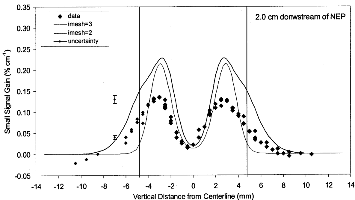
Figure 5.40 Measured and predicted gain profiles 2.0 cm downstream of the NEP for the ( F_2=2 , H_2=10 ) flow conditions. Solid black vertical lines indicate the vertical height of the nozzle at the NEP. Error bars represent 6% bias and 0.002\% \text{ cm}^{-1} precision uncertainties.
