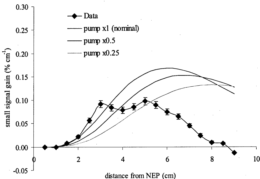
Figure 5.53 Measured and predicted centerline gain at different cold pumping reaction rate constants for the ( F_2=2 , H_2=10 ) flow conditions. Error bars represent 6% bias and 0.002\% \text{ cm}^{-1} precision uncertainties.
