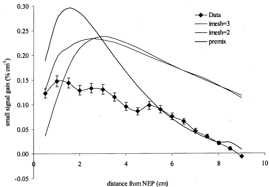
Figure 5.42 Measured and predicted peak gain for the (F_2=2, H_2=10) flow conditions. Error bars represent 6% bias and 0.002 \% \text{ cm}^{-1} precision uncertainties.
