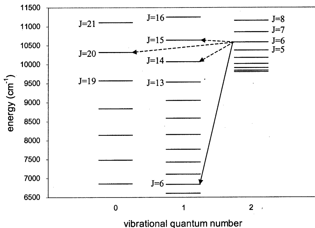
Figure 2.6 \text{HF}(v)+\text{HF}\rightarrow\text{HF}(v-1)+\text{HF} energy transfer routes. Solid arrow represents “true” V-T energy relaxation process. Broken arrows represent near-resonant V-R energy transfer.
