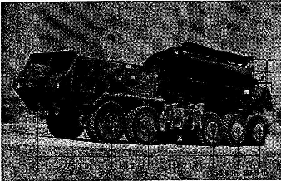
Figure 9. PLS Military-Vehicle axle spacing
