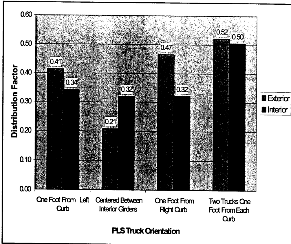
Figure 28. Distribution Factors for PLS Military-Vehicle (Patrick County Bridge)
