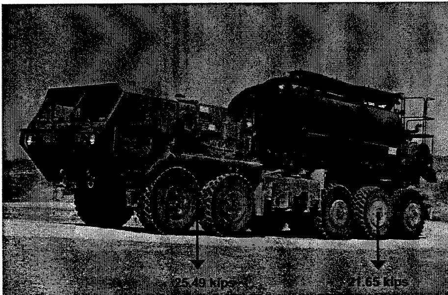
Figure 10. PLS Military-Vehicle axle weights
