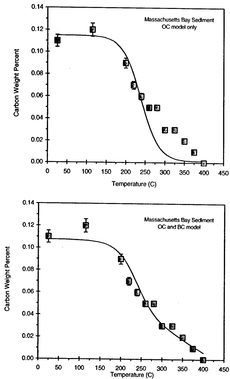
Figure 15: Thermogram (representing the measured carbon weight percentage after a 24-hour combustion at a given temperature (°C)) for Massachusetts Bay sediment (filled squares) along with (a) the best-fit OC model and (b) the best-fit, Eq. 2-based OC/BC model. Thermogram data are listed in Appendix A3.7 and Boltzmann parameters (Eq. 1) are listed in Table 3.
