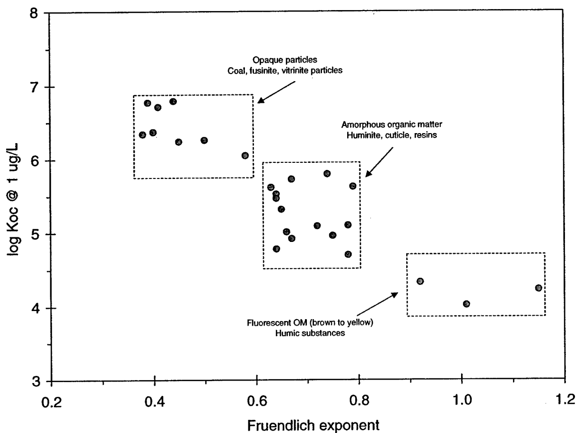
Figure 4: Reported phenanthrene sorption data (filled circles) by Kleineidam et al. (1999) Environ. Sci. Technol. plotted here as single-point log K_{oc} values calculated at 1 \mu\text{g/L} versus the Freundlich exponent. Based on the reported maturity of the organic matter, the data is subdivided with three dotted boxes to distinguish three organic carbon facies.
