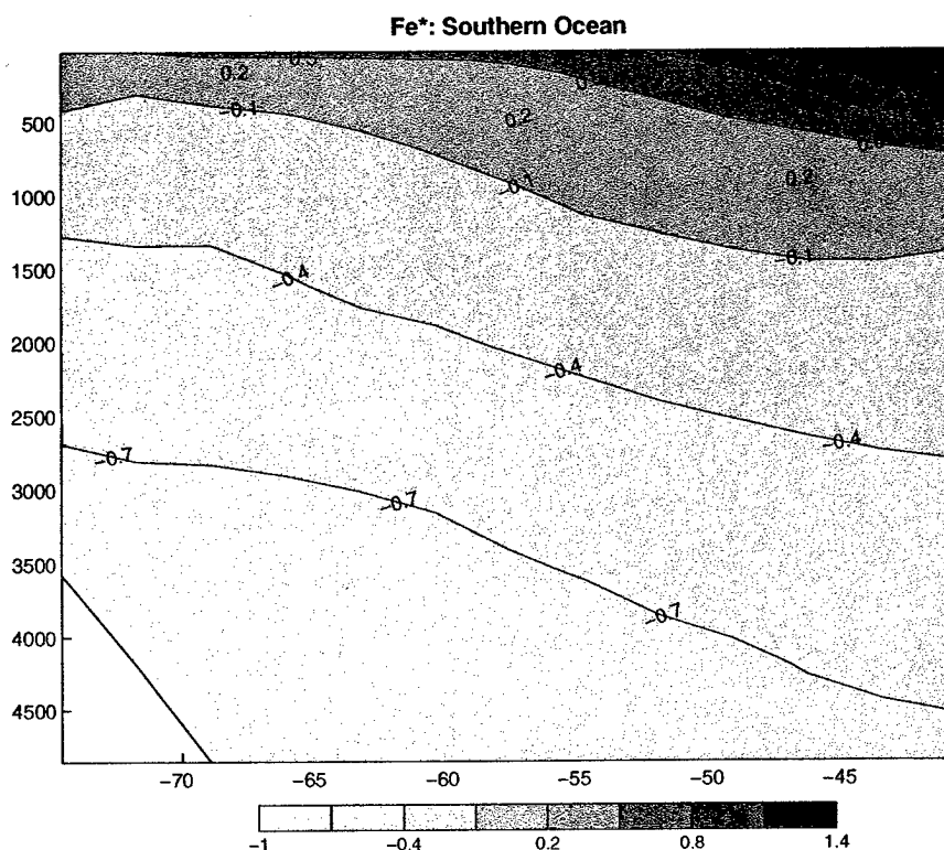
Figure 6-5: Zonally averaged Fe* in the Southern Ocean for the 'paleo' case.
