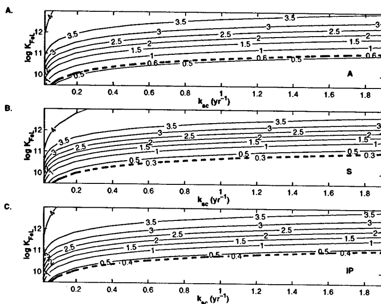
Figure 2-8: Complexation model: Sensitivity of modeled deep water [\text{Fe}_T] to scavenging rate ( k_{sc} , \text{yr}^{-1} ) and conditional stability constant ( \log K_{\text{Fe}'L} ) for the A) Atlantic, B) Southern Ocean, and C) Indo-Pacific basin with [\text{L}_T] = 4 nM. The dashed contour represents the observed average deep water [\text{Fe}_T] for each basin.
