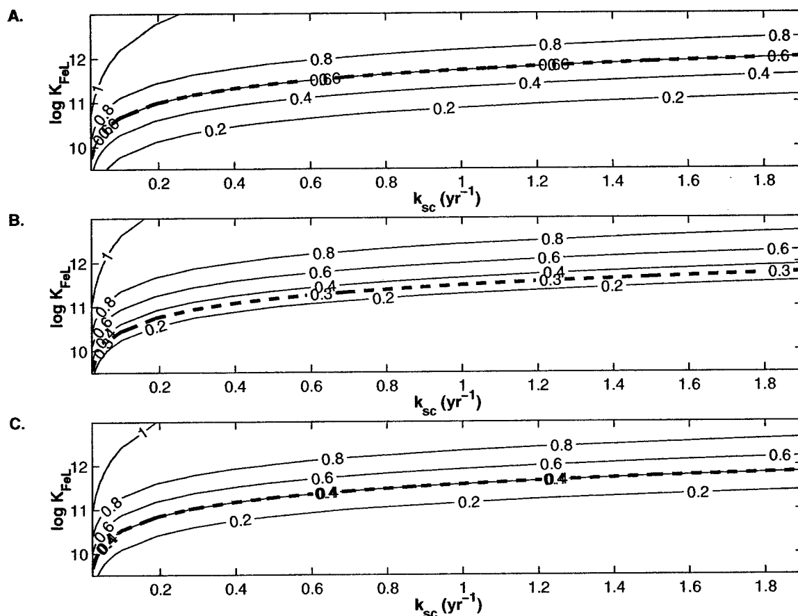
Figure 2-6: Complexation model: Sensitivity of [Fe_T] (nM) to scavenging ( k_{sc} , yr -1 ) and conditional stability constant ( \log K_{Fe'L} ) for the A) Atlantic, B) Southern Ocean, and C) Indo-Pacific basin with [L_T] = 1 nM. The dashed contour represents the average observed deep water [Fe] for each basin. The optimal solution is for k_{sc} between 0.2-1.8 yr -1 .
