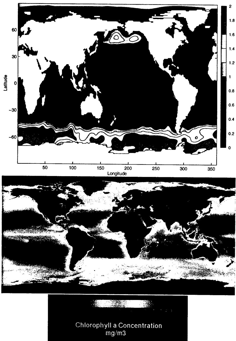
Figure 1-1: Top panel displays the surface \text{PO}_4 from Conkright et al. (1994) in \mu\text{M} . The bottom panel displays the yearly averaged chlorophyll a concentration ( \text{mg}/\text{m}^3 ) as sensed by SeaWiFs (Figure courtesy of NASA).
