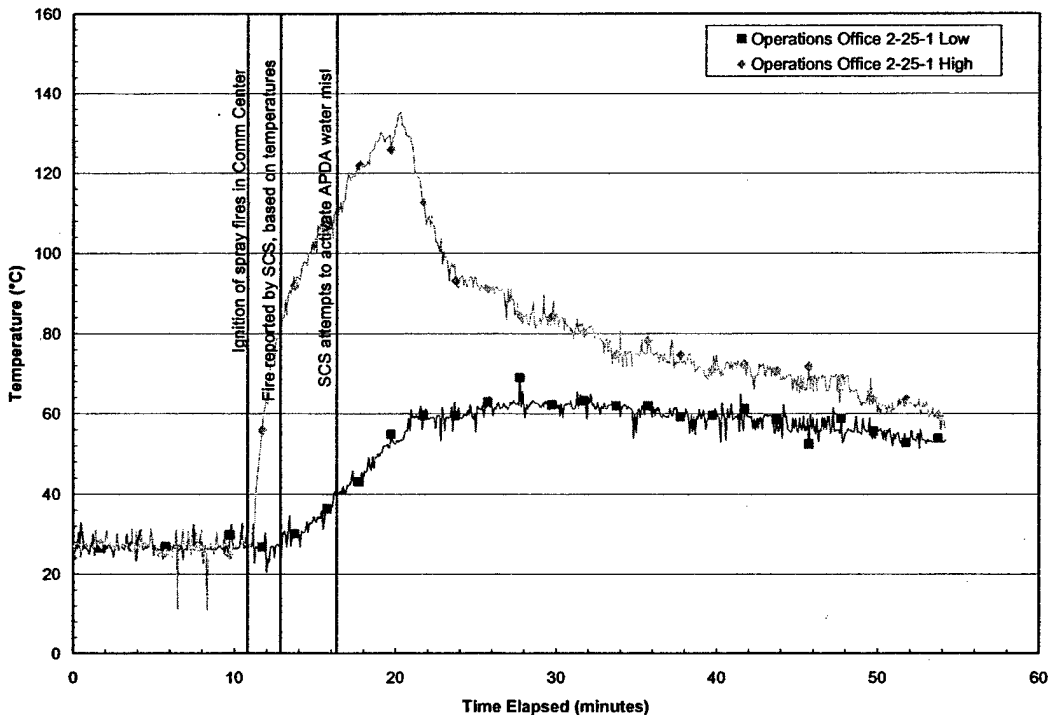
Fig. 23 – Operations Office high low thermocouples, afss15
