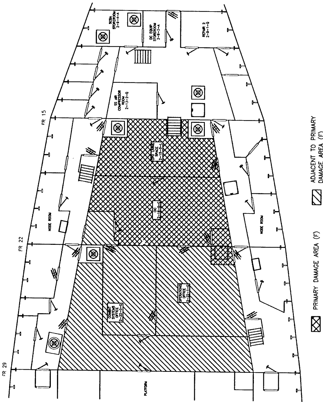
Fig. 12 - Compartment damage classification for the second deck
