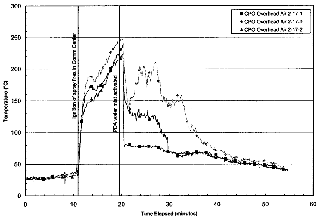
Fig. 22—CPO Living overhead air thermocouples, afss14
