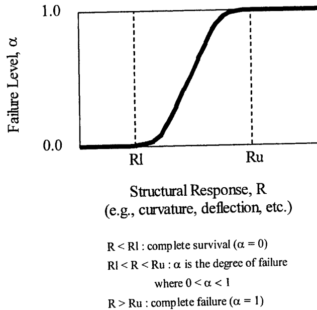
Figure 5.3-1. Vague Failure Model
