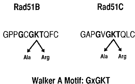
Figure 2. The Walker A motif in Rad51B and Rad51C. The Walker type A consensus sequence responsible for nucleotide binding is displayed on bottom.
