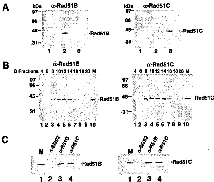
Figure 1. Rad51B and Rad51C form a stable complex. (A) Specificity of antibodies. Yeast cells harboring the empty expression vector pPM231 (2 \mu , GAL-PGK ; lane 1), the Rad51B expression plasmid pR51B.1 (2 \mu , GAL-PGK-RAD51B ; lane 2), and the Rad51C expression plasmid pR51C.1 (2 \mu , PGK-RAD51C ; lane 3) were run in an 11% polyacrylamide gel and then subjected to immunoblot analysis with either anti-Rad51B ( \alpha -Rad51B; left panel) or anti-Rad51C antibodies ( \alpha -Rad51C; right panel). (B) Rad51B and Rad51C are associated in a complex in human cells. HeLa cell extract was fractionated in a Q Sepharose column, and the indicated fractions were run in an 11% gel and then subjected to immunoblot analysis with anti-Rad51B antibodies ( \alpha -Rad51B; left panel) or anti-Rad51C antibodies ( \alpha -Rad51C; right panel). Yeast extracts containing Rad51B (lane 10 in left panel, marked M) or Rad51C (lane 10 in right panel, marked M) were used to help identify these proteins in the Q column fractions. (C) Coimmunoprecipitation of Rad51B and Rad51C from the Q column fractions. The Q Sepharose pool (fractions 8–16) was subjected to immunoprecipitation with protein A beads containing anti-ySrs2 antibodies ( \alpha -SRS2), anti-Rad51B antibodies ( \alpha -R51B) and anti-Rad51C antibodies ( \alpha -R51C). Proteins bound to the various immunobeads were eluted by SDS treatment and analyzed for their content of Rad51B (left panel) and Rad51C (right panel).
