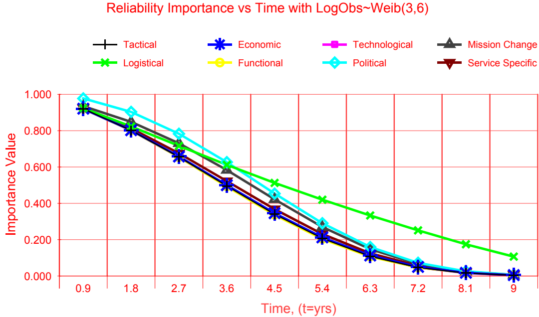
Figure 4-6. Graph of the Reliability Importance versus Time with Phase I Improvements
