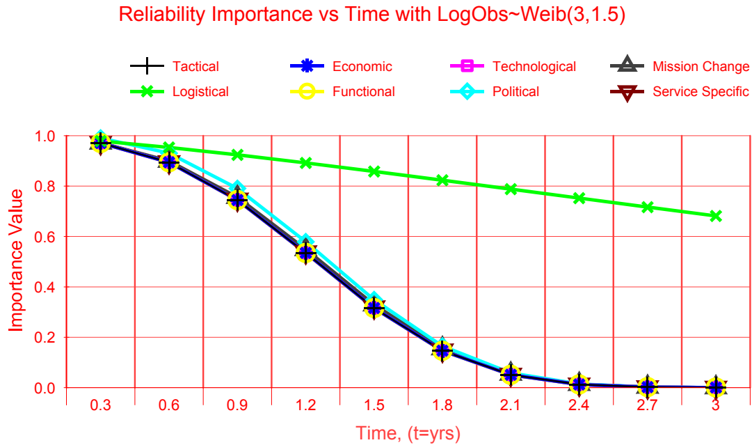
Figure 4-3. Graph of the Reliability Importance versus Time for Current Configuration
