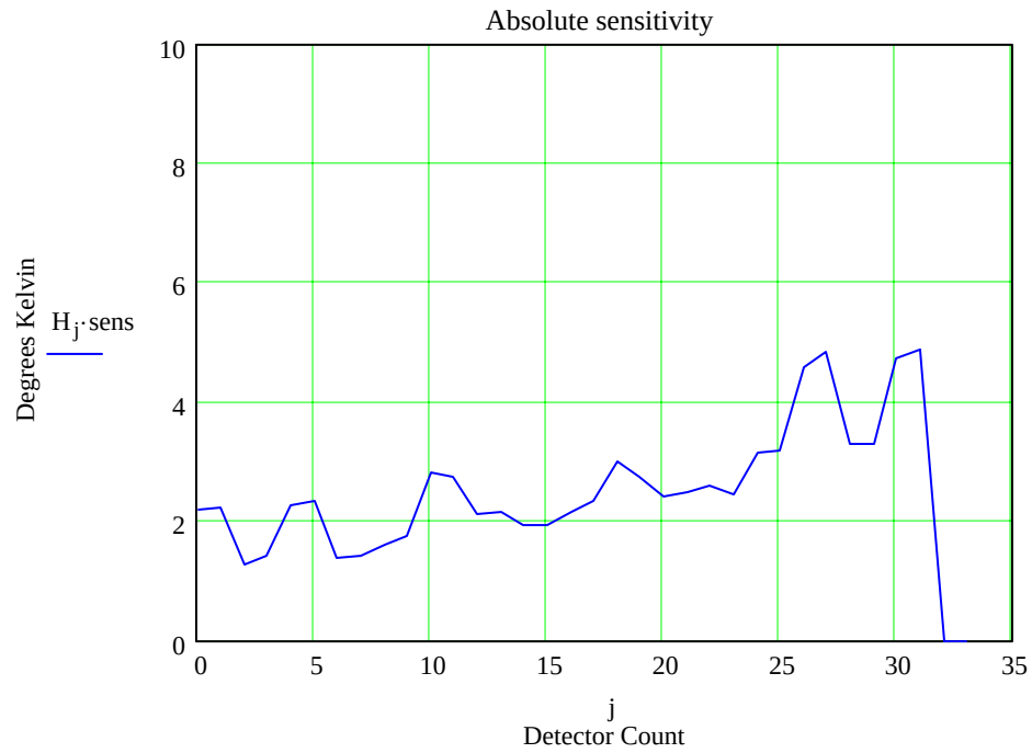
Figure 2.6-2. Absolute Sensitivity
