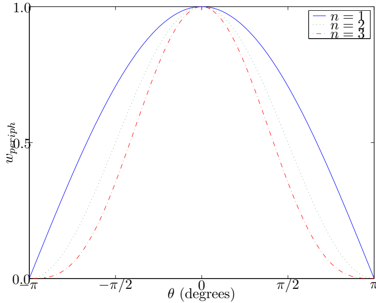
Figure 4.5 Peripheral Weight
