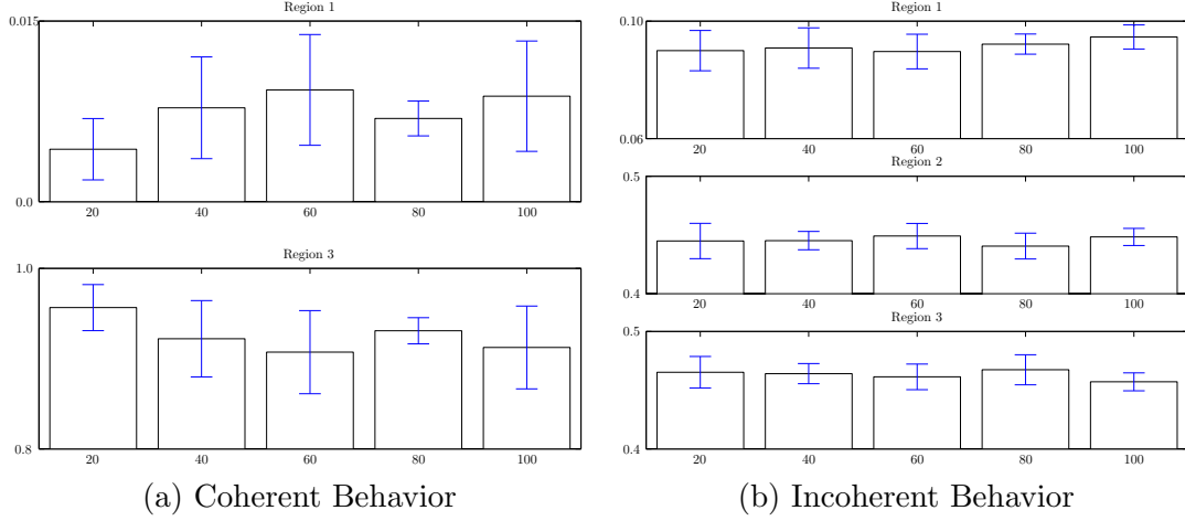
Figure 7.3 Region Proportions
