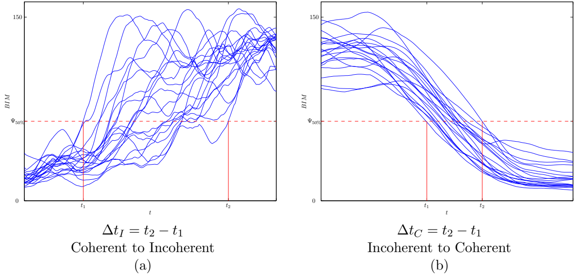
Figure 6.20 Behavior Transition
