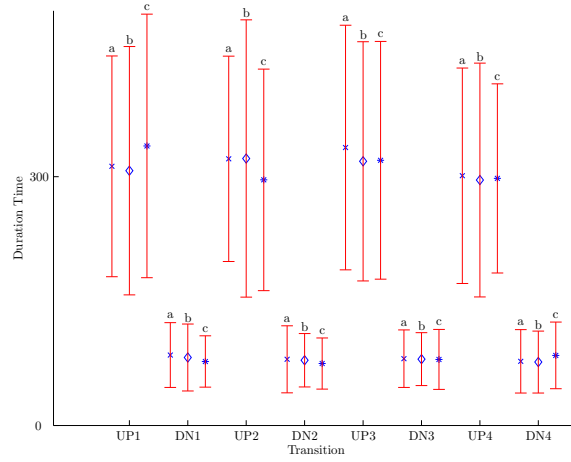
Figure 7.1 Transition Duration
