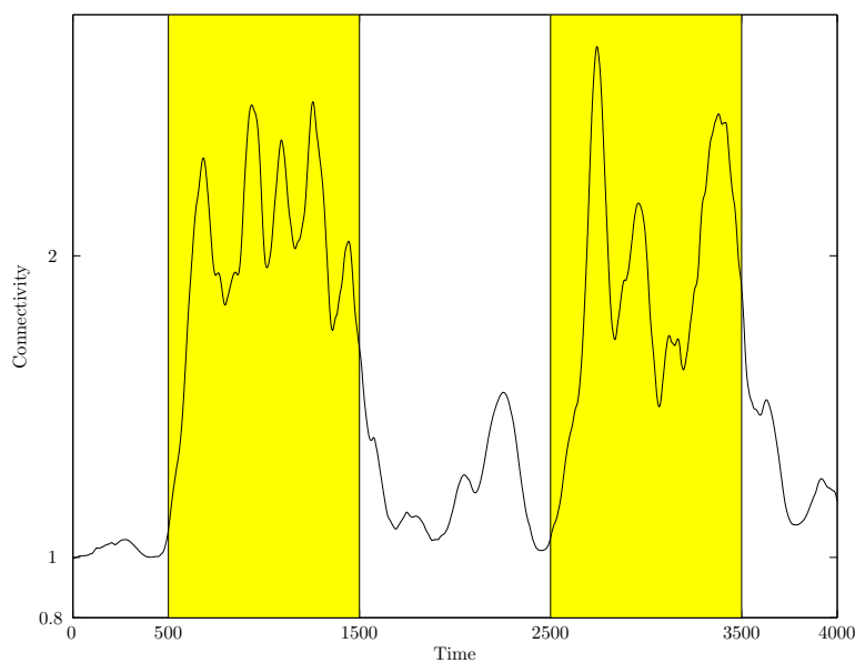
Figure 6.1 Connectivity
