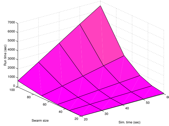
Figure C.2 OPNET run-time
