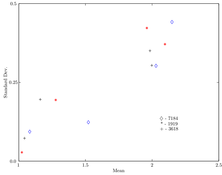
Figure 6.2 Connectivity Variations
