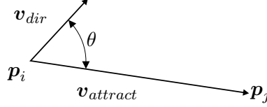
Figure 4.6 Peripheral Weight
