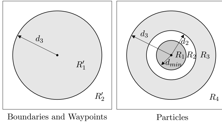
Figure 4.4 Neighborhood models
