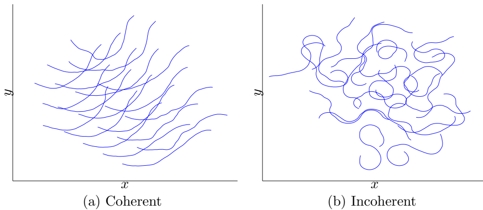
Figure 6.3 Behavior Sample
