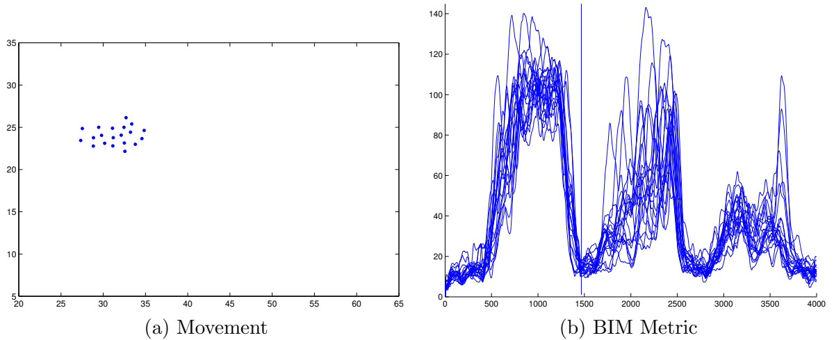
Figure I.1 Swarm Animation
