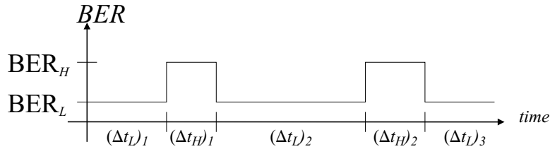
Figure 2.8 Bit Error Rate Model
