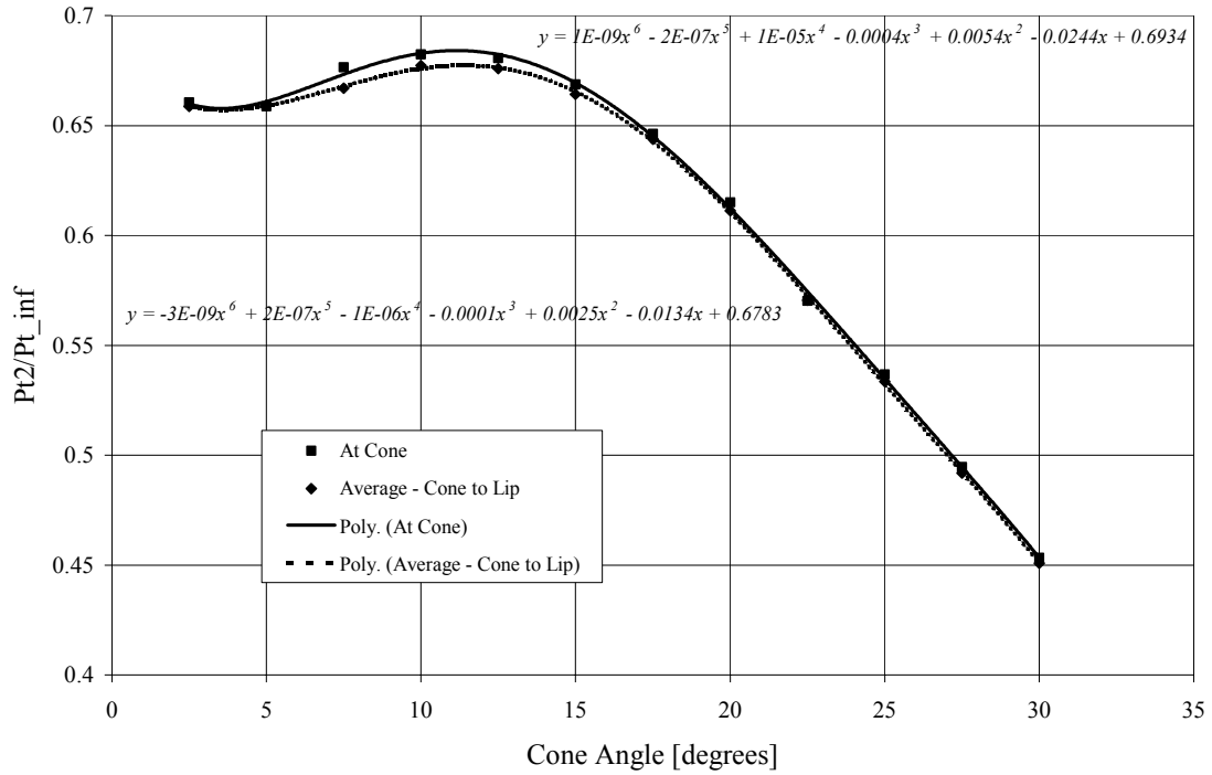
Figure 38. Normal shock recovery pressure ratio vs. cone angle at cone and lip of inlet cowl at Mach 4.0
