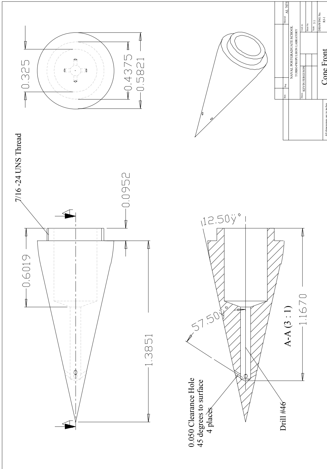
Figure 44. Part drawing: Ramjet inlet nose cone (RJ-1)
