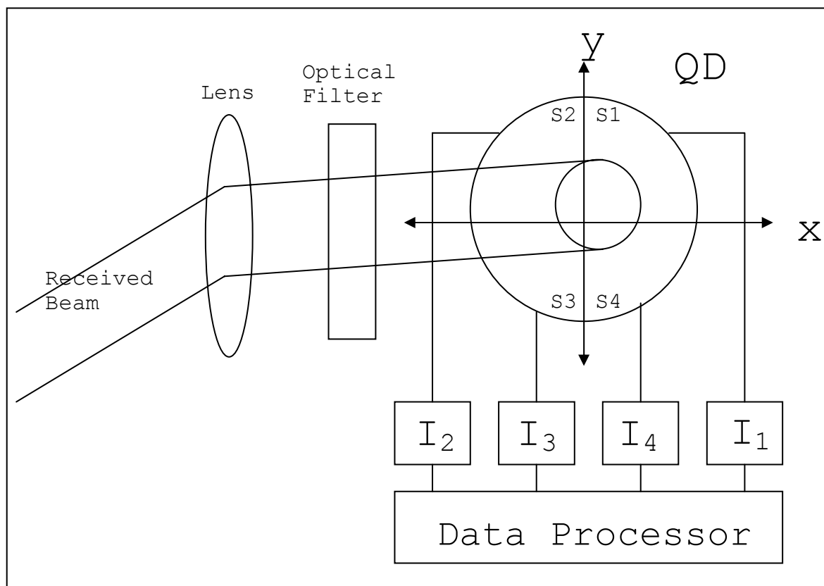
Figure 13. Quadrant Detector (QD) [After Ref 14]
