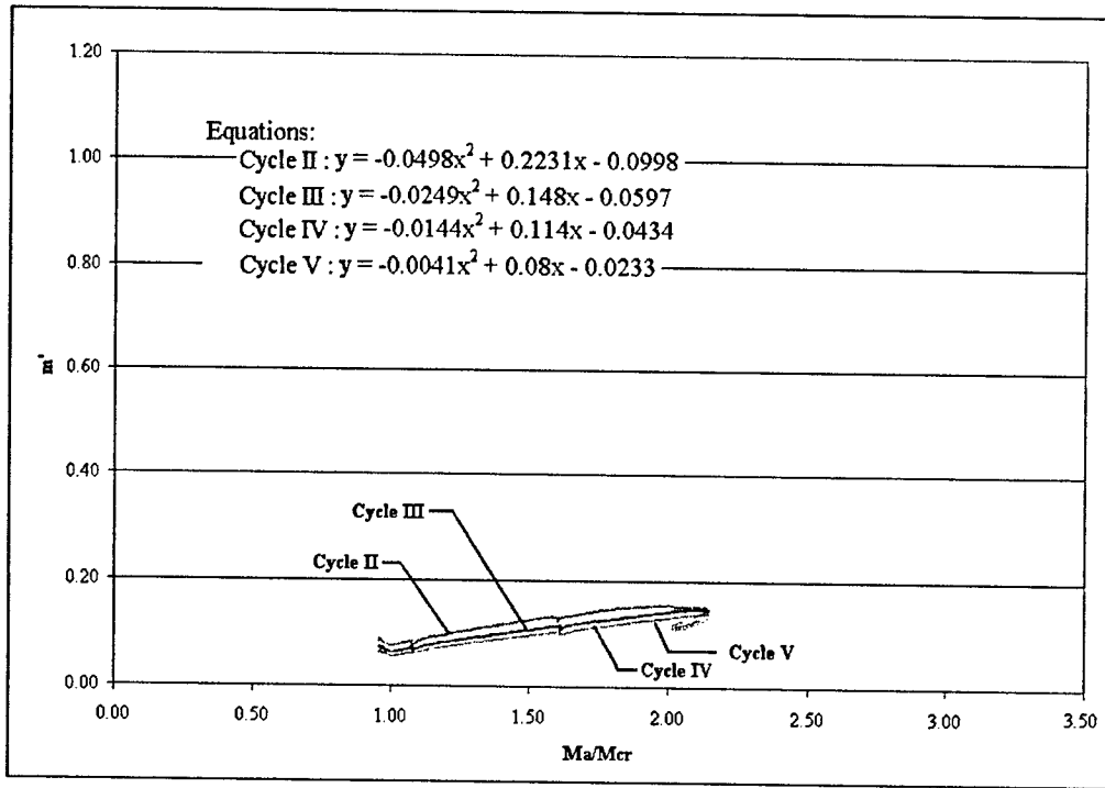
Figure C.9 - Exponent m' versus Applied Load (Specimen C3)
