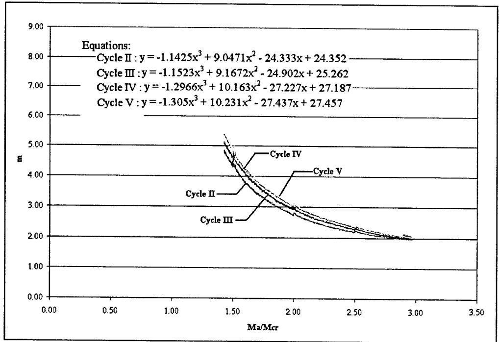
Figure B.6 - Exponent m versus Applied Load (Specimen C5)
