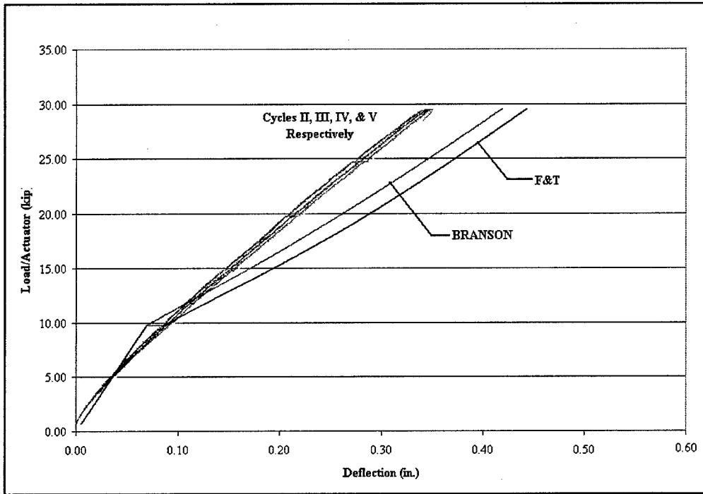
Figure 5.12. Typical Load versus Live-load Deflection A_g=8 \text{ in.}^2 (Specimen B8)
