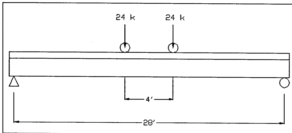
Figure 3.3. AASHTO Alternative Military Load Configuration
