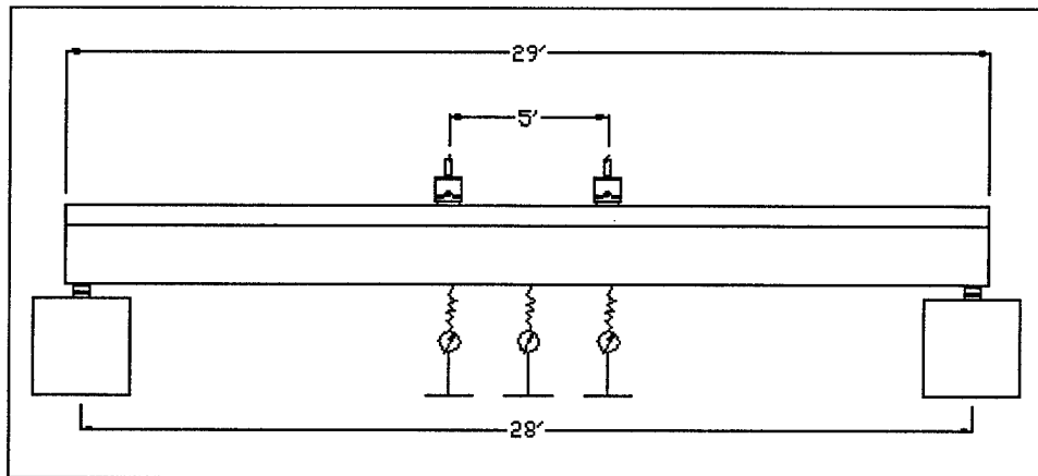
Figure 3.8. LVDTs Location on T-beam Specimen
