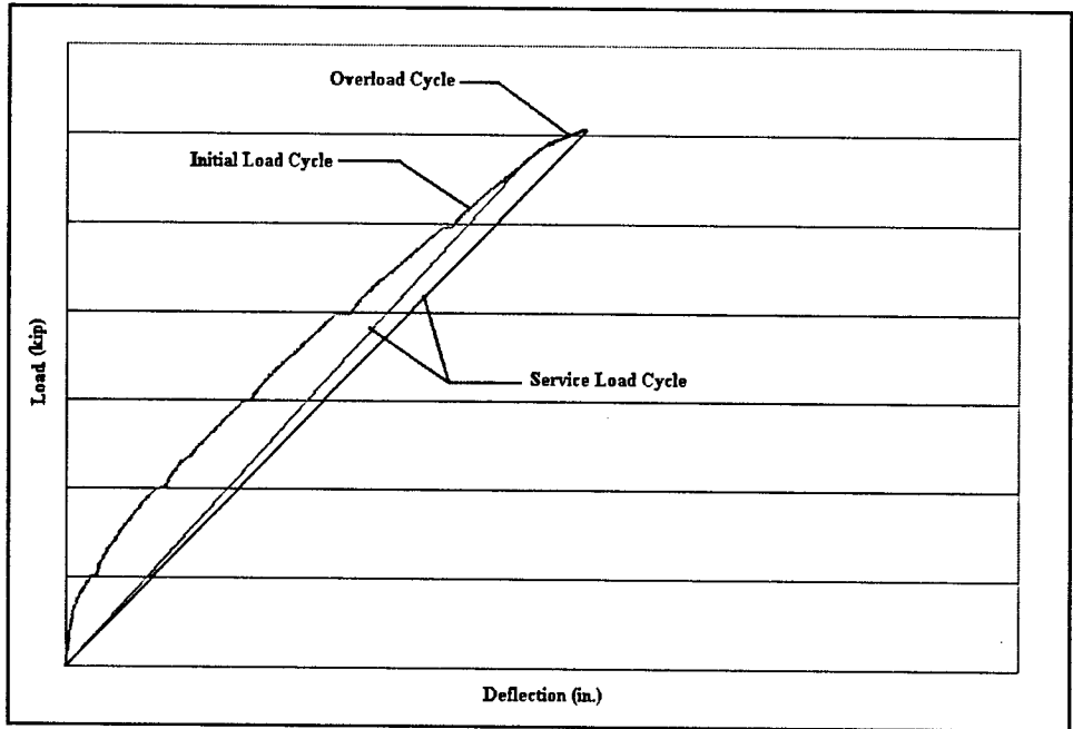
Figure 4.7. Life-cycle Behavior of T-beam Bridge Girder
