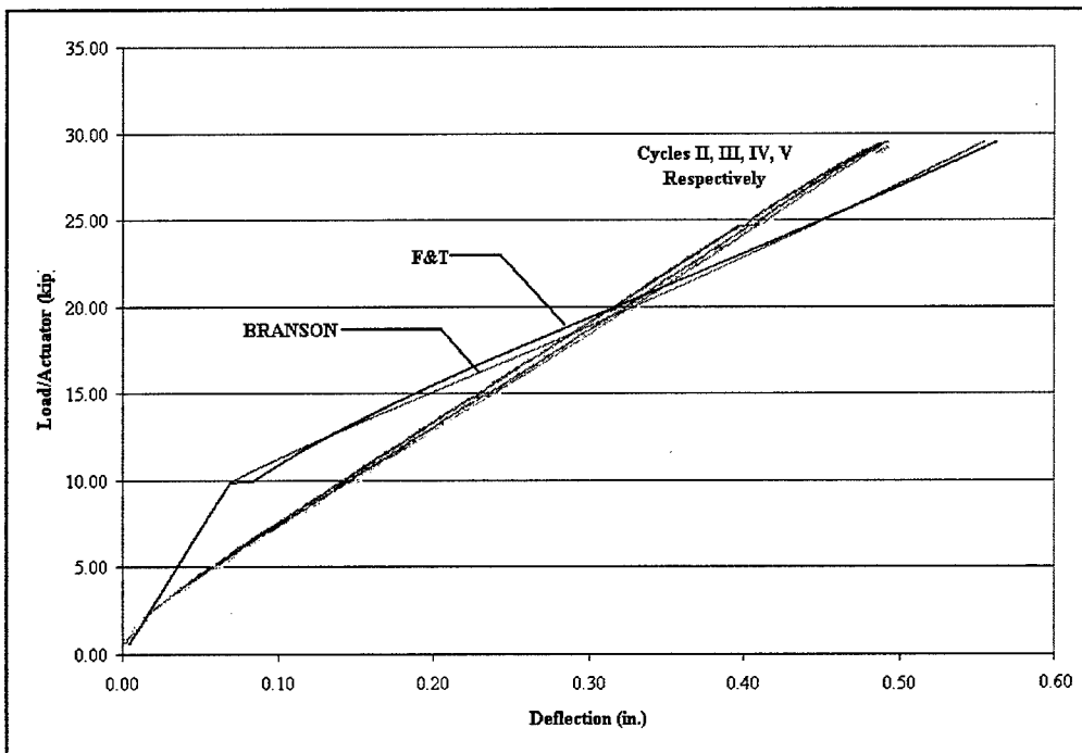
Figure 5.13. Typical Load versus Live-load Deflection A_g=5 \text{ in.}^2 (Specimen C5)
