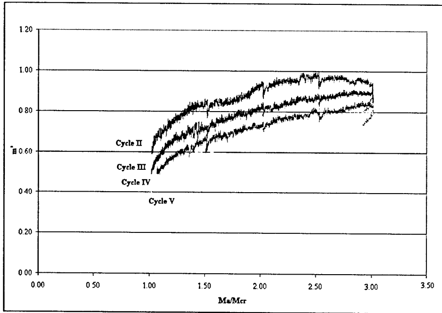
Figure 5.11. Typical m' versus Applied Load (Specimen B8) For A_s = 3 \text{ in.}^2 :
