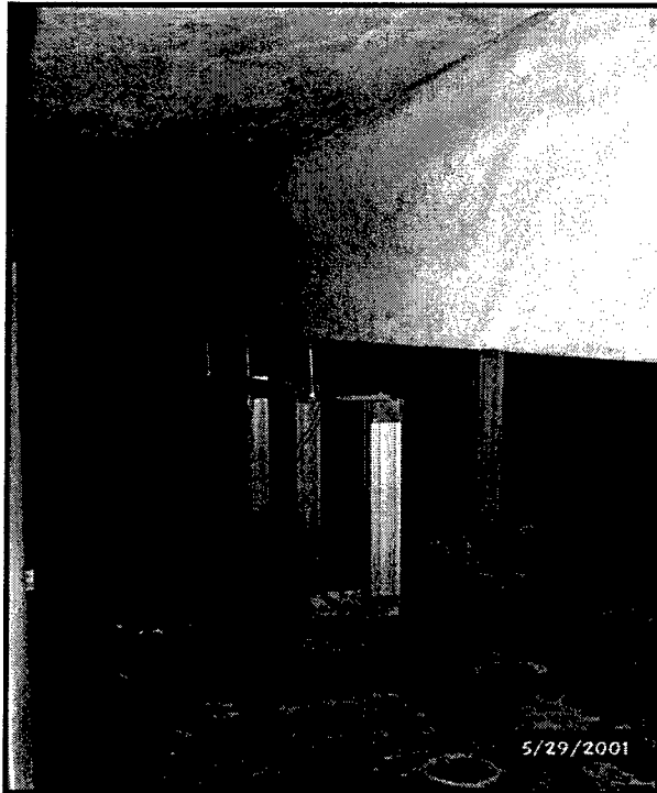
Figure 3.8. LVDTs Location on T-beam Specimen
