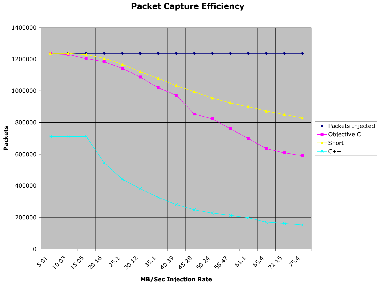
Figure 11. Packet Capture Efficiency
