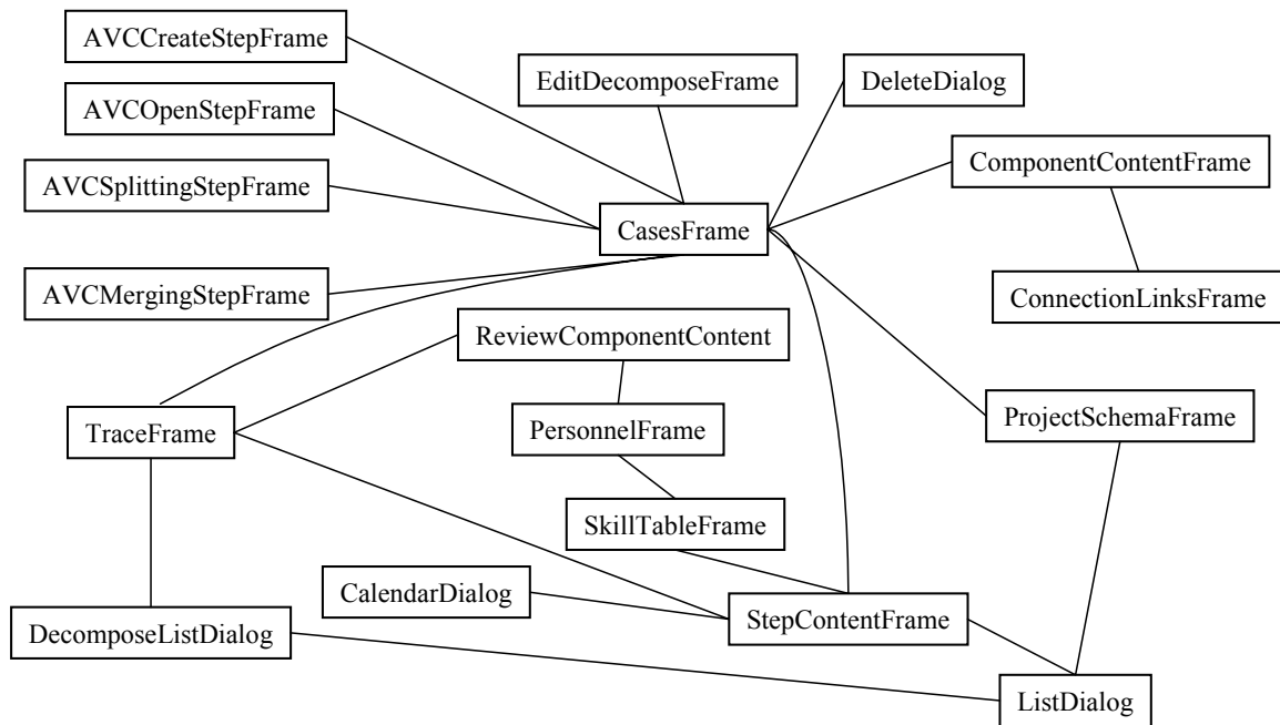
Figure 12 CASES 1.1 Elided Class Diagram (after [LEHC99])
