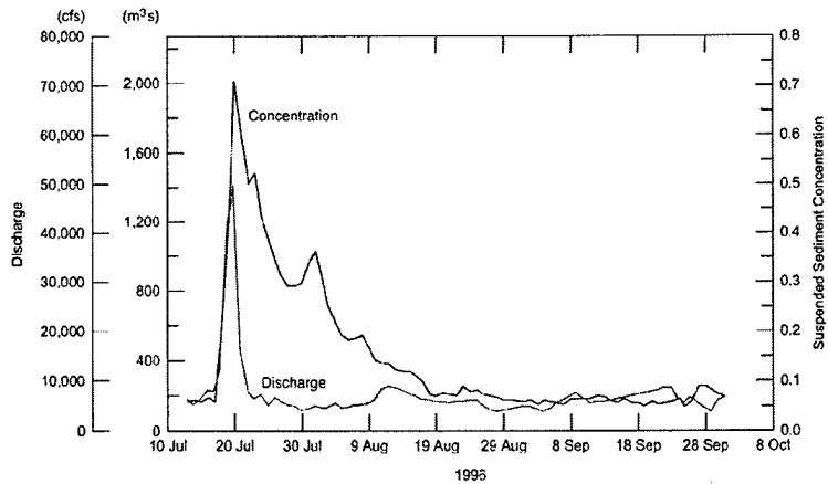
Figure 10. Hydrograph for water discharge and sediment concentration at the point of inflow.
