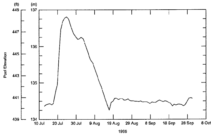
Figure 9. Observed downstream 1996 hydrograph.
