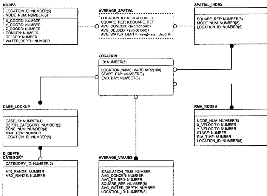
Figure 12. The entity relationship (ER) of data for the Peoria Lake Pilot Study.
