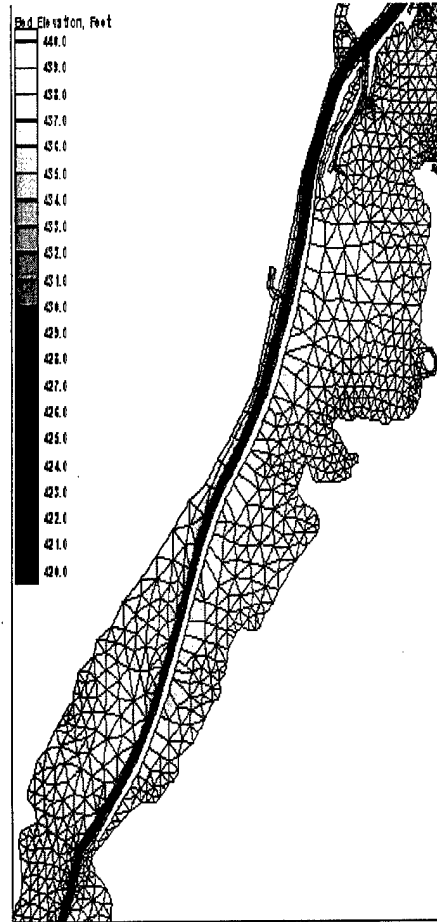
Figure 8. Grid of Upper Peoria Lake with levee, including bathymetry data used by RMA2 and SED2D.
