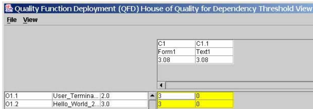
Figure 83 Dependency Threshold: S1.1 x C1.1, d = \text{Difficulty} , t = \mu
