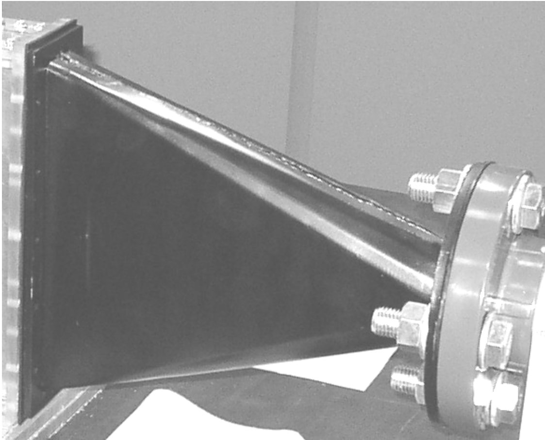
Figure 9. Exit duct
