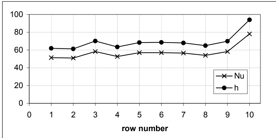
Figure 24. Row by row results of Nusselt number and heat transfer coefficient for case I \Delta T +6 , Reynolds number \sim 4500
