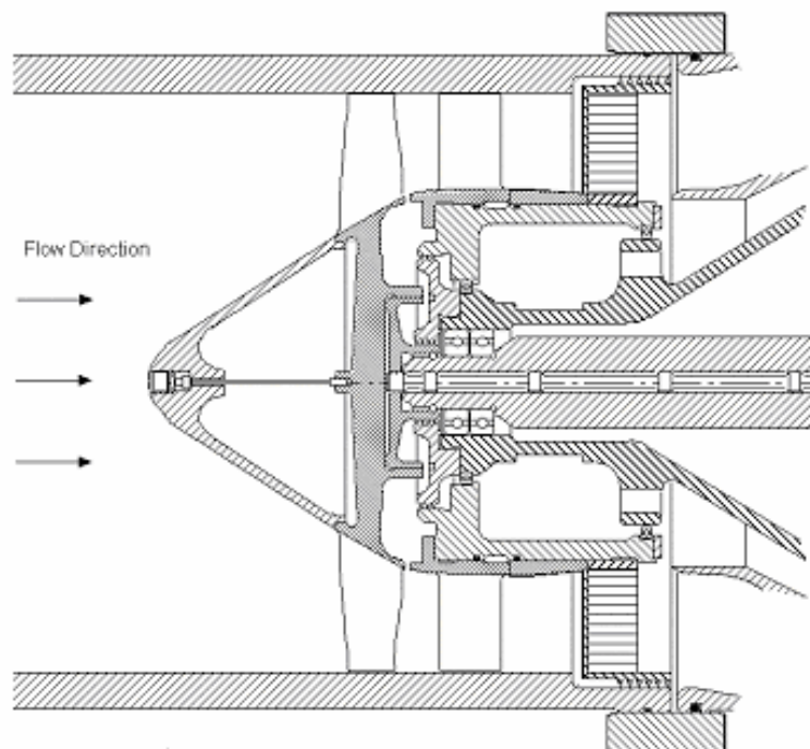
Figure 3. Transonic Compressor
