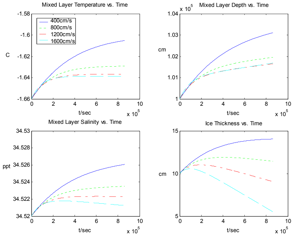
Figure 14. Simulation #5: Sensitivity study for varying winds with h = 1000 m, Q_0 = 0.0010 cal/cm 2 s, and ratio of \alpha_0 g \Delta T to \beta_0 g \Delta S equal to 0.45. Wind speed changes from 400 cm/s to 1600 cm/s in 400 cm/s intervals.
