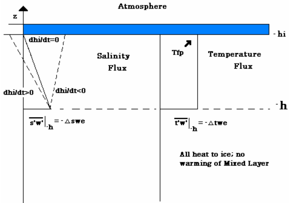
Figure 8. Representative temperature and salinity flux profiles for the high latitude regions.
