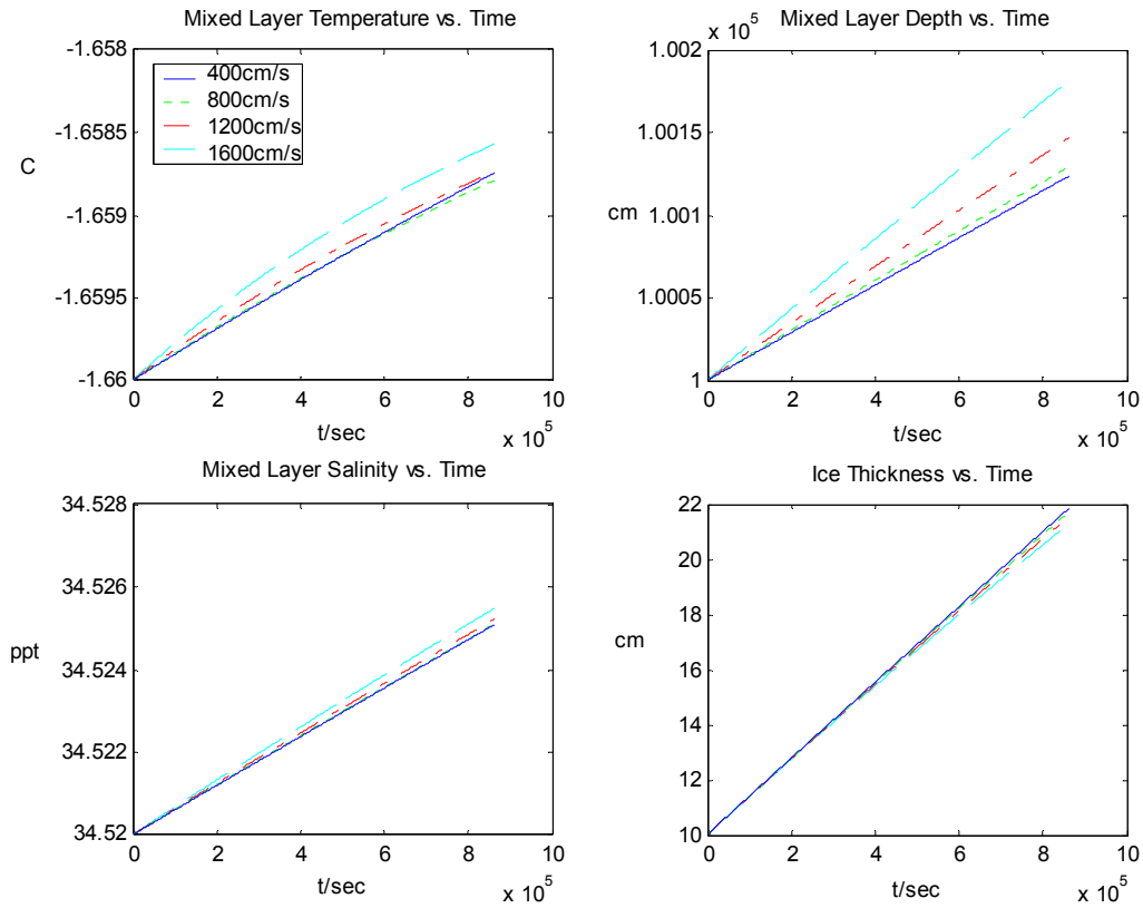
Figure 15. Simulation #6: Sensitivity study for varying winds with h = 1000 m, Q_0 = 0.0010 cal/cm 2 s, and ratio of \alpha_0 g \Delta T to \beta_0 g \Delta S equal to 0.036. Wind speed changes from 400 cm/s to 1600 cm/s in 400 cm/s intervals.
