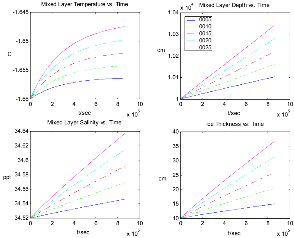
Figure 13. Simulation #4: Sensitivity study for heat fluxes with h=100 m, wind speed =700 cm/s, and ratio of \alpha_0 g \Delta T to \beta_0 g \Delta S equal to 0.036. Heat flux changes from 0.0005 cal/cm 2 /s to 0.0025 cal/cm 2 /s in 0.0005 cal/cm 2 /s intervals.
