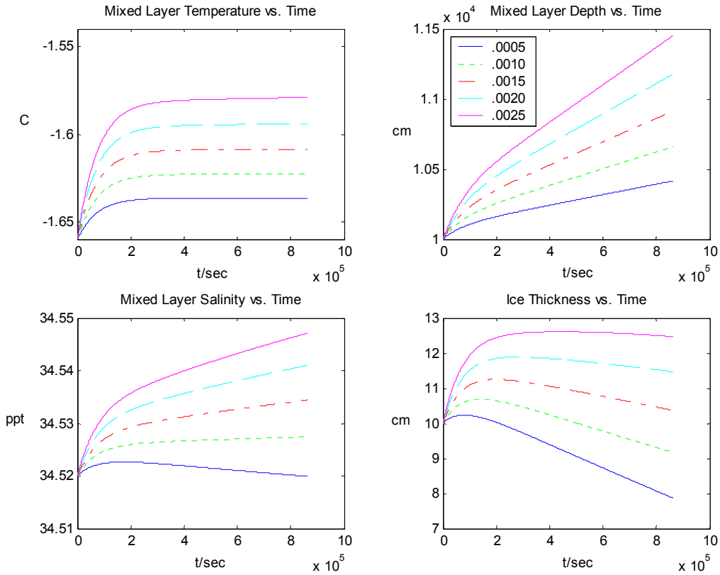
Figure 12. Simulation #3: Sensitivity study for heat fluxes with h=100 m, wind speed =700 cm/s, and ratio of \alpha_0 g \Delta T to \beta_0 g \Delta S equal to 0.45. Heat flux changes from 0.0005 cal/cm 2 s to 0.0025 cal/cm 2 s in 0.0005 cal/cm 2 s intervals.
