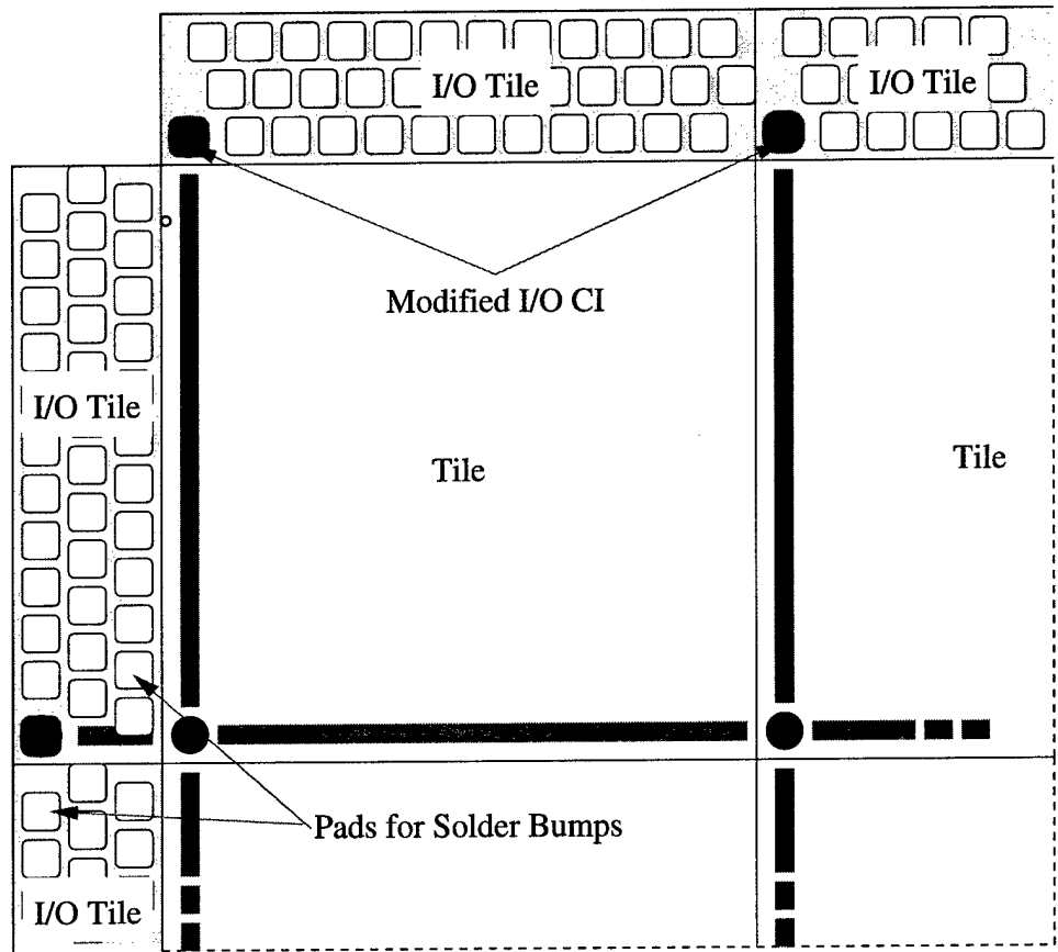
Figure 6.8. Input and Output Tiles
