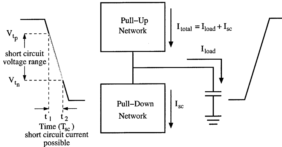
Figure 2.6. Source of Short Circuit Power
