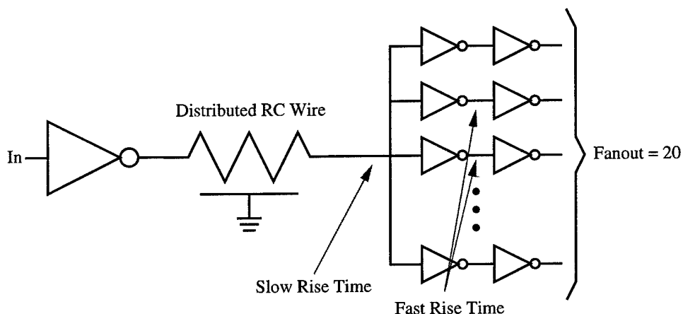
Figure 2.7. Example Circuit with Short Circuit Power Consumption
