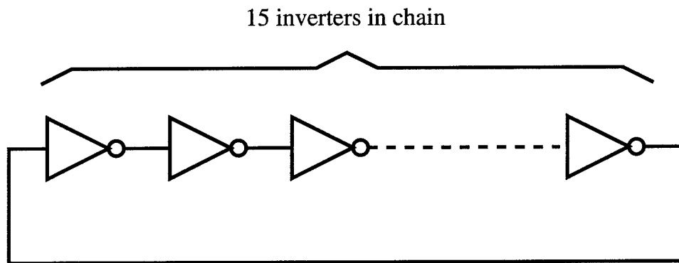
Figure 2.2. Ring Oscillator
