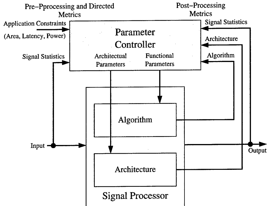
Figure 3.2. Dynamically Parameterized System Approach
