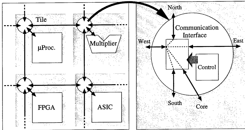
Figure 1.2. Tiled Architecture
