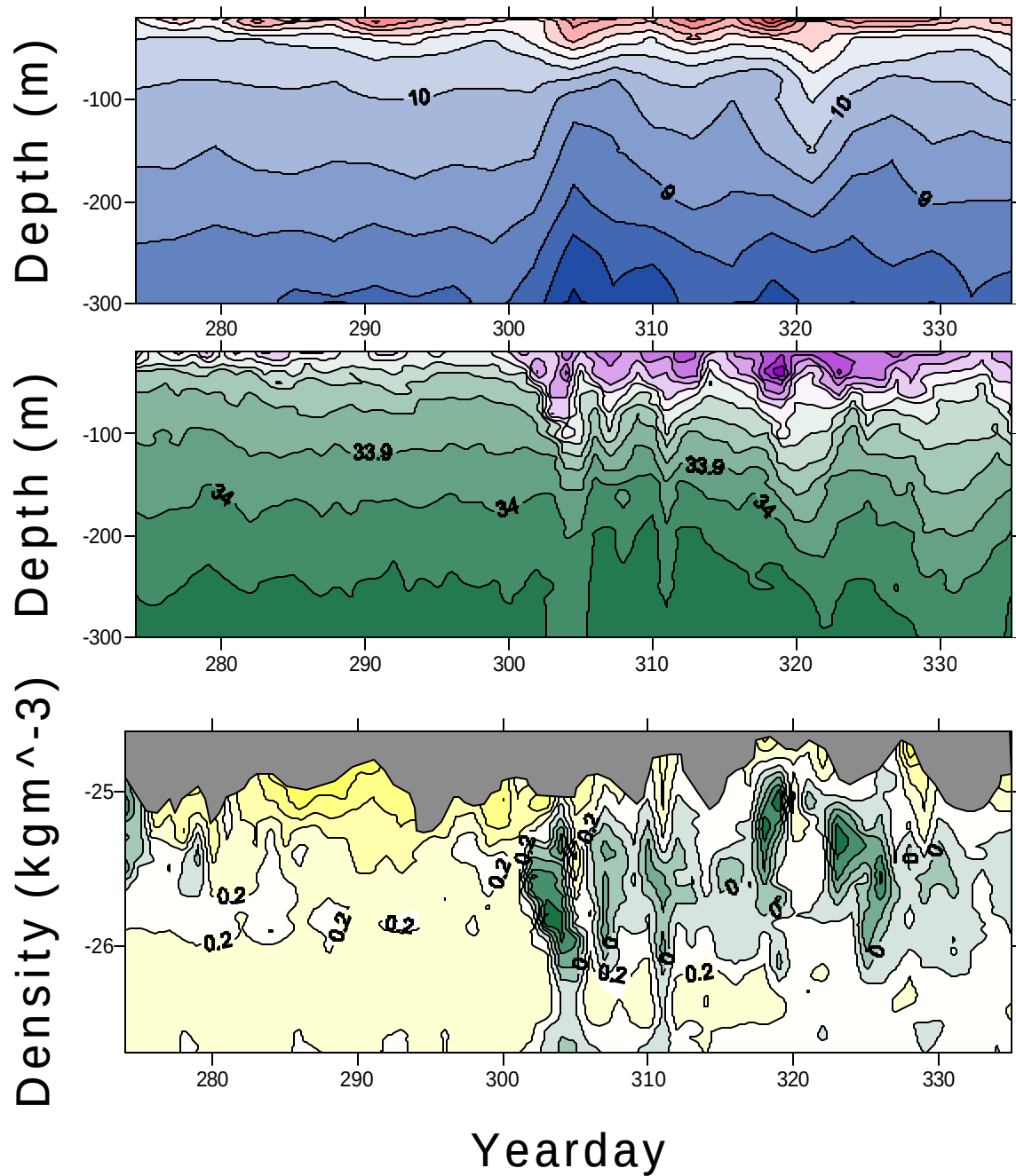
Figure II-8. Water properties at M2 over time (yearday). (top) Temperature ( ^{\circ}\text{C} ) stratification with depth (m). Contour interval is 0.5^{\circ}\text{C} . (middle) Salinity stratification with depth (m). Contour interval is 0.1. (bottom) Density anomaly ( \text{kg m}^{-3} ) versus yearday (yearday). The contour interval is 0.1 \text{ kg m}^{-3} . The lower limit for the gray region shows the minimum (surface) density anomaly.
