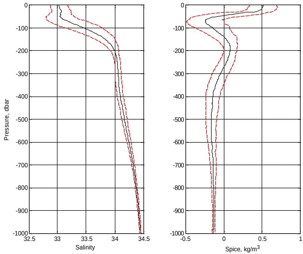
Figure III-5. Vertical profiles. (left) Mean salinity (black line) \pm one standard deviation. (red lines). (right) Mean spice (black line) \pm one standard deviation (red lines).
