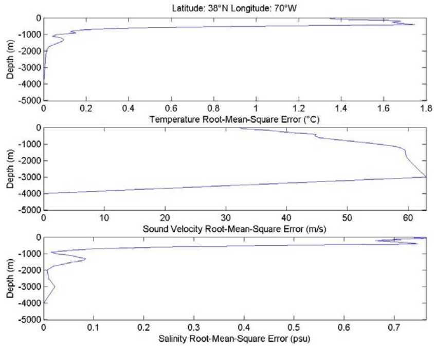
Figure 58. RMSD Profile
