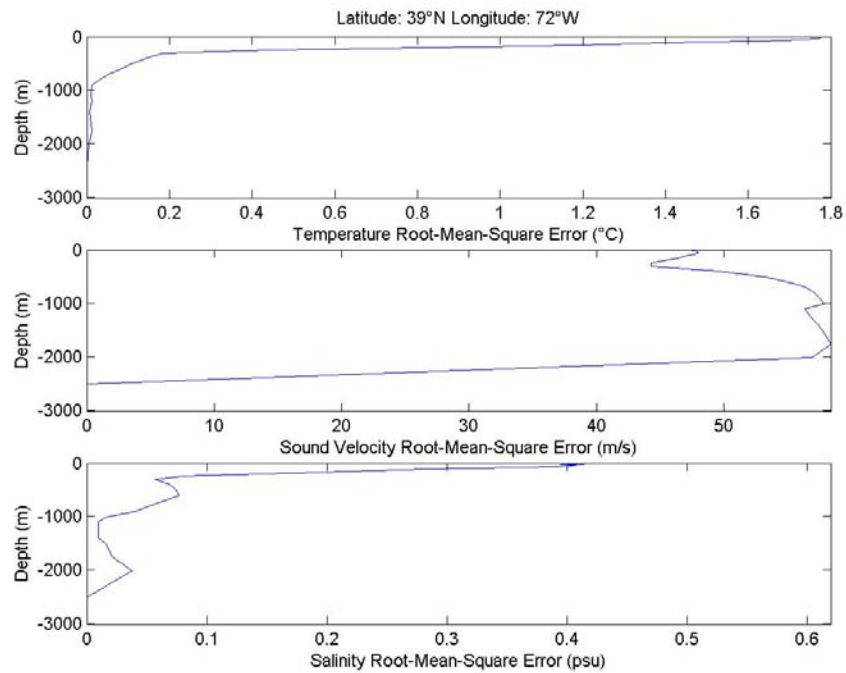
Figure 62. RMSD Profile
