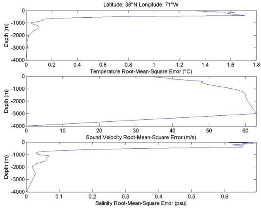
Figure 57. RMSD Profile
