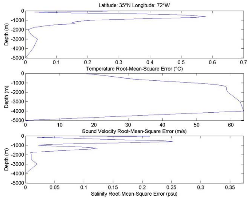
Figure 38. RMSD Profile
