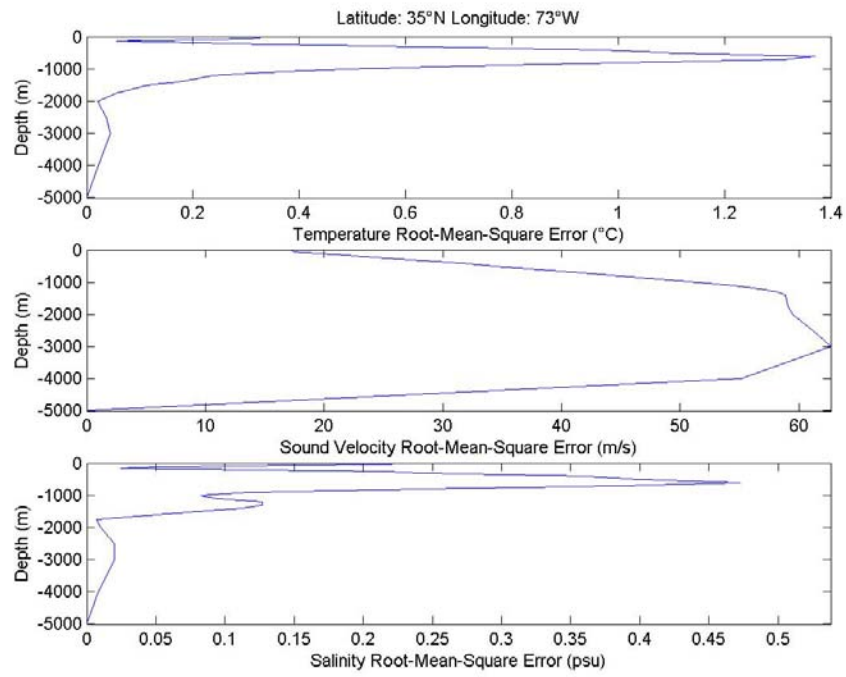
Figure 37. RMSD Profile
