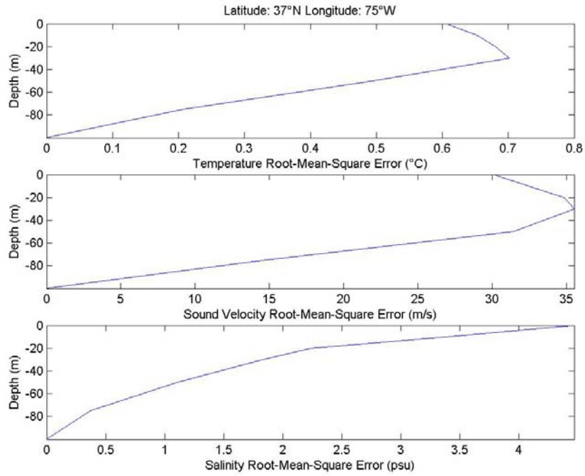
Figure 47. RMSD Profile
