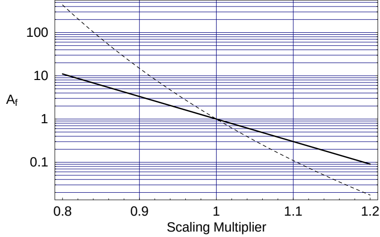
Figure 3.7: A_{f_{TDDB}} versus scaling multiplier. For T (dashed line) and \mathcal{C}_{ox} (solid line). E_{a_{TDDB}} = 0.75 \text{ eV} , T = 85^\circ\text{C} , E_{ox} = 4 \text{ MV/cm} , \gamma = 3 Naperians per MV/cm.
