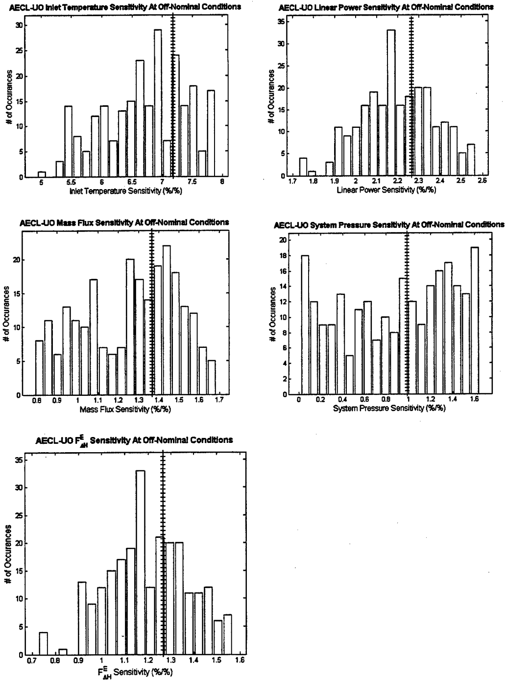
Figure 25: AECL-UO Look-Up Table Correlation Sensitivities.
