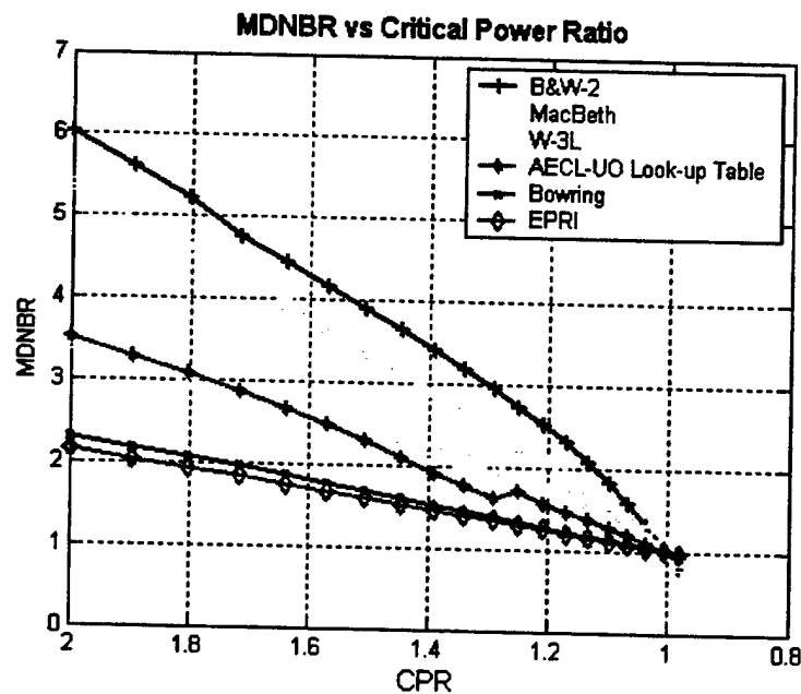
Figure 11: IRIS Open MDNBR vs CPR
