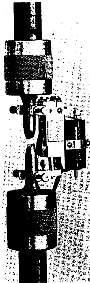
Fig. 14 Breakaway-type LVDT extensometer (50 mm, or 2 in. gage length) that can remain on the specimen through rupture
