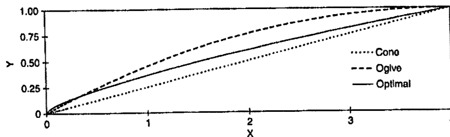
Fig. 7. Comparison of conical, ogival and optimal shapes for a penetrator with a = 1 and b = 4 ( \alpha = 0.25 )
