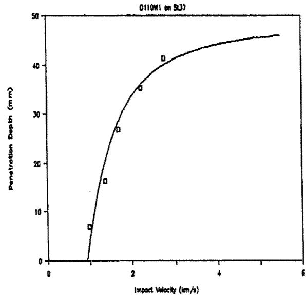
Figure 10b. Penetration Depth (mm) vs Impact Vel.(km/s)
