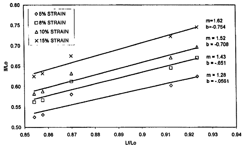
Figure 5. The results of 4340 steel impact tests.
