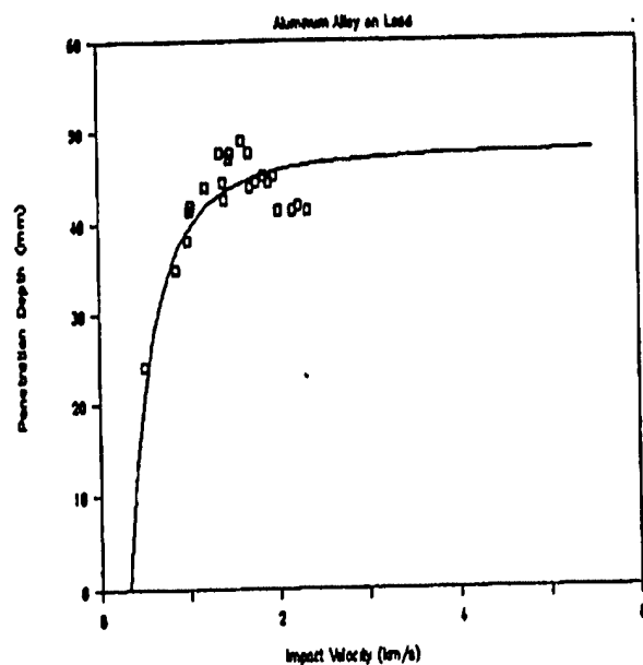
Figure 7b. Penetration Depth (mm) vs Impact Vel. (km/s)
