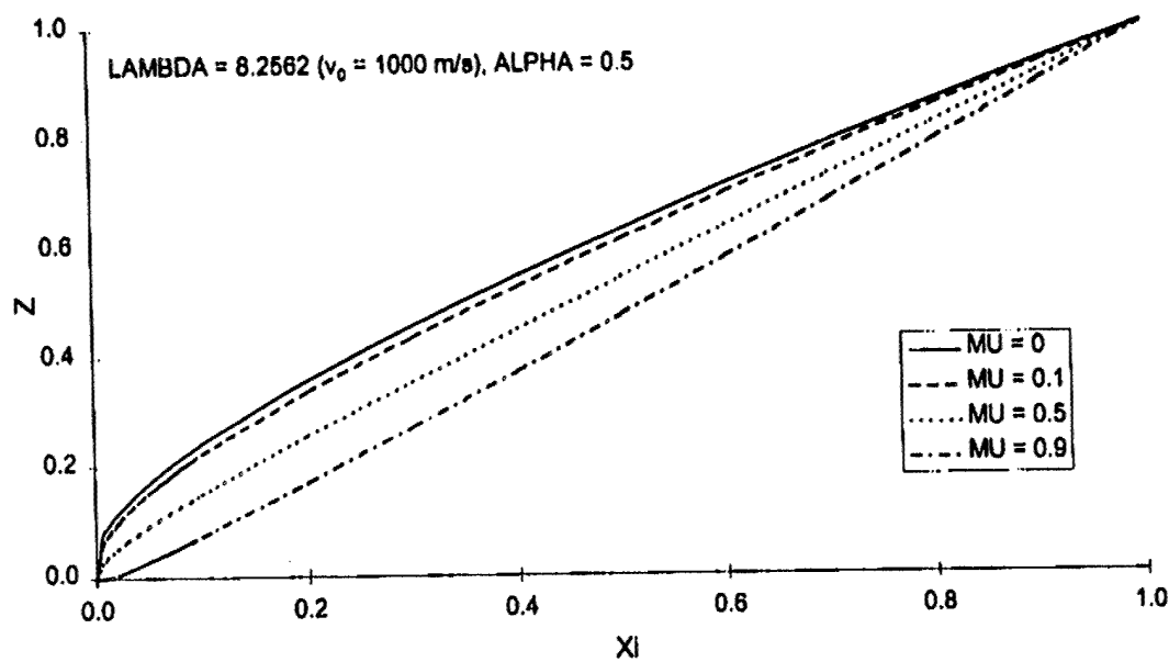
Fig. 5. Plots of optimal nose shape for \alpha = 0.5 and \lambda = 8.2562 ( v_0 = 1000 m/s) for various values of friction coefficient \mu .
