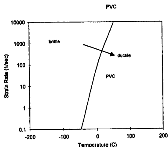
Fig. 2. Brittle-ductile transition for tensile failure: PVC.
