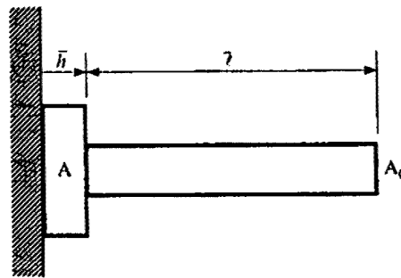
Fig. 9. Elementary mushrooming rod geometry. The mushroom is a cylinder with cross-sectional area A = A_0/(1 + e) . The undeformed section is a cylinder of length \bar{z} with cross-sectional area A_0 .
