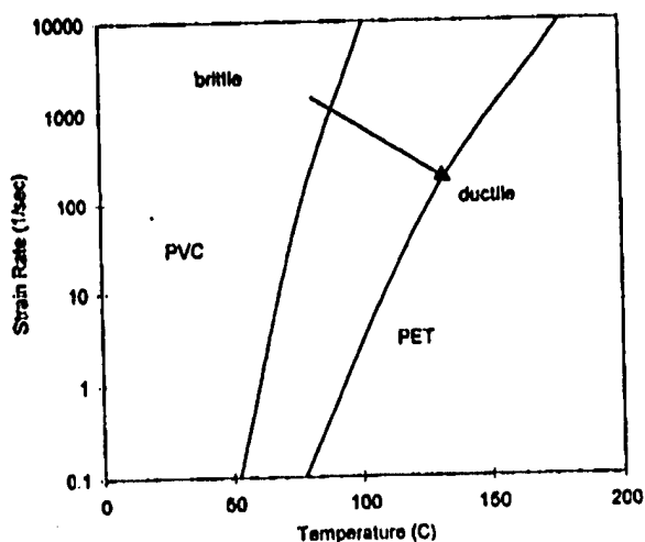
Fig. 5. Brittle-ductile transition for compressive failure: PVC and PET.
