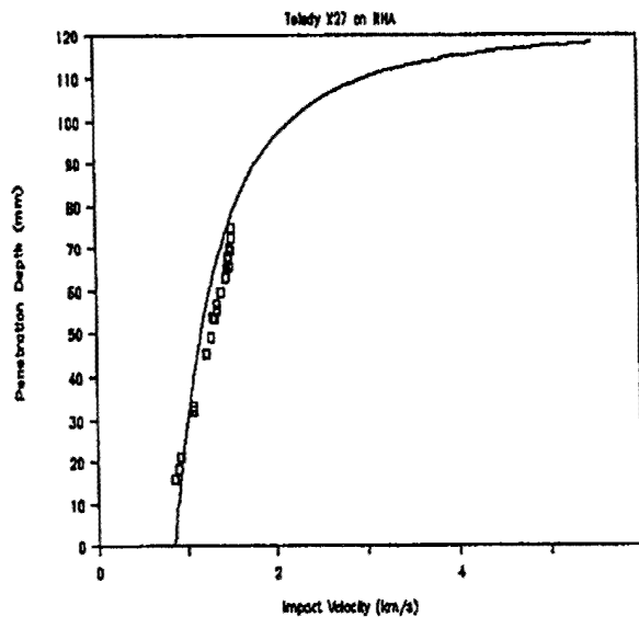
Figure 14b. Penetration Depth (mm) vs Impact Vel. (km/s)
