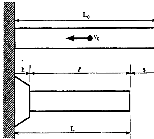
Fig. 1. A uniform cylinder of length L_0 impacts an uncompliant target with velocity v_0 . Subsequent deformation of the specimen can be successfully modeled in terms of deformed and undeformed regions h and \ell . L is the current overall specimen length and s is the displacement of the back end of the specimen.
