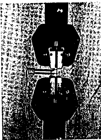
Fig. 18 Test setup using wedge grips on (a) a flat specimen with axial extensometer and (b) a round specimen with diametral extensometer
