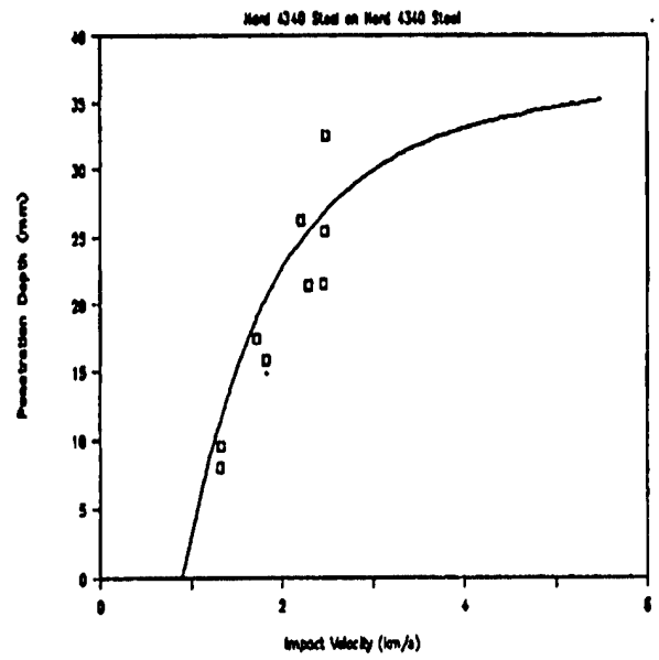
Figure 19b. Penetration Depth (mm) vs Impact Vel.(km/s)
