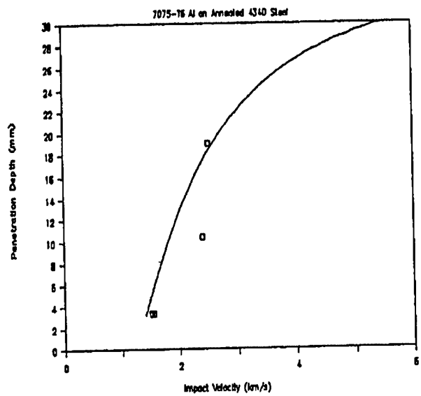
Figure 16b. Penetration Depth (mm) vs Impact Vel.(km/s)
