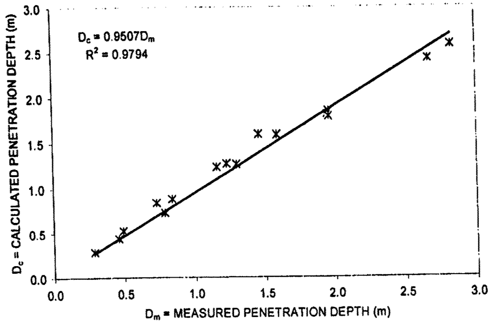
Figure 5. Plot of measured versus calculated penetration depths obtained by applying Equation (9) to the data of Table 3 with the parameters R+M\tau_0 = 478 MPa and \mu = 0.0 . The parameters were obtained by a least squares fitting process.
