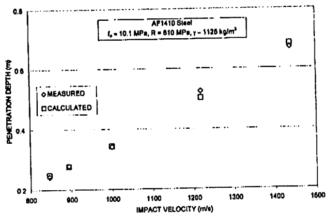
Figure 6. Plot of penetration depth versus impact velocity for AF1410 steel.
