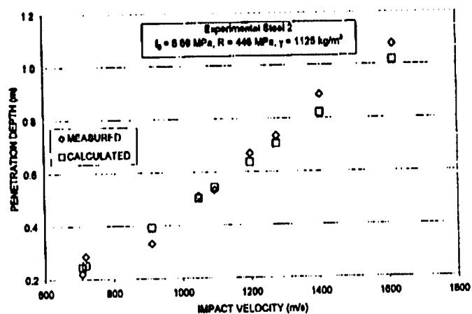
Figure 5. Plot of penetration depth versus impact velocity for experimental steel_2.
