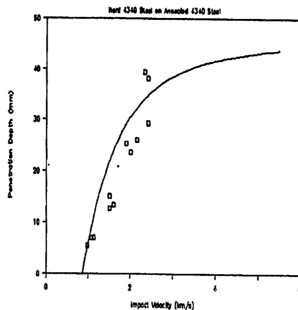
Figure 17b. Penetration Depth (mm) vs Impact Vel.(km/s)
