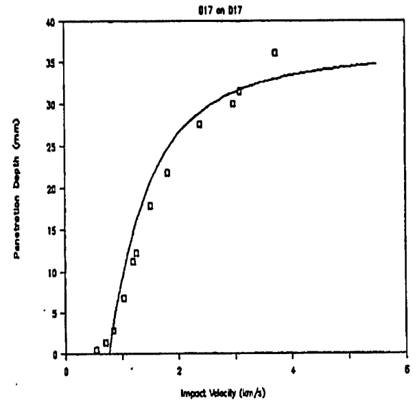
Figure 20b. Penetration Depth (mm) vs Impact Vel.(km/s)
