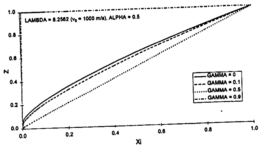
Figure 4. Plots of optimal nose shape for \alpha = 0.5 and \lambda = 8.2562 ( v_0 = 1000 m/s) for various values of friction coefficient \gamma .
