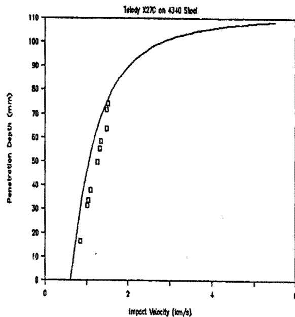
Figure 18b. Penetration Depth (mm) vs Impact Vel.(km/s)
