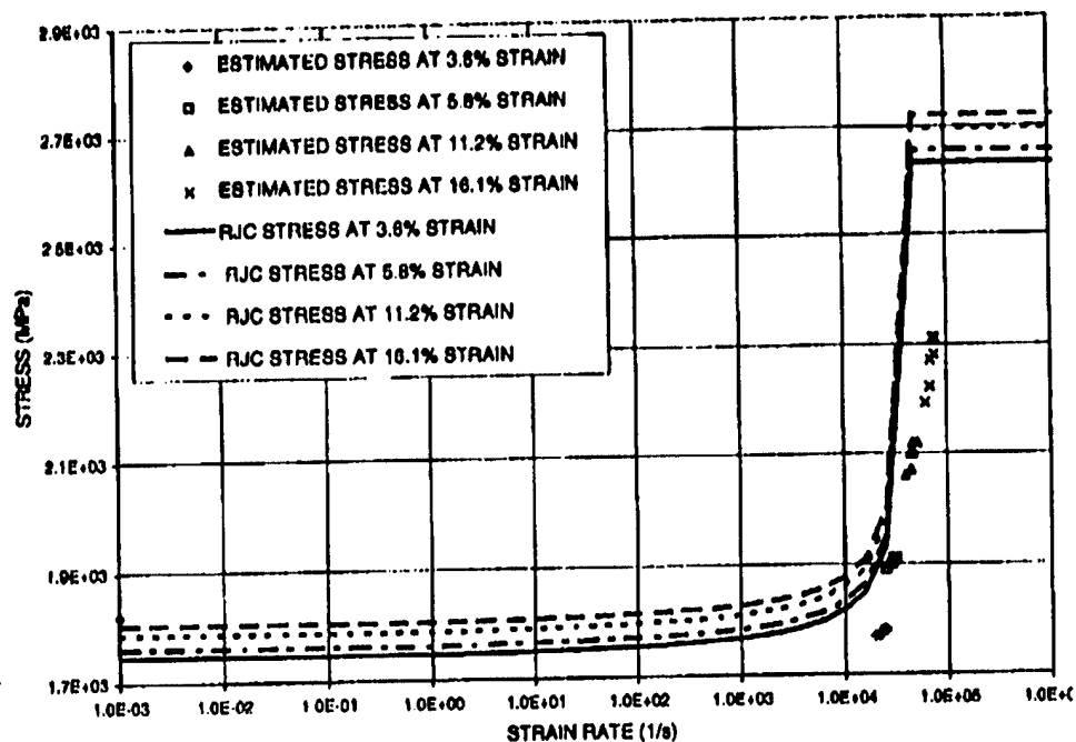
Fig. 7. Plots of yield strength versus strain rate for Astralloy-VH steel for various strain levels comparing RJC strength model results (Eqns (3) and (4)) with quasi-static measurements and estimates from a one-dimensional Taylor specimen model.
