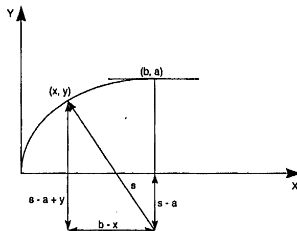
Fig. 2. The ogival nose geometry. The tip passes through zero at x = 0 and the tangent is zero at x = b . The remainder of the projectile is a cylinder of length L
