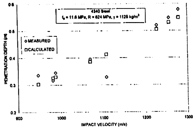
Figure 10. Plot of penetration depth versus impact velocity for 4340 steel.
