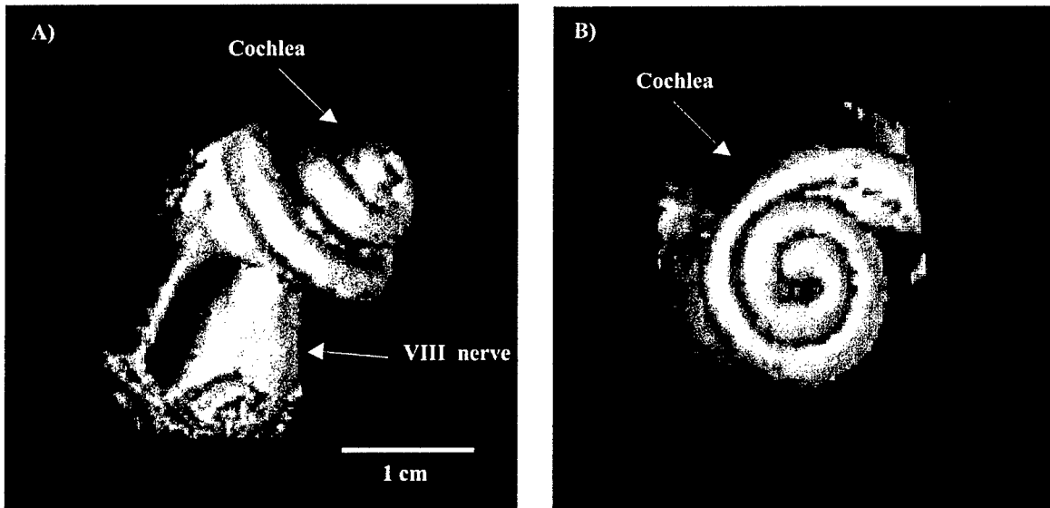
Figure 5.2. 3-D reconstruction of the cochlea from specimen EG 6 A) lateral view showing the height of the right whale cochlea spiral and the VIIIth nerve B) View of the cochlear spiral illustrating the number of turns in the right whale cochlea.
