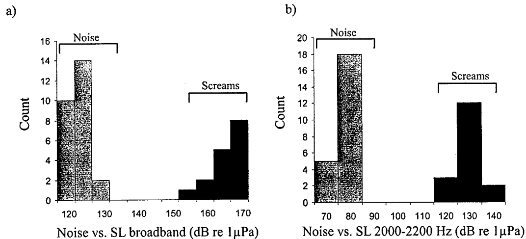
Figure 3.23. Plot showing the measured noise levels and the calculated source levels for the right whale Scream both broadband and in the 2000-2200 Hz band. These values were used to roughly estimate the range that right whales may be able to detect these signals.
