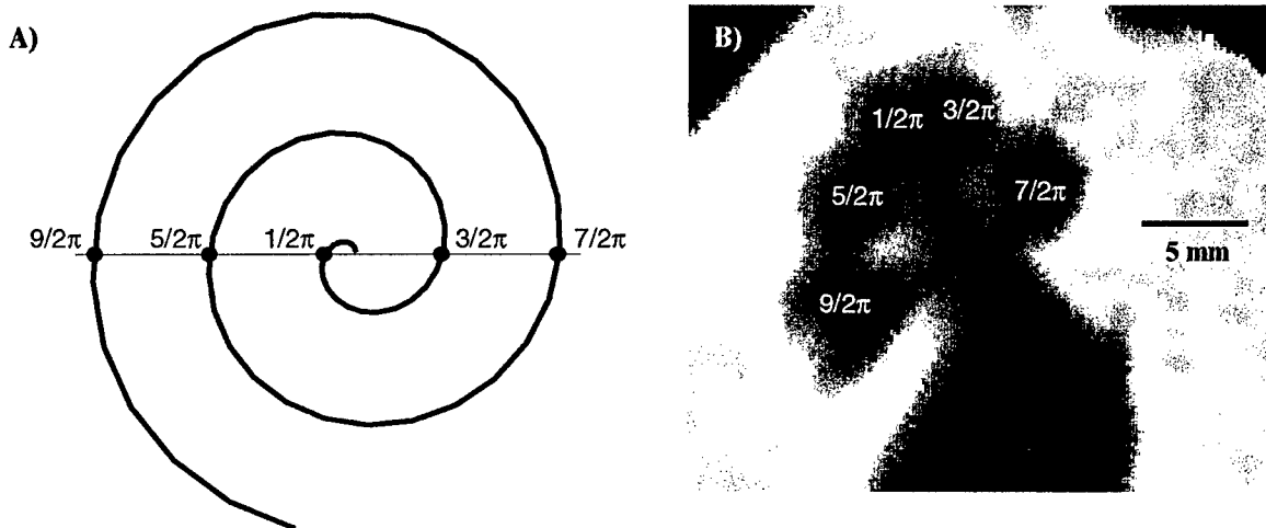
Figure 5.4. Cross section through a right whale cochlea for CT measurements. A) Schematic showing the orientation of the cross section B) An example of the resulting 2D CT image from the cross section.
