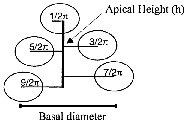
Figure 5.5. Illustration of the measurements made from 2D CT cross sections from right whale specimens with 2.5 turns.
