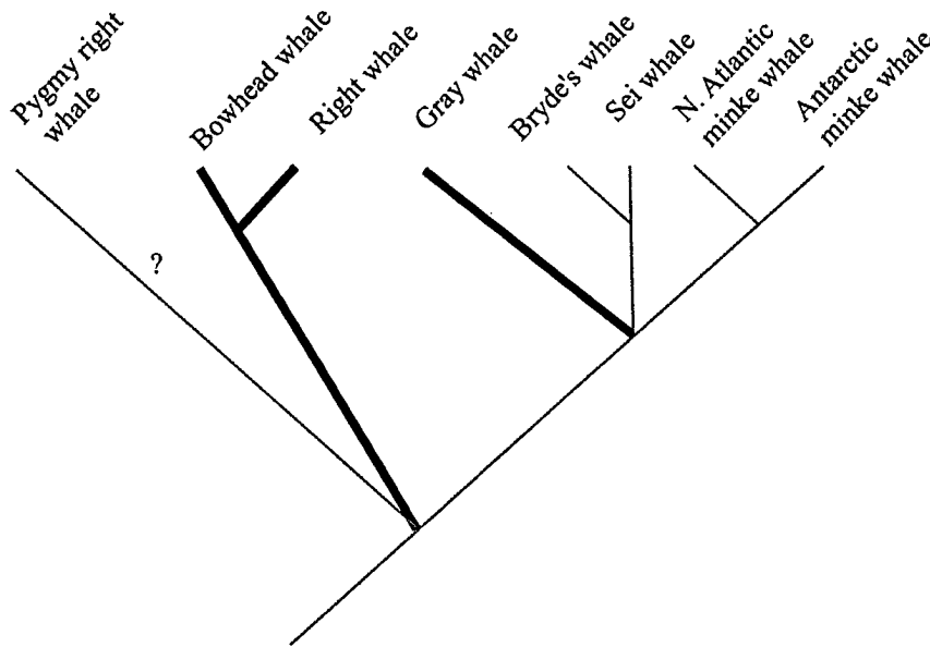
Figure 6.1. Relationship among mysticete species based on total evidence molecular data (Hasegawa et al., 1997). The darker branches indicate species with documented observations of SAG-like behaviors.
