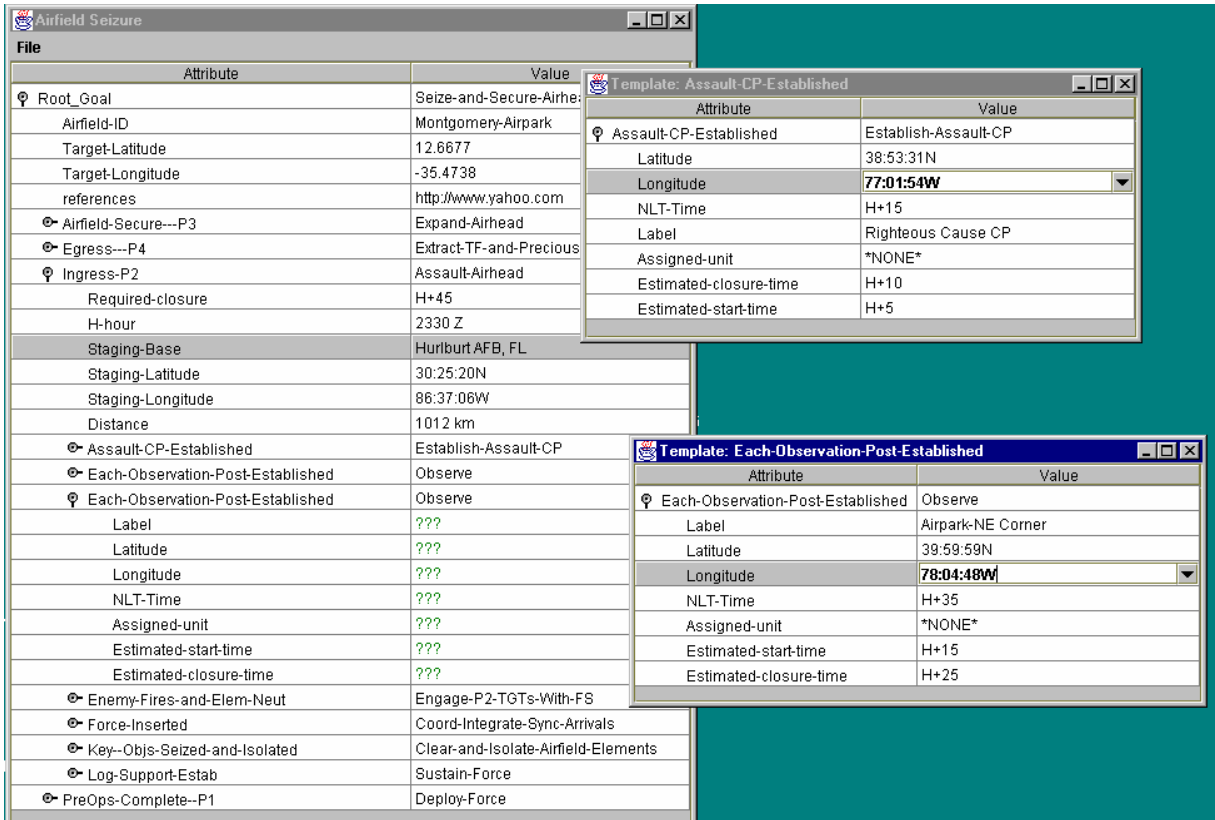
Figure A-7 Spreadsheet Interface
