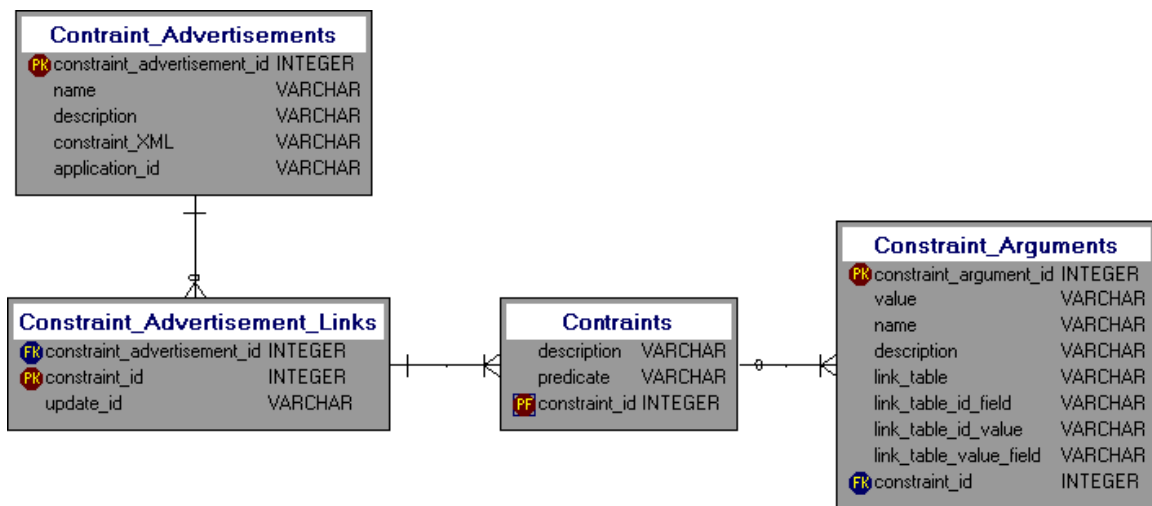
Figure 6 - Constraint Tables w/o links to rest of SDM
