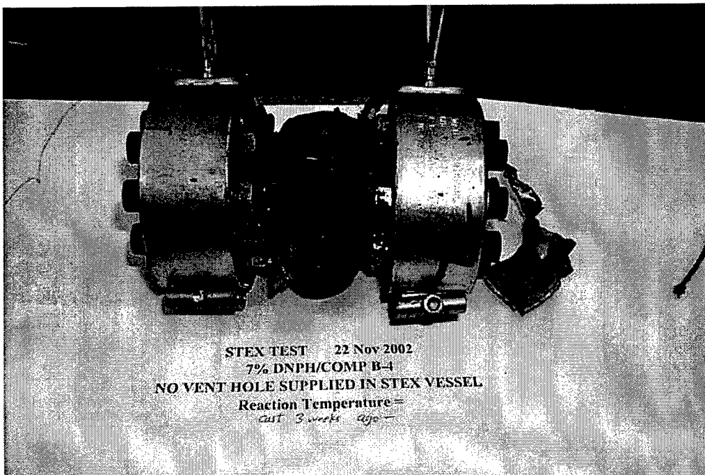
Figure 6 STEX test mild result using 7% DNPB with Comp B and no venting
