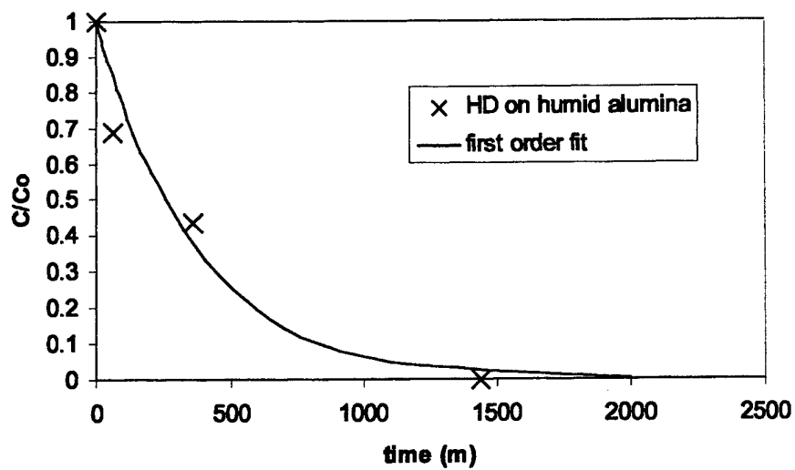
Figure 18. Reaction Rate Behavior of HD on Humid Alumina Demonstrating First Order Behavior.
