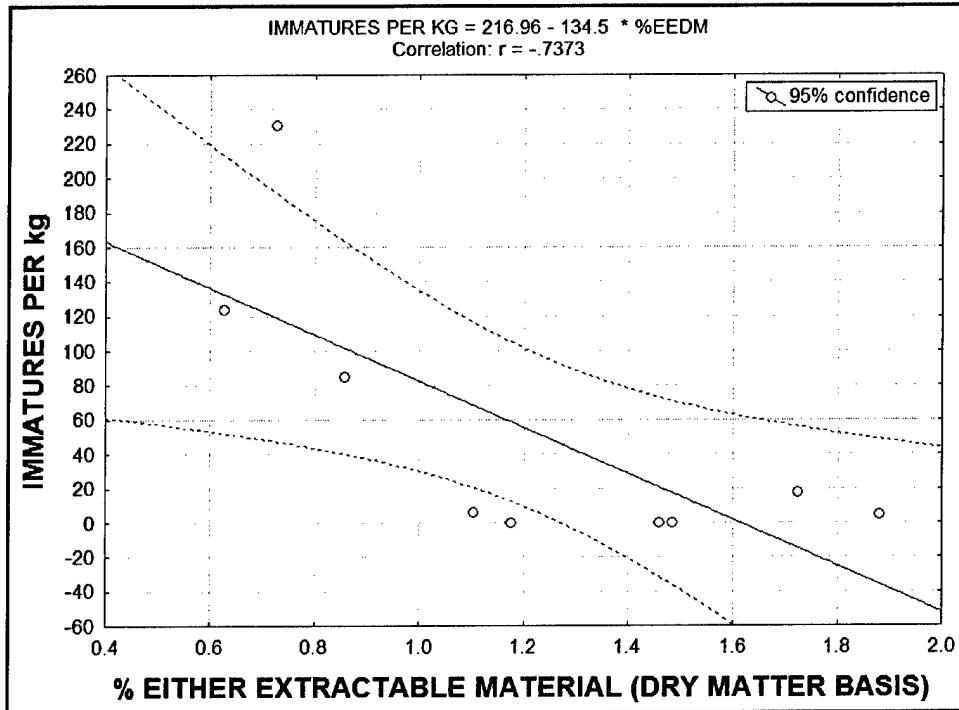
Figure 13. Relationship between mean immatures per kg and ether extractable compounds for sites on Lake Seminole during 2000 ( p < 0.05 , n = 9 , r = -0.7373 )
