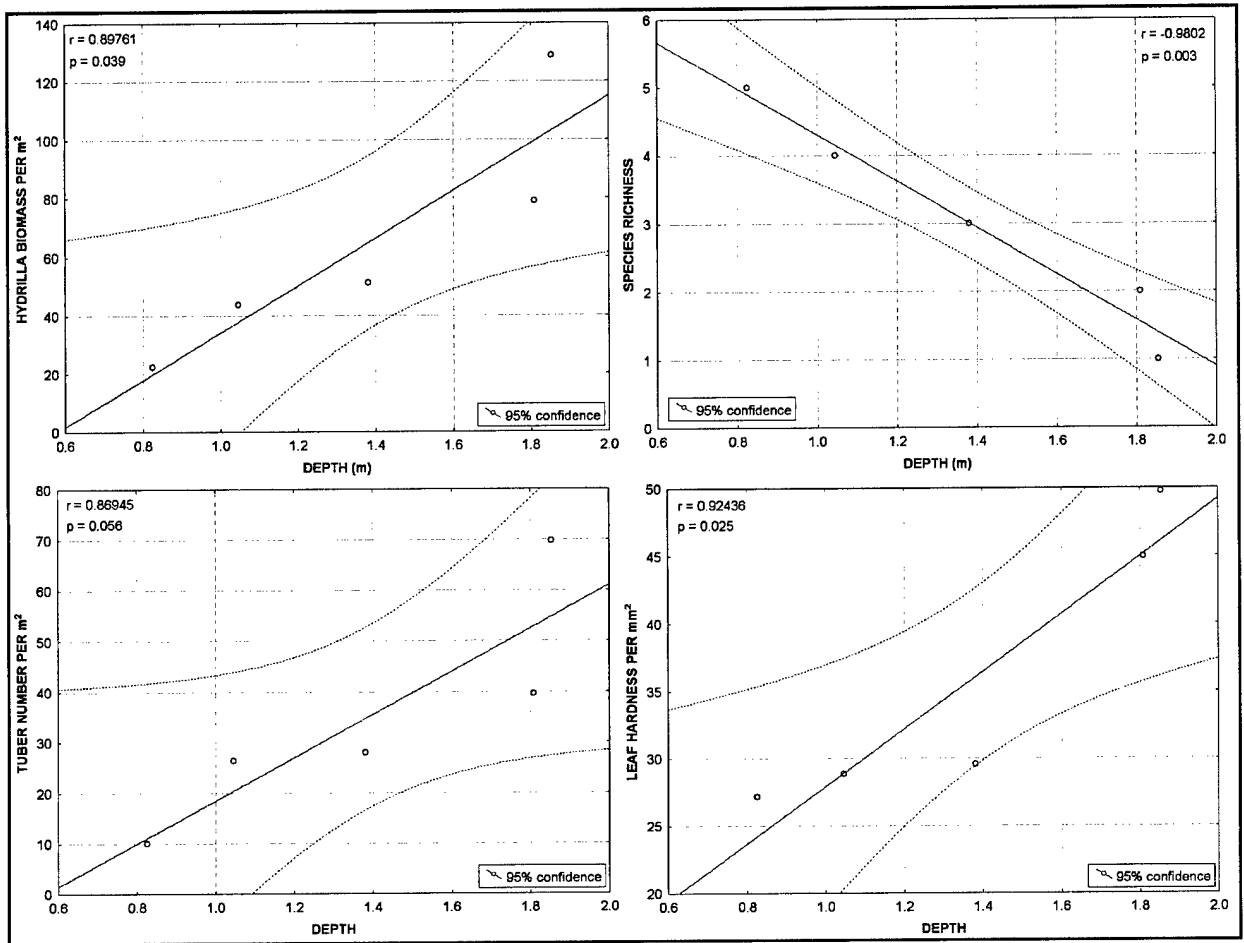
Figure 17. Correlations between depth and hydrilla biomass, species richness, tuber number per m 2 , and leaf hardness for means calculated on a species richness basis. All correlations are significant at the p < 0.05 except for tuber number which is significant at p = 0.056 level and n = 5 . The r -values and actual p -values are printed on each graph
