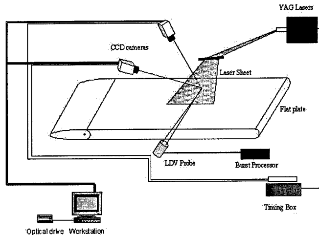
Schematic of DPIV setup
