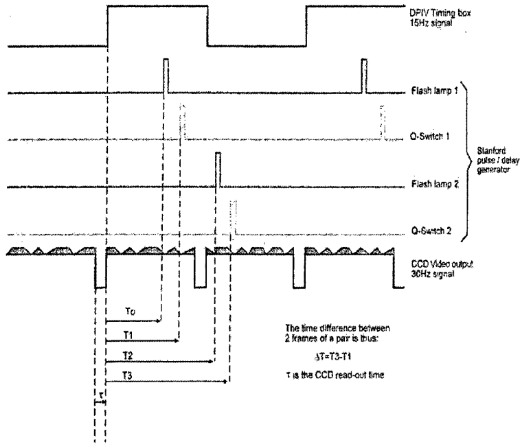
Figure 4: Timing Diagram
