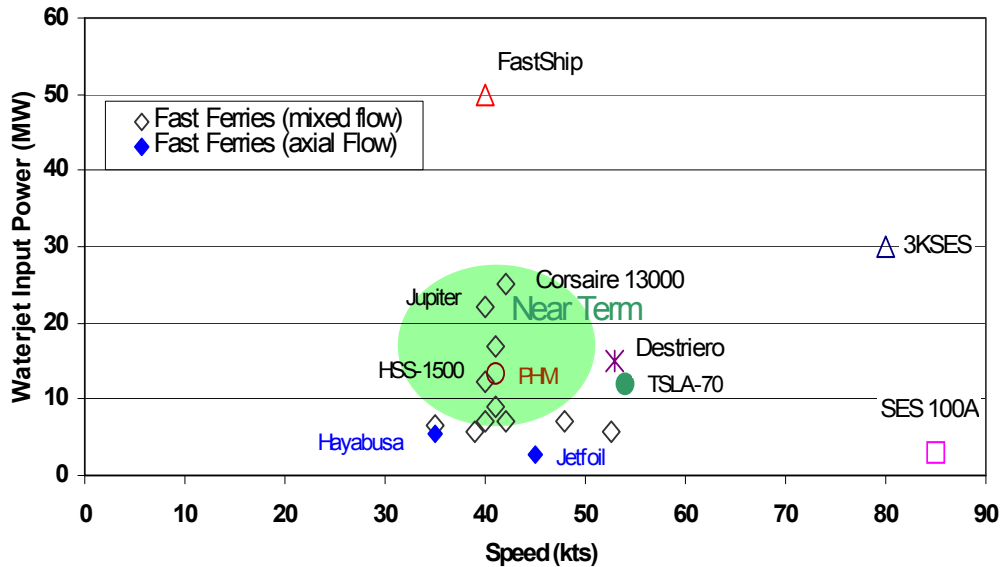
Figure 5.3.2-2: Waterjet Technology
