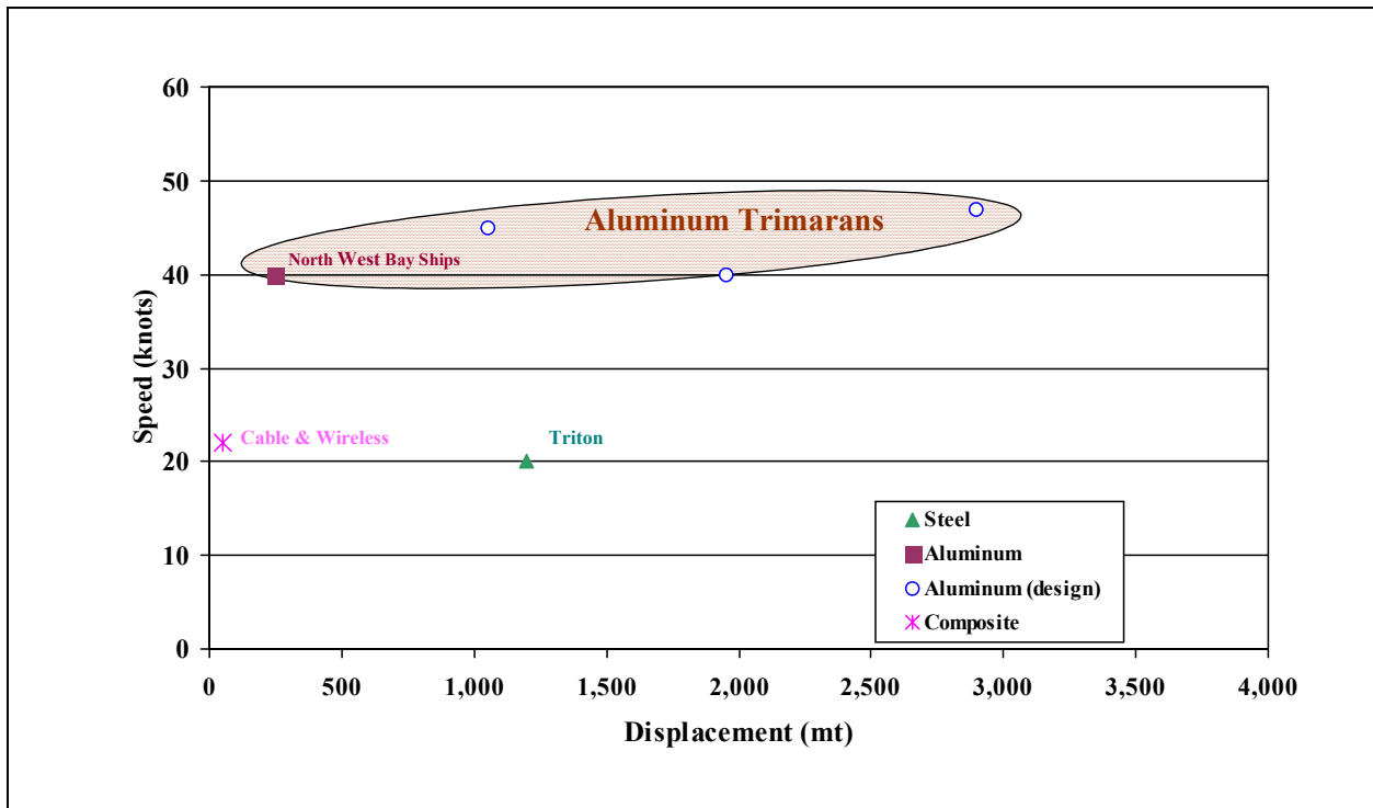
Figure 2.4.1-4: Trimaran Technology
