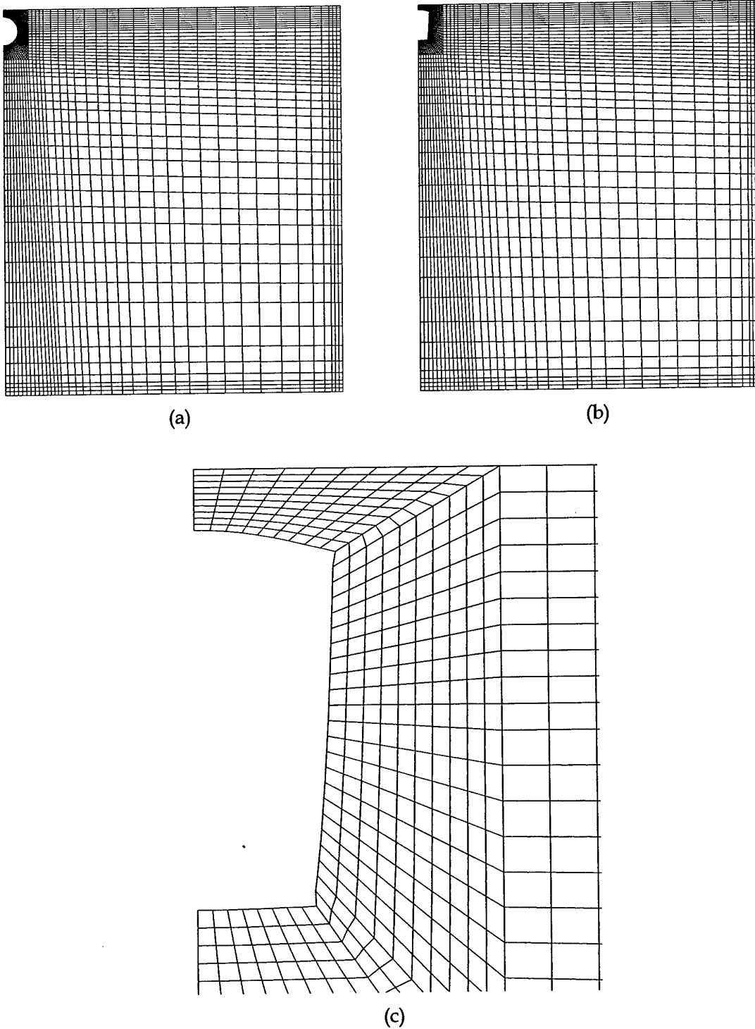
Fig. 13. Finite element mesh for 1/4 -symmetry model of large rectangular plate containing two closely-spaced holes for mixed biaxial field remote loading S_1 = -1/2S_2 . (a) Initial circular hole with e/h = 0.5 . (b) Optimal hole with e/h = 0.3224 . (c) Close-up view of mesh for optimal hole.
