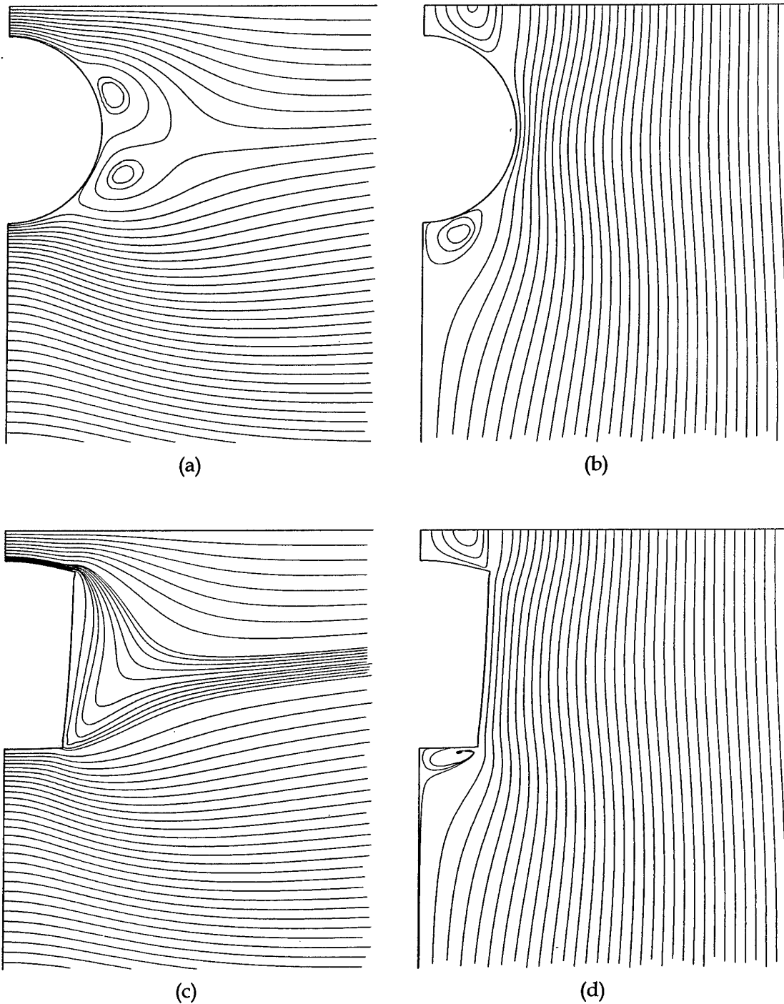
Fig. 18. Loadpaths for 1/4 -symmetry models of two interacting non-optimal circular holes and optimal holes in a large plate for mixed biaxial field remote loading S_1 = -1/2 S_2 and e/h = 0.3224 . (a) x-direction loadpaths and (b) y-direction loadpaths for the circular hole. (c) x-direction loadpaths and (d) y-direction loadpaths for the optimal hole.
