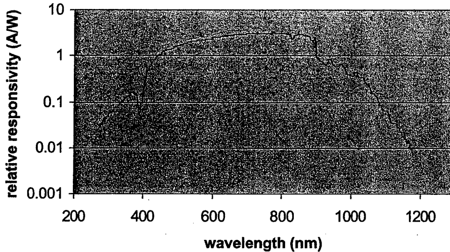
Figure 8. Spectral response of a p-GaN/GaN:Er/n-Si (pin) sample on silicon.
