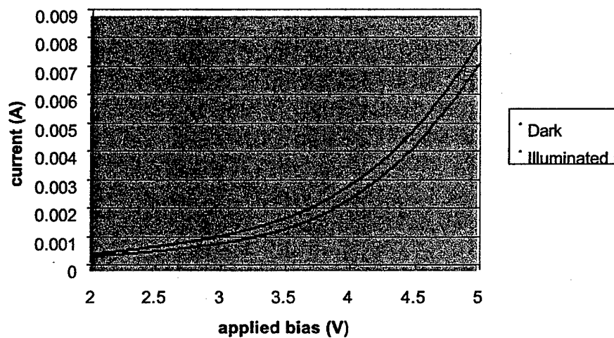
Figure 7. (a) I-V curves measured from one of the processed GaN:Er samples showing effect of response under illumination. (b) The same I-V curves showing more clearly the diode action of the GaN:Er diode to light.
