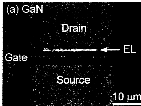
Fig. 18. EL distributions in (a) Ga N HEMT at V_{DS} = 70V and V_{GS} = -2V . (Takeshi NAKAO, Yutaka OHNO, Mitsutoshi AKITA, Shigeru KISHIMOTO, Koichi MAEZAWA, Takashi MIZUTANI, "Electroluminescence in AlGa N /Ga N High Electron Mobility Transistors under High Bias Voltage", Jpn. J. Appl. Phys. Vol. 41 (2002) pp. 1990–1991)
